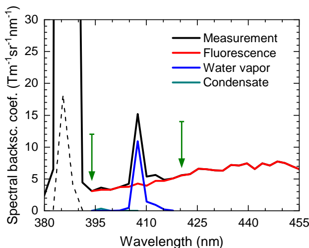
Figure 7. Decomposition of spectra obtained with the UVA spectrometer as exemplified by the RAMSES measurement at 4.3 km on 9 August 2021, 22:58 UTC. Center wavelengths of spectrometer detection channels that are unaffected by Raman scattering from molecular nitrogen, water vapor and condensate (liquid water, ice) are indicated (green arrows). The measurement is multiplied by a factor of 0.03 to fit into the display range around the vibrational-rotational Raman band of N_2 (dashed curve).
