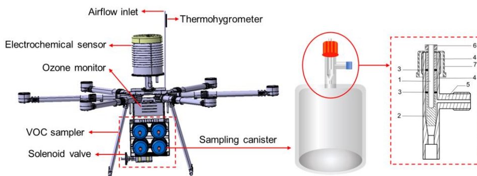
Figure 1. Left: the UAV sampling system. Right: schematic diagram of designed quartz sampling canister (1: stainless-steel column with internal thread; 2: polytetrafluoroethylene column; 3: rubber O-ring; 4: glass valve with inner inclined cone; 5: air inlet channel; 6: stop-screw nut; 7: screwable part).
