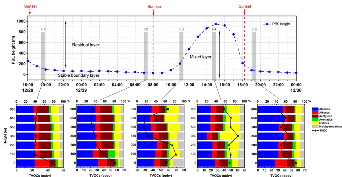
330 Figure 6. Evolution of VOC vertical profiles with PBL development in five flights during 28–29 December (the grey area in the top panel is the time and height covered by each flight).
