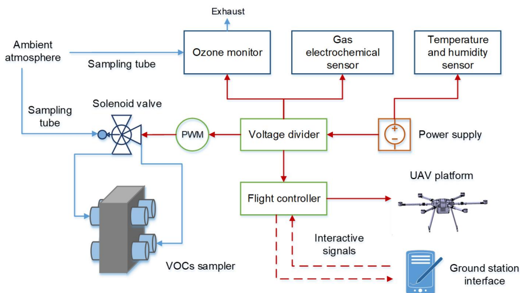
155 Figure 2. Schematic diagram of integrated sampling device (the blue and red lines represent air flow and electronic connections, respectively).
