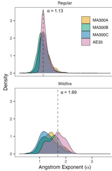
Figure S9: Distribution of Ångström Exponent ( \alpha ) from the four aethalometers during regular (top) and wildfire (bottom) period. The \alpha values have been calculated from hourly estimates of UV and IR b_{\text{abs}} values. Vertical dashed line represents the peak of the distributions from AE33 measurements for individual period.
