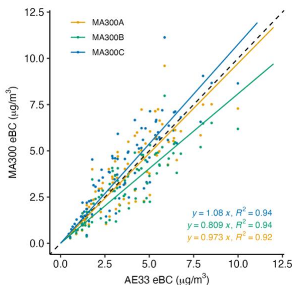
Figure S 14: Scatter plot of eBC mass concentration for individual MA300 units A,B and C vs AE33 during the high PM event.. The dashed line represents the 1:1 line, and solid colors are the regression fit lines for the individual MA300 units
