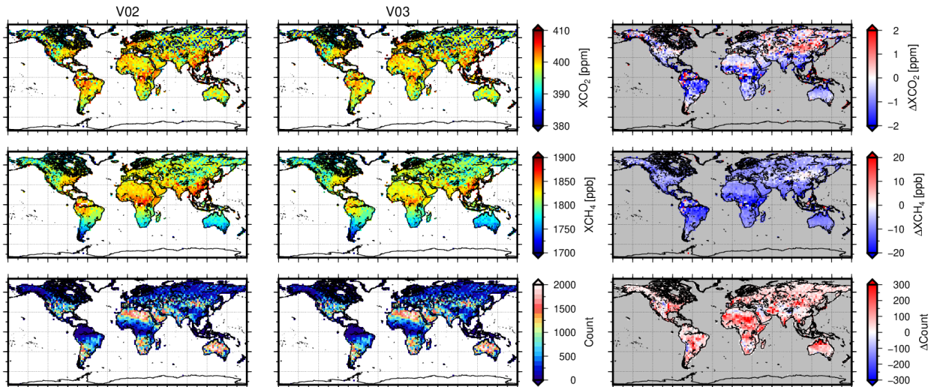
Fig. 5: Global distributions of XCO 2 (top), XCH 4 (middle), and the number of observations (bottom) for V02.90/91 (left), V03.00 (middle), and their differences (right) from the launch to 2021 over land and mixed surface. The values are averaged or integrated within 2.5°×2.5° grid boxes. All the observations were used for each version.
