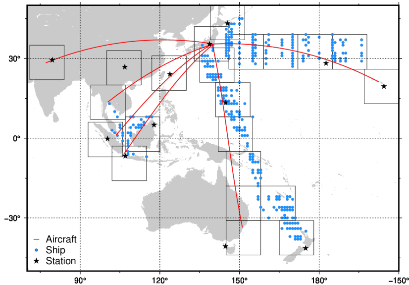
Fig. 12: Main route or locations of the aircraft (red line), ship (blue dot), and station (black star) measurements. The areas for comparison with the GOSAT data are shown in boxes. Here, we only show the main routes of the aircraft measurements (Haneda/Narita to Delhi, Bangkok, Singapore, Jakarta, Sydney, and Honolulu) accounting for more than 97% although the remaining data contain the other routes (Haneda/Narita to Taipei, Kuala Lumpur, Denpasar, Cairns, Brisbane, and Guam).
