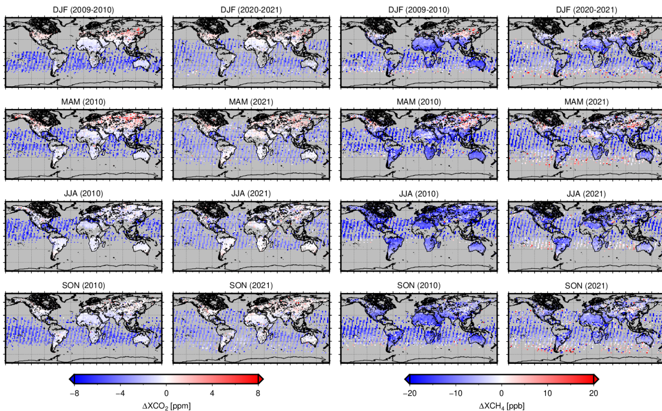
770 Fig. 8 Global distributions of the differences in seasonal mean XCO_2 (left eight panels) and XCH_4 (right eight panels) in 2010 and 2021. The grid size is same as Fig. 5. All the observations were used for each version.
