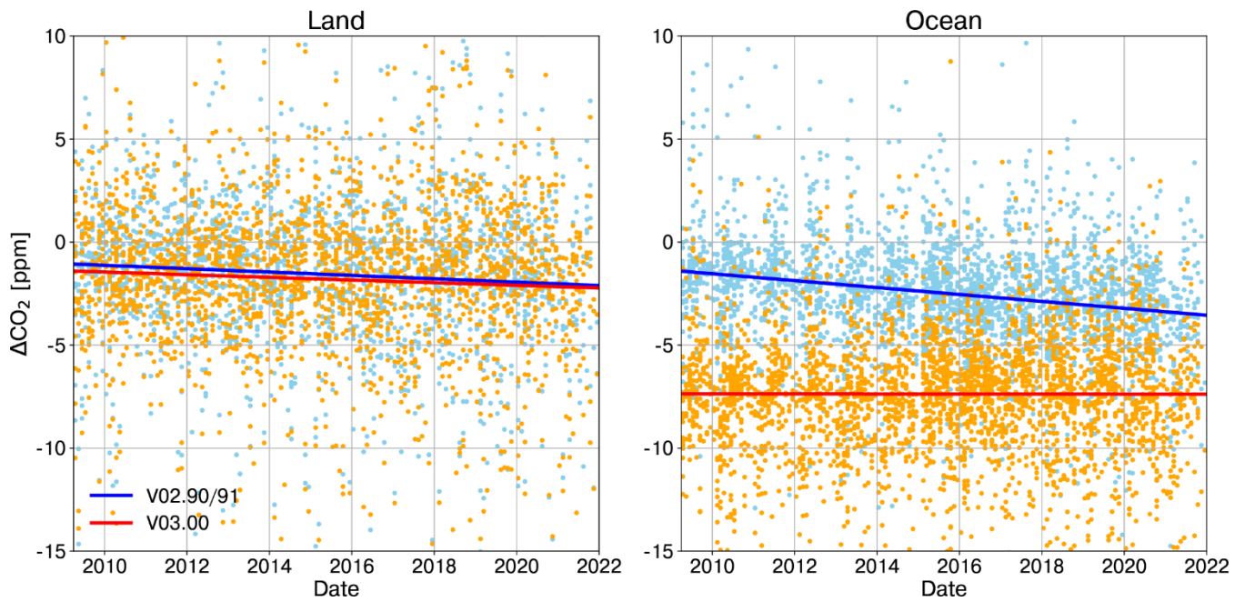
805 Fig. 13: Time series of the differences between the GOSAT products and in situ measurements (GOSAT minus in situ measurements) over land (left panels) and the ocean (right panels). The regression lines are plotted as red and blue lines.
