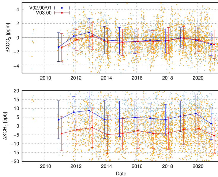
Fig. 11: Annual mean differences of the GOSAT L2 product and TCCON GGG2020 in the match-up condition of \pm 0.1^\circ for XCO 2 (top) and XCH 4 (bottom). The red and blue lines indicate V03.00 and V02.90/91, respectively. The annual mean plots are slightly shifted between V02 and V03 for visibility. Each individual observation from V03.00 and V02.90/91 is plotted as orange and light-blue dots.
