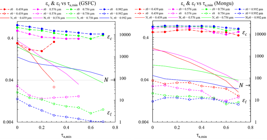
Figure 9: GSFC and Mongu variations of regression-derived values of \epsilon_c and \epsilon_f as a function of a minimum value of total AOD at 500 nm ( \tau_{a,min} ) employed in the \eta' vs \eta regressions 11 (to be clear, the regressions of Figure 6 and the regression-derived \epsilon_c and \epsilon_f values of Figure 7 were obtained with no restrictions on the matched AERinv and SDA retrievals). Same colour scheme as Figure 6 and 7. The number of matched retrievals ( N ) are also shown (right-hand axis). Result are not shown in cases where N < 20 . The orange filled large circle represents the only \epsilon_f point of the r_0 = 0.439 \mu\text{m} regressions that survived the N < 20 criterion and that did not yield a negative \epsilon_f value.
