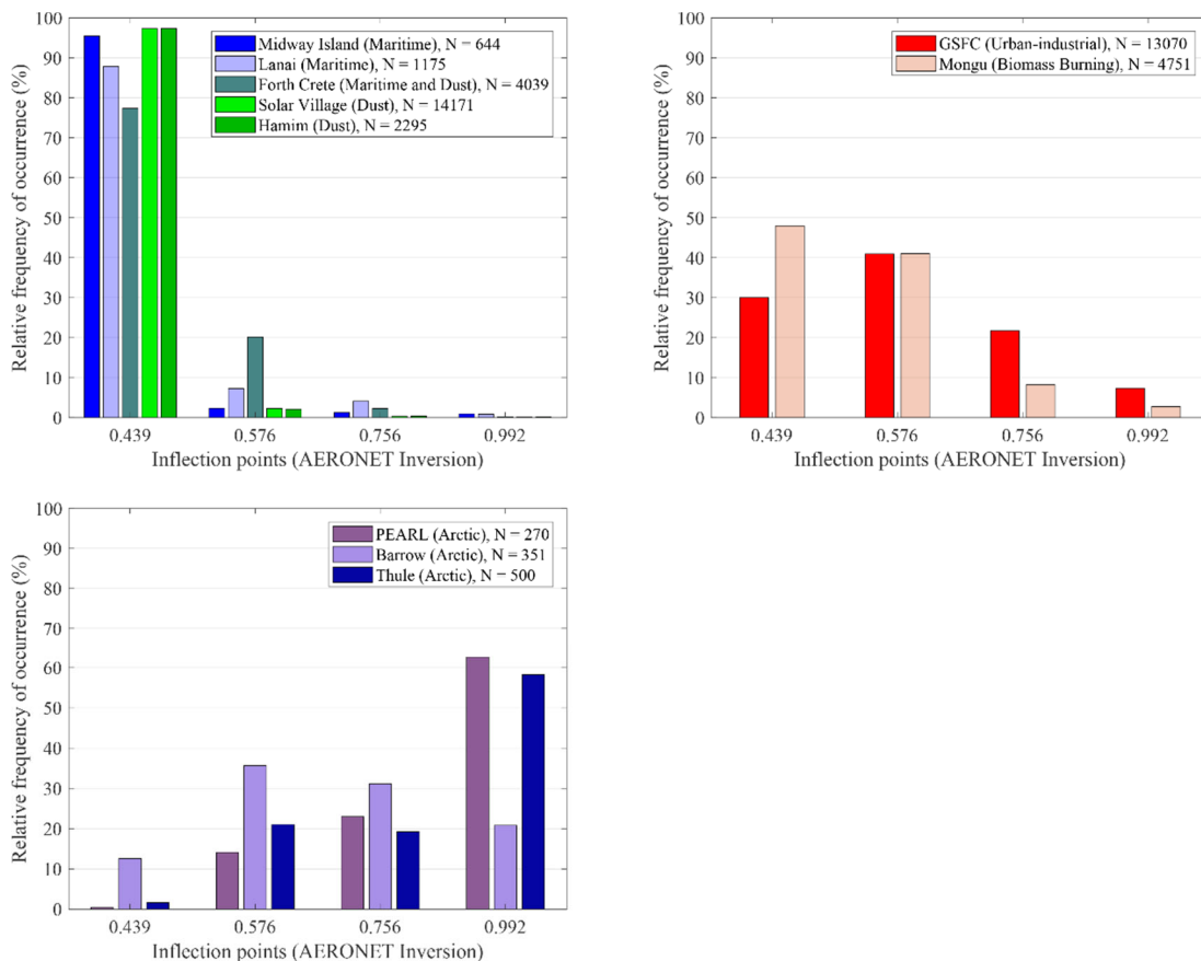
Figure 5: Relative frequency occurrence (FO) distributions for the four different AERONET inflection points ( r_0 values) for all Table 1 AERONET sites.
