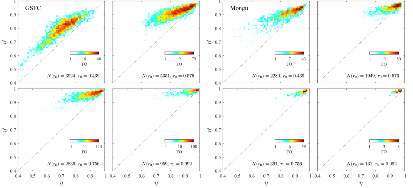
Figure A2: \eta' vs \eta FO distributions for GSFC and Mongu. See the caption of Figure S1 for details. \eta' vs \eta FO distributions for GSFC and Mongu.
