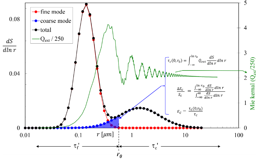
120 Figure 1: Illustrative, fine and coarse mode (red and blue) lognormal particle-surface size distributions ( dS/d \ln r ) and the Mie kernel (extinction efficiency Q_{ext} ) for a wavelength of 0.5 \mu\text{m} and a refractive index of 1.44 - 0.0035i (by particle surface we mean the projected particle surface area of \pi r^2 ). The cutoff radius 7 ( r_0 ) applies to a SMF type of computation. The total dS/d \ln r (black curve) is (in order to have a level of grounding in reality) the sum of the FM and CM lognormal dS/d \ln r curves that were individually manipulated to fit the mean of a series of AERONET and ground-based ( dV/d \ln r ) FM and CM sea-salt curves reported in Figure 8f of Reid et al. (2006). We 125 base this illustration on dS/d \ln r because it is more optically fundamental than the AERInv particle-volume PSD (the projected particle surface area is employed to normalize the extinction cross section to obtain the fundamental extinction efficiency). An analogous explanation (and a graph similar to that of Figure 2) would apply to the particle-volume PSD.
