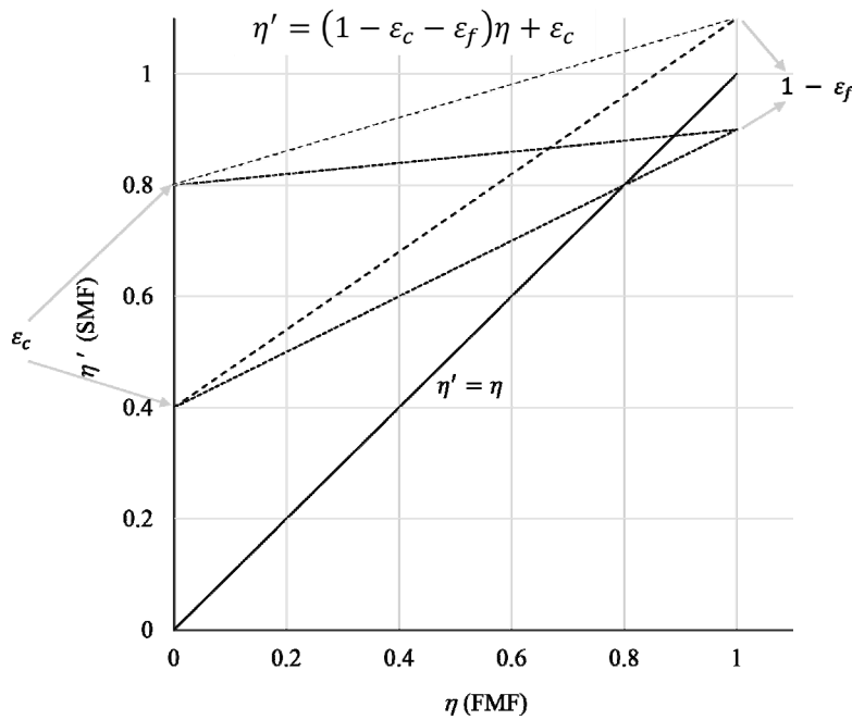
195 Figure 3: \eta' (SMF) vs \eta (FMF) lines of equation (7a) for three \varepsilon_c values and three \varepsilon_f values (0, 0.4, 0.8 and -0.1, 0 and 0.1 respectively). The \varepsilon_f values were inspired by the range of empirical values seen in Figure 6 (and, in the case of \varepsilon_f by the range of values, whether real or artefactual, seen in Figure 7).
