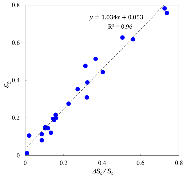
190 Figure 2: Plot of \varepsilon_c vs \Delta S_c/S_c for a variety of simulated optical depth retrievals. The lognormal FM and CM PSDs employed in these simulations were obtained by fitting their sum to retrieved AERinv PSDs over a variety of sites whose predominant aerosol type was urban, dust or marine (and employing the refractive indices provided by the retrieval product). The AERinv PSD retrievals were Version 2 (for which r_0 was fixed at 0.6 \mu\text{m} and, accordingly, for which the \varepsilon_c vs \Delta S_c/S_c regression would be only dependent on \varepsilon_c and 2 nd order parameters such as refractive index (i.e. independent of r_0 ).
