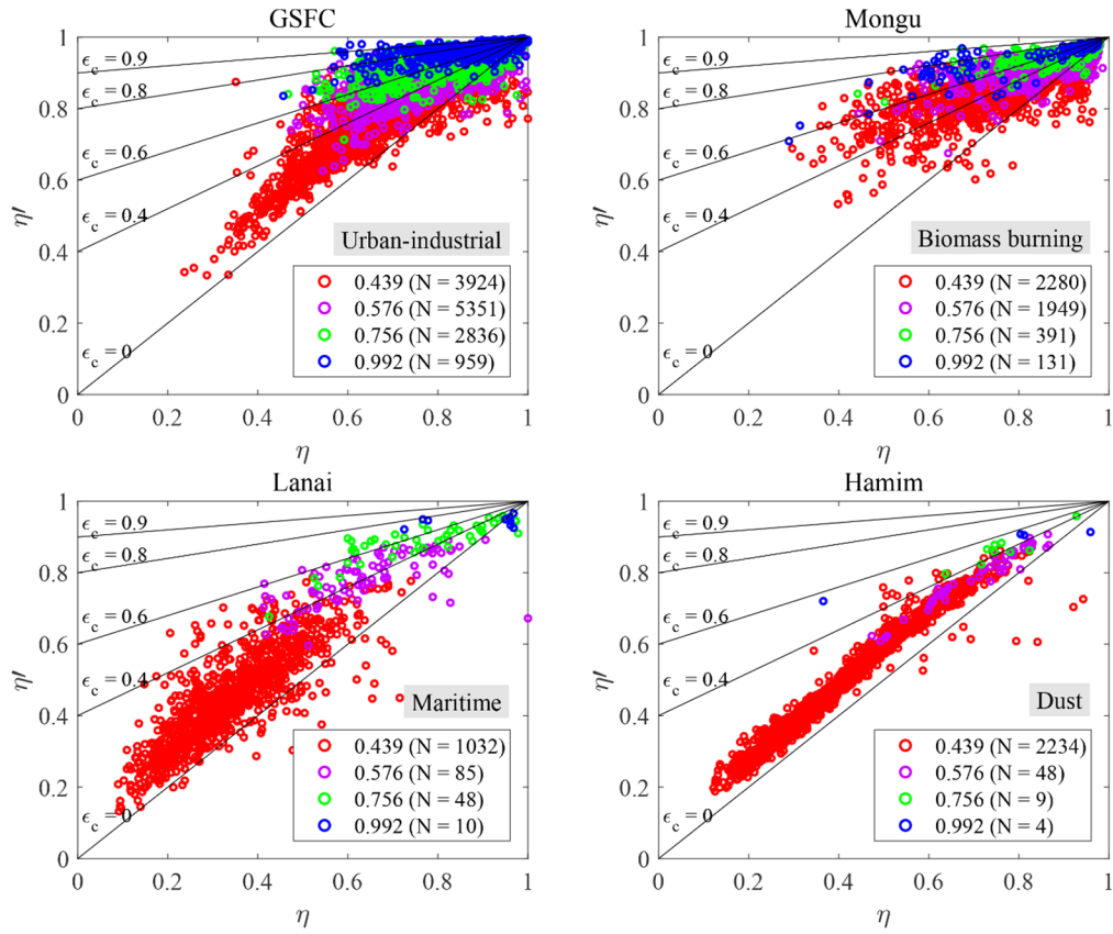
Figure 6: \eta' vs \eta (AERInv-derived SMF vs SDA-derived FMF) scattergrams for the sites of GSFC, Mongu, Lanai, and Hamim (respectively aerosol types of urban-industrial, biomass burning, marine and dust as per Table 1). The remaining scattergrams for the other sites are shown in Figure S1. The solid black lines are those of equation (7a) with (for the sake of the simplicity of the presentation coupled with the fact that \epsilon_f has a relatively minor role), \epsilon_f was set to 0.
