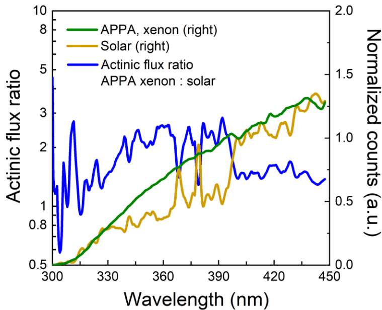
540 Figure 10. Spectral actinic fluxes inside the reactor when illuminated by the xenon lamp (green curve) and outdoors around noon on a sunny day in April (yellow curve), and the wavelength-dependent ratio of the two (blue curve). The approach used to calculate actinic flux from spectral irradiance measured with a spectrometer is described in the text.
