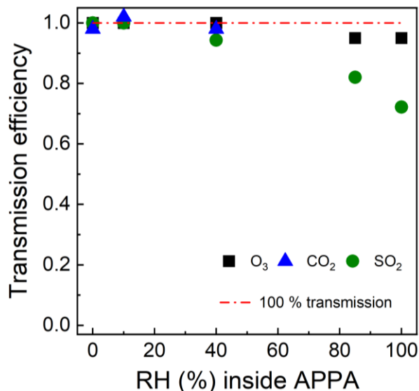
Figure 56. Gas transmission efficiencies of the APPA reactor as a function of relative humidity.
