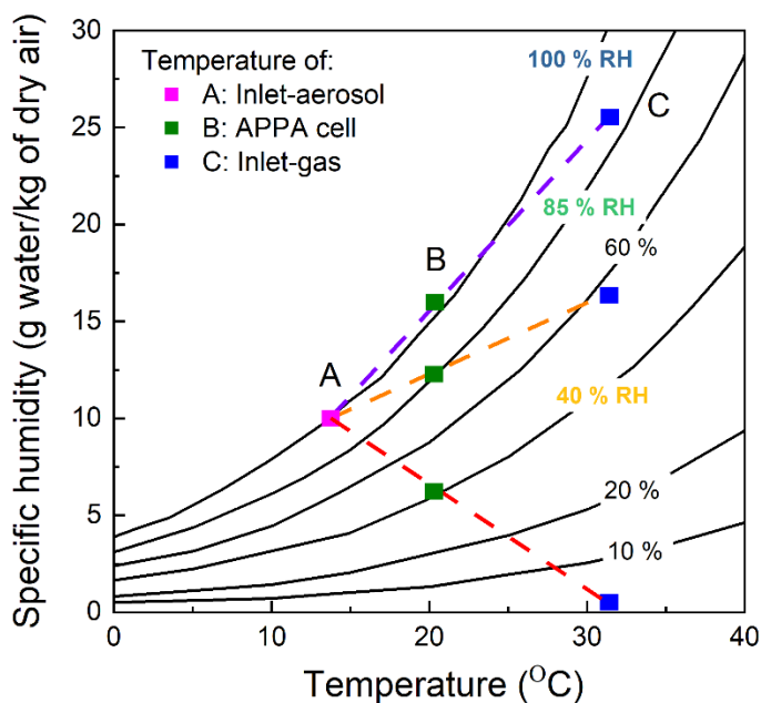
Figure 4. Relationship between the temperature and water vapor content of the two inlet flows and the resulting RH in the reactor.
