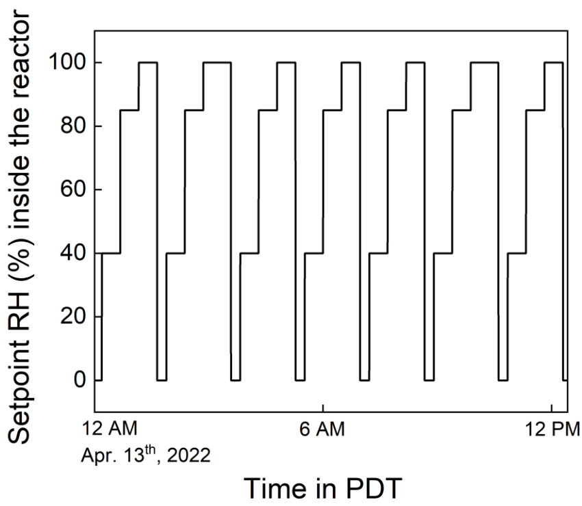
685 Figure 16. A typical RH cycle showing steps in the sequence of 40 %, 85 %, and 100 % RH. The short periods with very low RH follow the 100 % RH measurements and are designed to evaporate any residual liquid water from the walls before the start of the next 40 % RH measurement.
