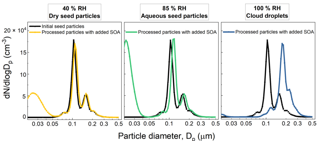
645 Figure 124. Example of a set of number size distributions of seed particles without and with added SOA formed from OH-oxidation of benzene for 40 % RH (left), 85 % RH (middle), and 100 % RH (right). The initial benzene mixing ratio was 90 ppb and the OH_{exp} estimated from KinSim is 3 \times 10^{11} molec. cm^{-3} s.
