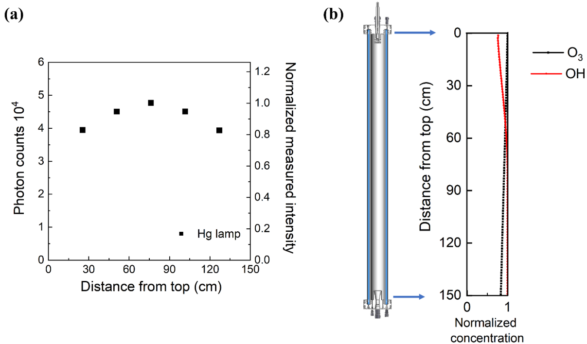
555 Figure 911. (a) Relative UV intensity profile and (b) normalized ratio of O 3 and OH concentration as a function of position in the reactor cell.
