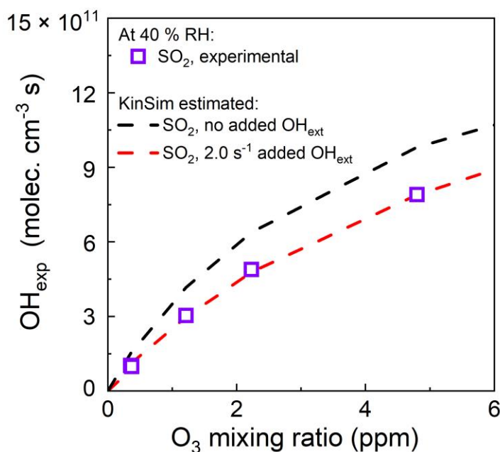
610 Figure 120. Variation of \text{OH}_{\text{exp}} estimated from \text{SO}_2 decay as a function of initial \text{O}_3 mixing ratio for 40 % RH.
