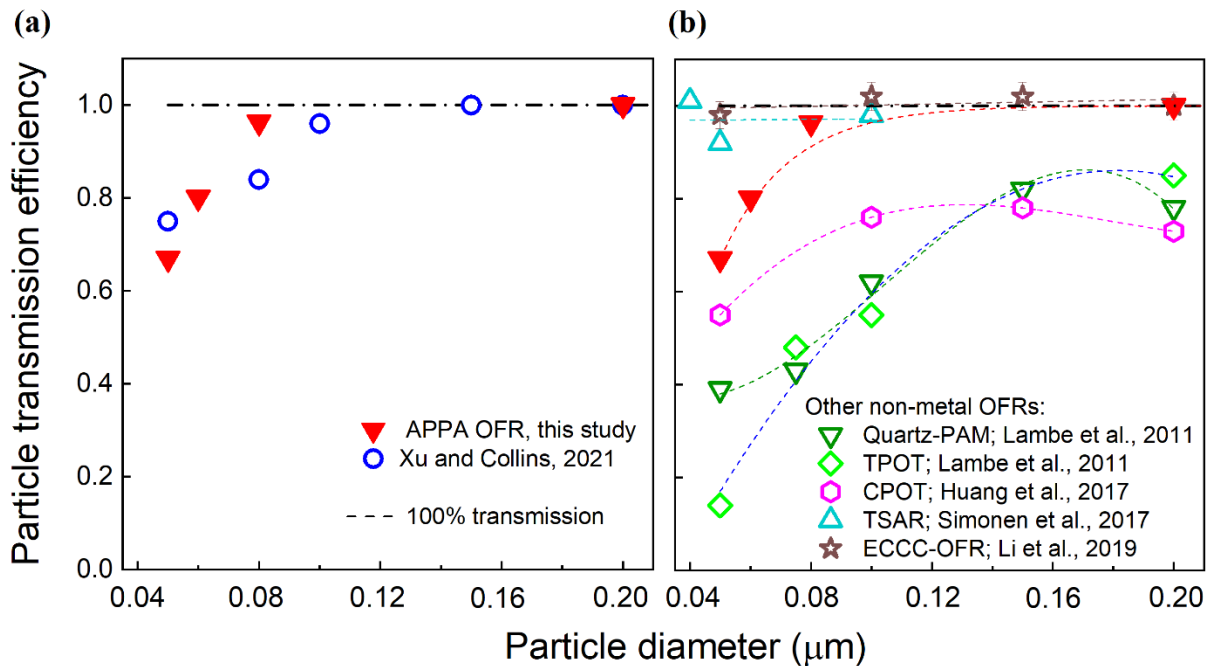
Figure 54. Particle transmission efficiency of the APPA reactor compared with those reported (a) for the OFR described by Xu and Collins (2021) and (b) for several non-metal OFRs reported in the literature, as described in the text.
