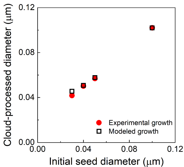
520 Figure 89. Measured diameters of cloud-processed and evaporated particles as a function of the diameter of the injected \text{K}_2\text{SO}_4 seed particles (red solid points), and the expected diameters calculated for the reactor conditions (3.3 \mu\text{m} droplet diameter, 50 ppb \text{SO}_2 , and 1.5 ppm \text{O}_3 ) and the set of relevant aqueous-phase reactions (black hollow squares).
