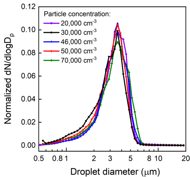
Figure 78. Droplet size distributions measured at the outlet of the APPA reactor for a range in concentration.
