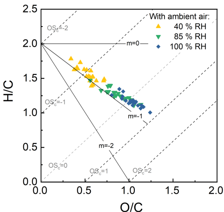
705 | Figure 147. O/C and H/C ratios determined from AMS measurements of SOA formed as ambient air was processed in the reactor. The significant decrease in H/C ratio and increase in O/C ratio with the progression from no liquid water in the reactor (40 %) to ALW (85 %) to cloud droplets (100 %) suggests oxidation in the aqueous phase was important.
