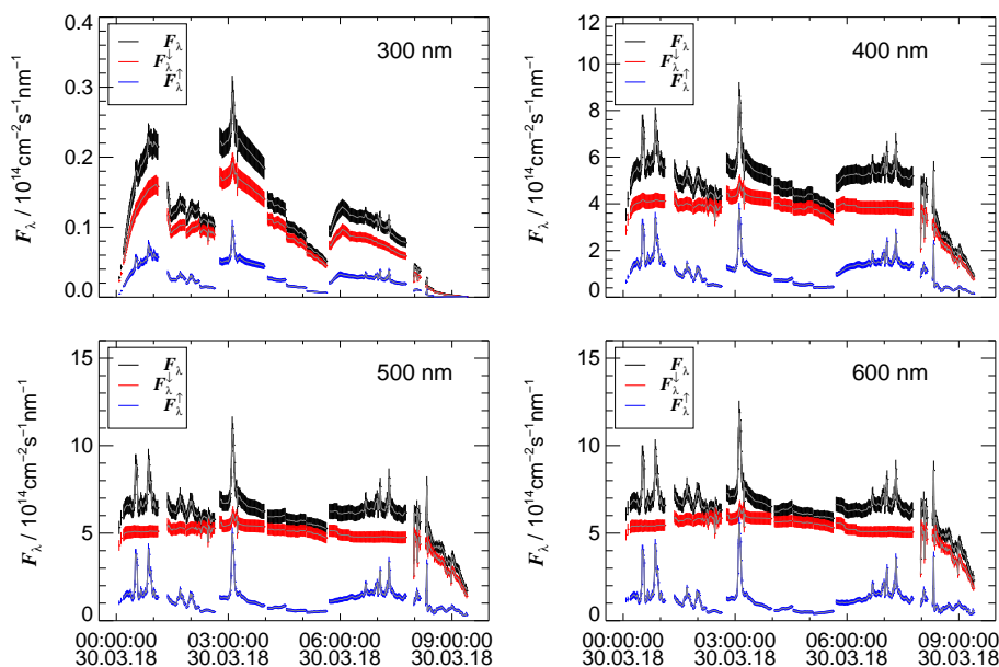
Figure 17. Total ( F_\lambda ), downward ( F_\lambda^\downarrow ) and upward ( F_\lambda^\uparrow ) spectral actinic flux densities of the HALO flight shown in Fig. 16 for the four selected wavelengths. The error bars correspond to total uncertainties including those from corrections and calibrations (Sect. S7, Supplement).
