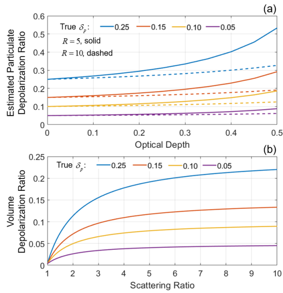
210 Figure 3. (a) Estimated particulate depolarization ratio as a function of optical depth for four values of the true particulate depolarization ratio in layers having unattenuated scattering ratios of 5 (solid lines) and 10 (dashed lines). (b) Volume depolarization ratio as a function of scattering ratio for four values of true particulate depolarization ratio.
