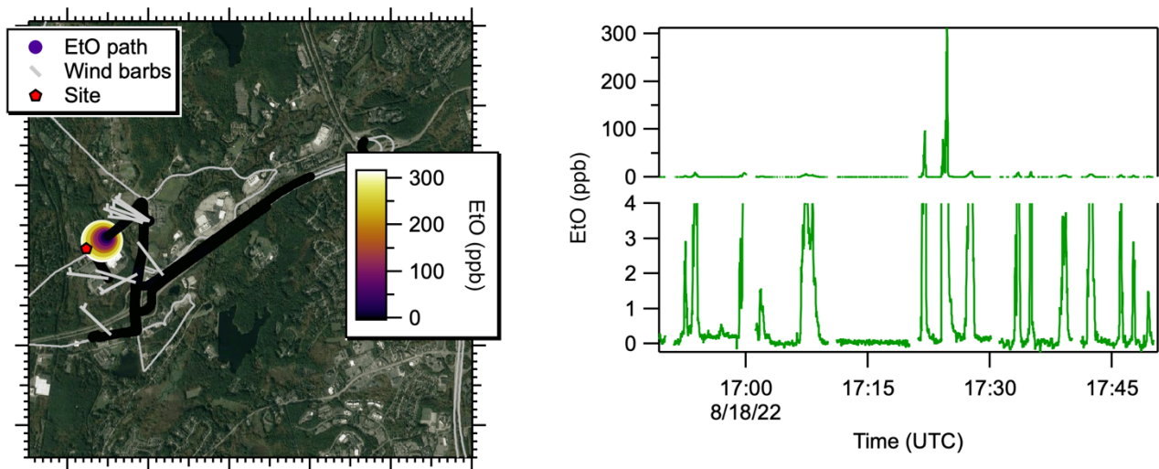
140 Figure S8. Afternoon Summary data downwind of Facility A. A map (left) shows AML path colored by EtO concentration, with wind barbs pointing into the wind. Time series show EtO concentrations zoomed to 0-4 ppb (bottom right) and at full scale (top right). Map underlay: Google, © 2022 CNES / Airbus, Landsat / Copernicus, MassGIS, Commonwealth of Massachusetts EOE, Maxar Technologies, USDA/FPAC/GEO
