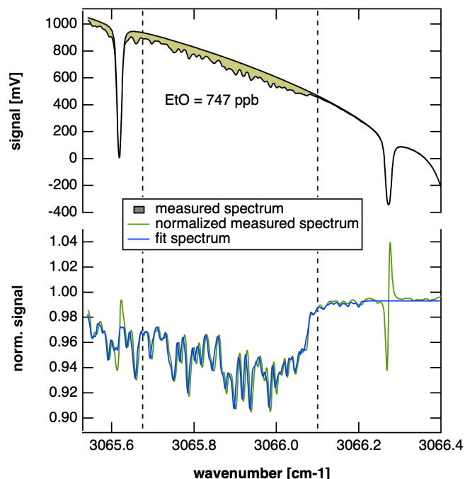
Figure S1. Summary spectrum for instantaneous Facility A measurement of 747 ppb. The top shows signal as a function of wavenumber, with EtO contributions highlighted in yellow. The bottom shows normalized measured (green) and fit (blue) spectrum.
