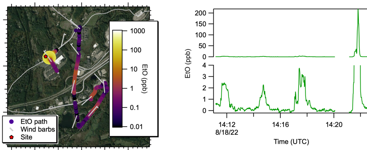
145 Figure S9. Detail of Morning Transect Downwind of Facility A. A map (left) shows AML path colored by EtO concentration (log scale), with wind barbs pointing into the wind. Time series show EtO concentrations zoomed to 0-4 ppb (bottom right) and at full scale (top right). Map underlay: Google, © 2022 CNES / Airbus, Landsat / Copernicus, MassGIS, Commonwealth of Massachusetts EOE, Maxar Technologies, USDA/FPAC/GEO
