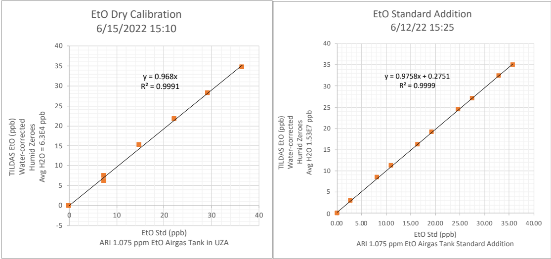
Figure S2. Example standard addition and dry dilution calibrations for EtO.
