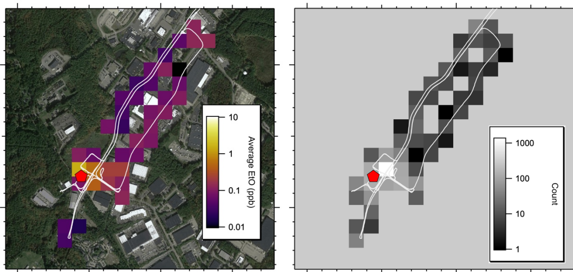
170 Figure S13. Binned average EtO concentrations downwind of Facility B (left) along with data point count (right). The facility is located at the red marker. Wind was from the West during these measurements. Map underlay: Google, © 2022 CNES / Airbus, MassGIS, Commonwealth of Massachusetts EOE, Maxar Technologies, RIGIS, USDA/FPAC/GEO
