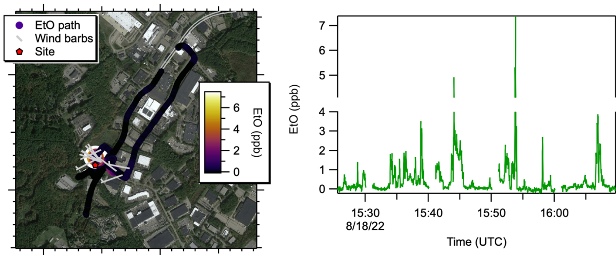
160 Figure S11. Full Summary time series downwind of Facility B. A map (left) shows AML path colored by EtO concentration, with wind barbs pointing into the wind. Time series show EtO concentrations zoomed to 0-4 ppb (bottom right) and at full scale (top right). Map underlay: Google, © 2022 CNES / Airbus, Landsat / Copernicus, MassGIS, Commonwealth of Massachusetts EOE, Maxar Technologies, RIGIS, USDA/FPAC/GEO
