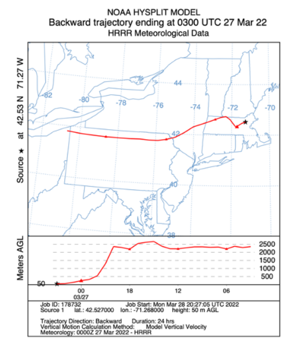
Figure S5. Back trajectory simulation for the EtO event on 3/27/2022. (NOAA Air Resources Laboratory)
