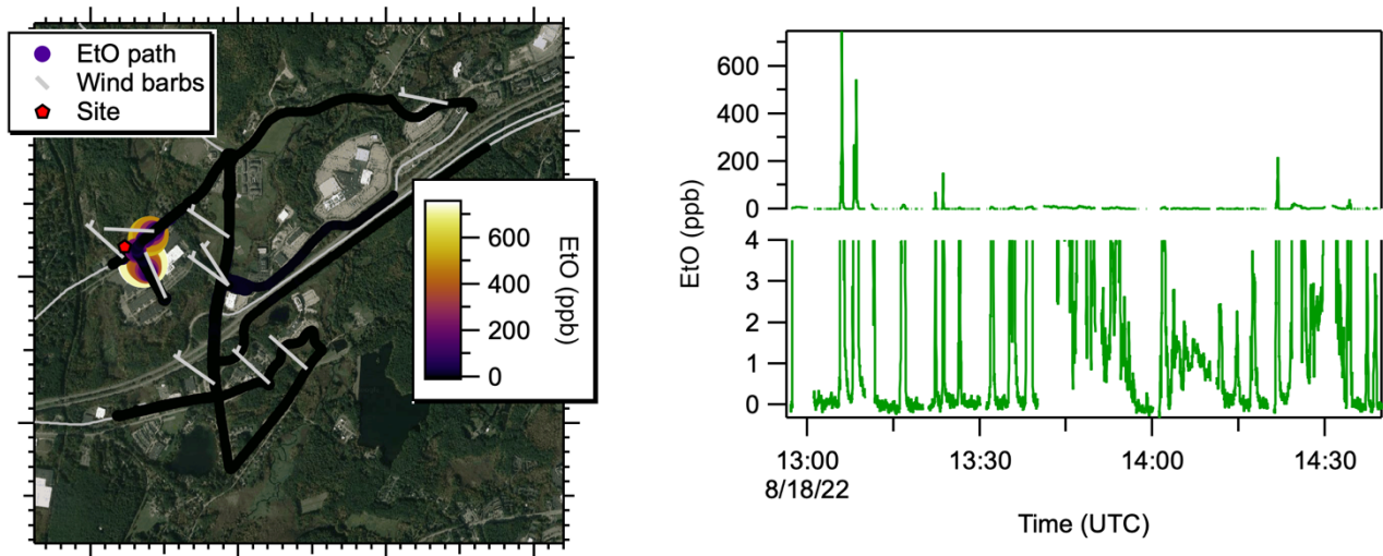
135 Figure S7. Morning summary data downwind of Facility A. A map (left) shows AML path colored by EtO concentration, with wind barbs pointing into the wind. Time series show EtO concentrations zoomed to 0-4 ppb (bottom right) and at full scale (top right). Map underlay: Google, © 2022 CNES / Airbus, Landsat / Copernicus, MassGIS, Commonwealth of Massachusetts EOE, Maxar Technologies, USDA/FPAC/GEO
