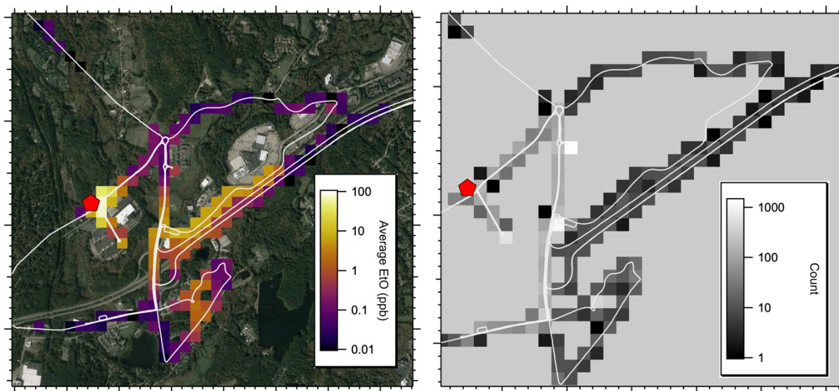
150 Figure S10. Binned average EtO concentrations (log scale) downwind of Facility A (left) along with data point count (right). The facility is located at the red marker. Wind was consistently from the North-West during these measurements. Map underlay: Google, © 2022 CNES / Airbus, Landsat / Copernicus, MassGIS, Commonwealth of Massachusetts EOE, Maxar Technologies, USDA/FPAC/GEO
