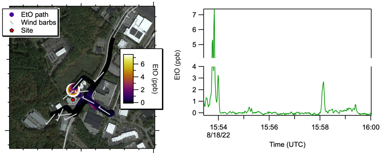
165 Figure S12. Detail of time series downwind of Facility B. A map (left) shows AML path colored by EtO concentration, with wind barbs pointing into the wind. Time series show EtO concentrations zoomed to 0-4 ppb (bottom right) and at full scale (top right). Map underlay: Google, © 2022 CNES / Airbus, MassGIS, Commonwealth of Massachusetts EOE, Maxar Technologies, RIGIS, USDA/FPAC/GEO
