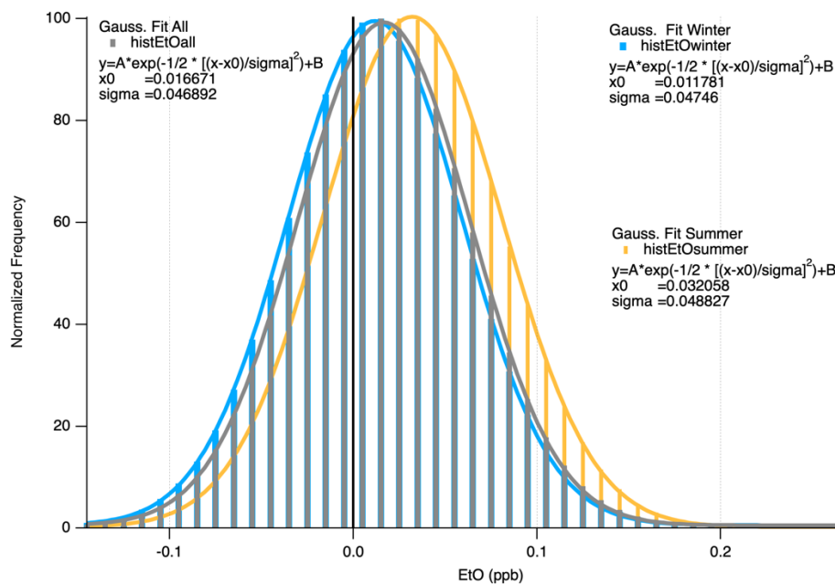
Figure S4. Histogram of 1hr average data in winter/spring (blue), summer (yellow) and all ambient measurements (grey).
