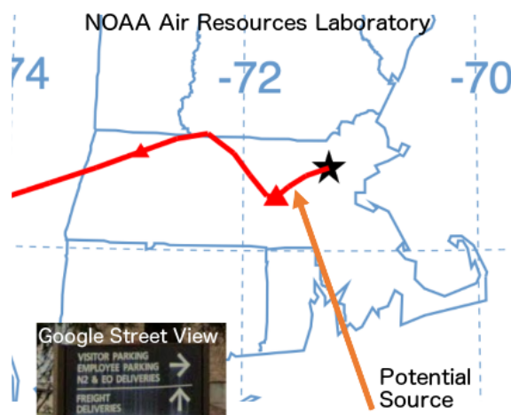
Figure S6. Detail of back trajectory (NOAA Air Resources Laboratory). The orange arrow indicates location of one potential EtO source in the state. A roadside-view of this facility's signage is inset (© Google Street View), with "EO deliveries" noted.
