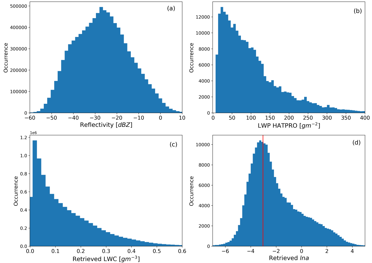
Figure 12. Histogram of (a) Radar reflectivity(Z) (b) LWP from MWR (c) Retrieved LWC (d) Retrieved \ln a for 39 cloudy days, and the red line in \ln a histogram indicates the a priori of \ln a from table 1
