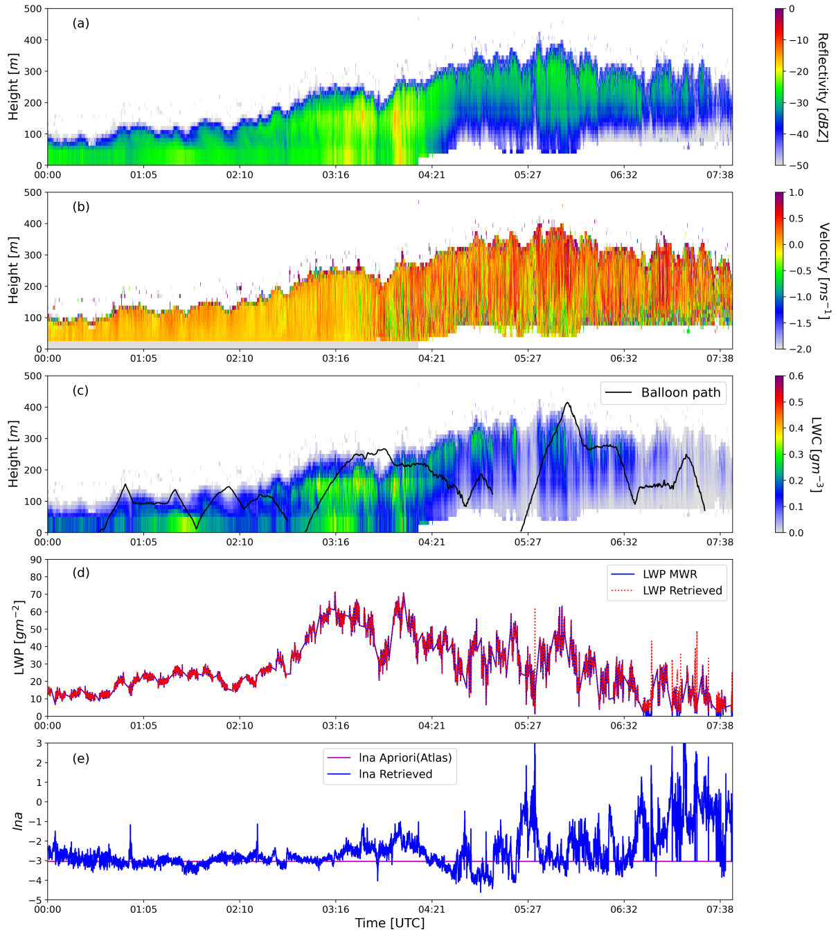
Figure 6. (a) Radar reflectivity Z extended to the lowest gates (b) Doppler velocity plotted only for the available gates (c) Retrieved LWC, (d) LWP and (e) Retrieved \ln a for 09 February 2020 case at SOFOG-3D super-site. Tethered balloon trajectory over retrieved LWC is shown in the black line.
