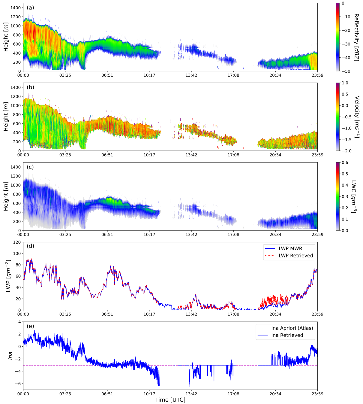
Figure 2. (a) Time-height plot of radar reflectivity (b) Time-height plot of vertical velocity (c) Time-height plot of retrieved LWC, (d) LWP estimated by the radiometer alone through quadratic regression, interpolated at radar time and (e) Retrieved scaling factor lna of each profile for 05 February 2019 case at SIRTa.
