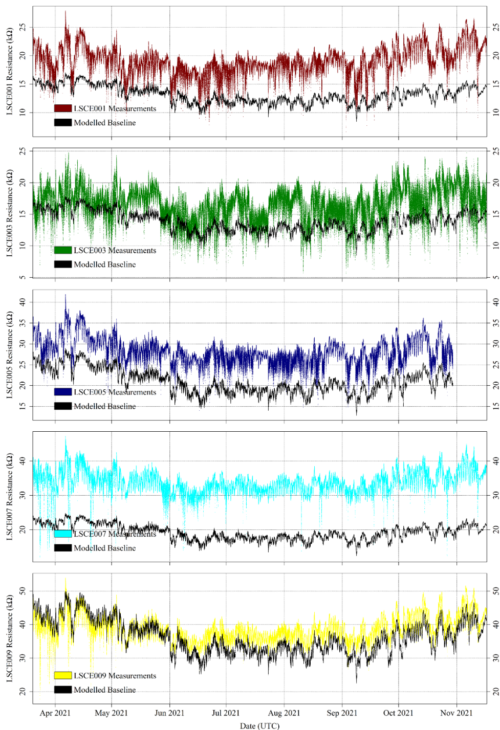
Figure 16: Measured System A Figaro resistance (coloured dots) and modelled standard 2 ppm [CH 4 ] reference resistance (black dots) from the SUEZ Amailloux landfill site for LSCE001, LSCE003, LSCE005, LSCE007 and LSCE009 (top to bottom) between 20 March 2021 and 17 November 2021 (period 1).
