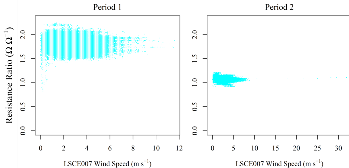
Figure 19: The ratio between measured Figaro resistance and standard 2 ppm [CH 4 ] reference resistance (cyan dots) from the SUEZ Amailloux landfill site for LSCE007, plotted against minute-averaged wind speed as measured by the LSCE007 anemometer, for wind directions between 180° and 270°. Data from period 1 is plotted on the left and data from period 2 is plotted on the right.
