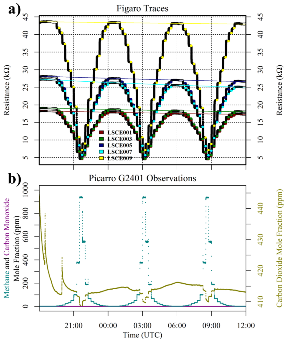
Figure 9: (a) Measured resistance for five Figaro sensors (black dots), under exposure to various methane mole fraction intervals up to 1 000 ppm. Highlighted coloured dots represent 2-minute periods used to derive average resistance values for each methane step (see legend for corresponding sensor colours). White-highlighted dots indicate periods used to derive standard gas reference resistances for each sensor and coloured lines show respective polynomial reference resistance fits. (b) Corresponding mole fraction observations from the Picarro G2401. Methane (dark cyan) and carbon monoxide (dark magenta) mole fraction measurements are plotted on the left-hand axis. Carbon dioxide (dark yellow) mole fraction measurements are plotted on the right-hand axis. Carbon dioxide measurements become unreliable at high methane mole fraction due to spectral overlap.
