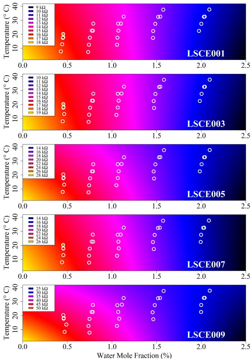
Figure 8: Modelled reference resistance at 2 ppm methane mole fraction (standard gas) for LSCE001, LSCE003, LSCE005, LSCE007 and LSCE009 (coloured background). Points inside white circles represent 30-minute measured resistance averages. Each plot has a unique colour scale (see legend).
