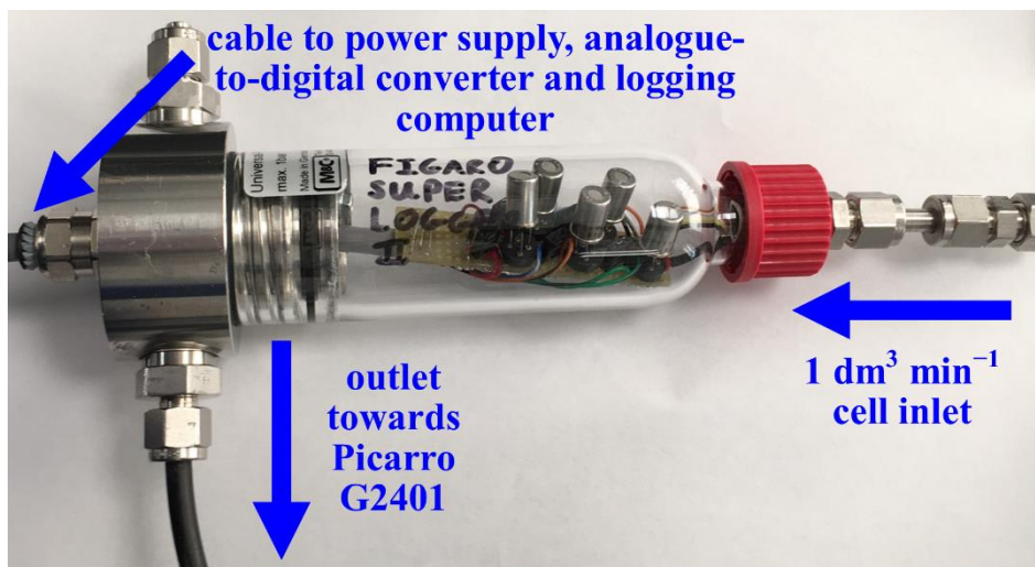
1085 Figure 4: System B laboratory testing logging cell (logging computer and power supply not shown). Five Figaro sensors are plugged into the cell circuit board in this photograph.
