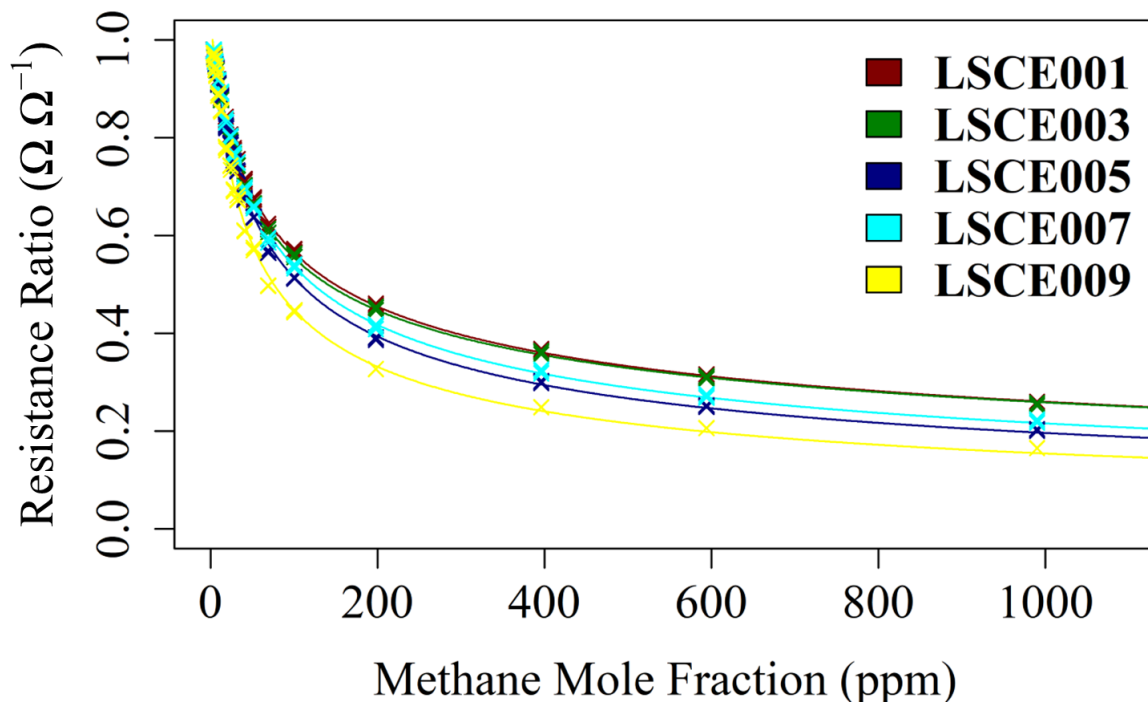
1125 Figure 11: The ratio between each 2-minute average Figaro resistance (from 15-minute sampling intervals) and its corresponding reference resistance estimate (crosses), plotted against methane mole fraction for five Figaro sensors (see legend for respective colours). A model fit for each sensor (coloured lines) is plotted, according to Eq. (6).
