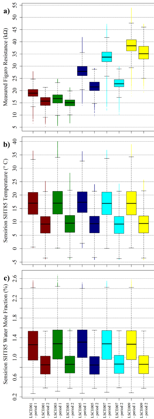
Figure 18: (a) Measured Figaro resistance, (b) measured SHT85 temperature and (c) derived SHT85 water vapour mole fraction (see text for derivation details), from inside each LSCE001, LSCE003, LSCE005, LSCE007 and LSCE009 System A enclosure at the SUEZ Amailloux landfill site, shown as box plots, with outliers presented as coloured dots. Data for period 1 and period 2 are plotted separately.
