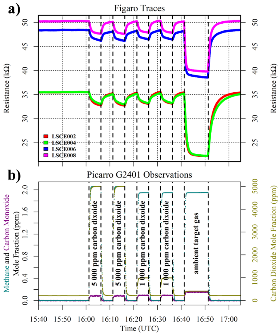
1135 Figure 13: (a) Measured resistance for four Figaro sensors (coloured dots; see legend) in System B, under exposure to 5 000 ppm and 1 000 ppm carbon dioxide mole fraction, compared to gas from a zero-air generator. (b) Corresponding Picarro G2401 observations, with annotations indicating the sampled cylinder type. Areas not annotated correspond to gas from the zero-air generator. Methane (dark cyan) and carbon monoxide (dark magenta) mole fraction measurements are plotted on the left-hand axis. Carbon dioxide (dark yellow) mole fraction measurements are plotted on the right-hand axis. 1140
