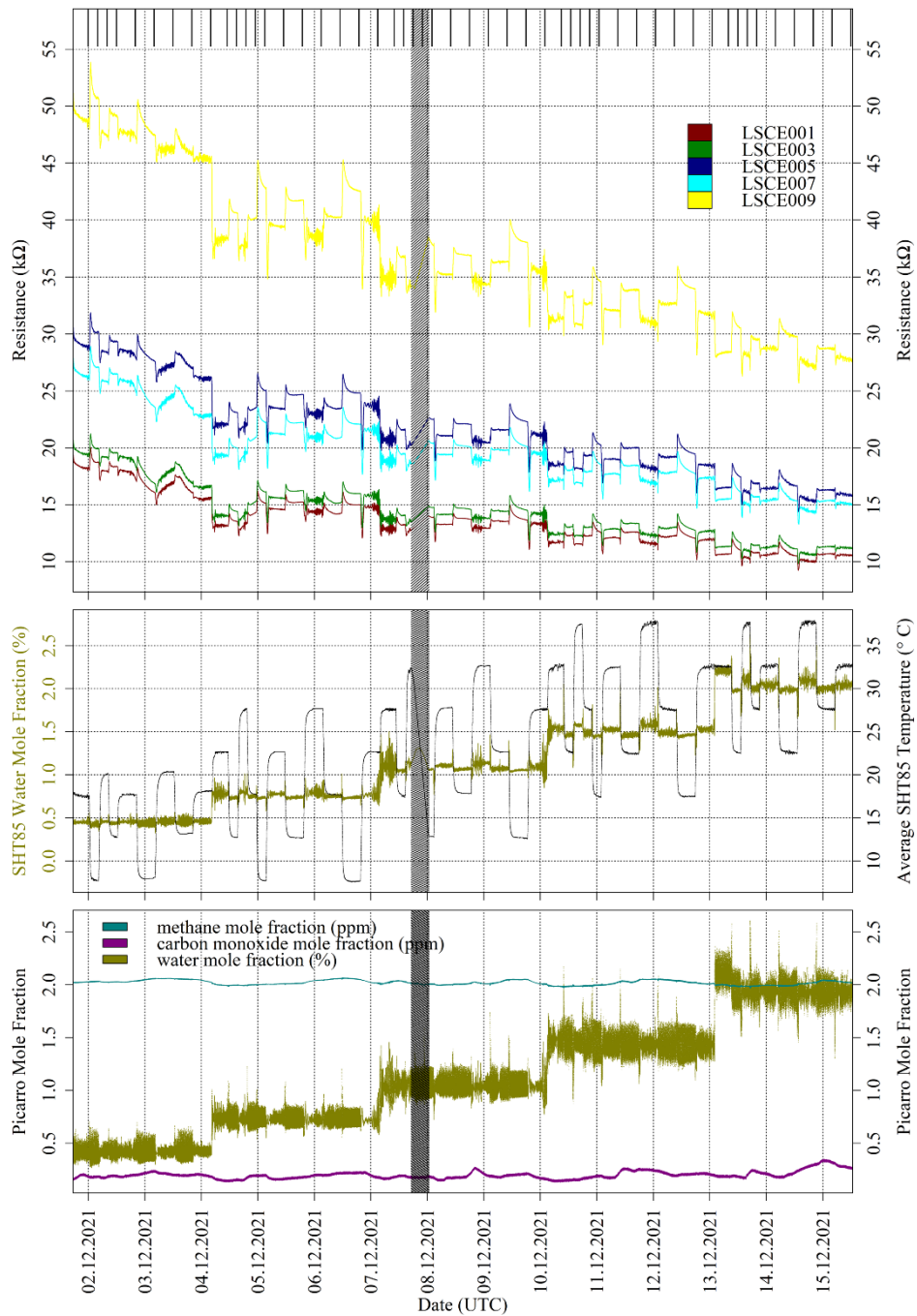
Figure 7: (top) Resistance for five Figaro sensors, sampling inside the environmental chamber (coloured dots; see legend). The black bars at the top of the plot indicate periods used to derive 30-minute averages for each sampling period. The shaded area indicates a data transmission gap. (middle) Derived SHT85 water vapour mole fraction (dark yellow dots) averaged from all five system A boxes plotted against the left-hand axis (see text for derivation details) and measured SHT85 temperature averaged from all five System
