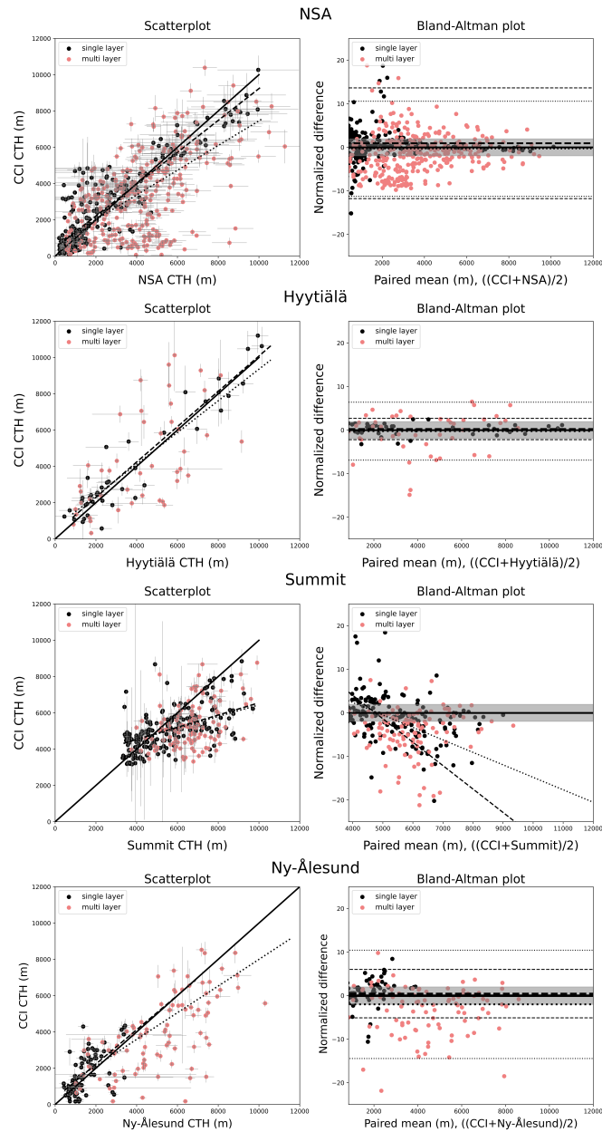
Figure 5. Similar to Fig.3 but for CTH over Hyttiälä (2014), NSA (2012-2016), Ny-Å (2016-2018), and Summit (2010-2014). Tables 3 and 4 lists the corresponding statistics. The data points are classified by single-layer (black) and multi-layer (red) clouds as identified from the ground-based observations. Left: The regression lines for the single-layer cloud cases (dashed) and for all cloud cases (single- and multi-layer; dotted) are shown as well. Right: The BA bias and Limits of Agreements (LOA) are shown for single-layer cloud cases (dashed) and all cloud cases (dotted). Note that the dashed (dotted) line in the BA plot for Summit represents the regression line for single-layer cloud (all cloud) cases instead.
