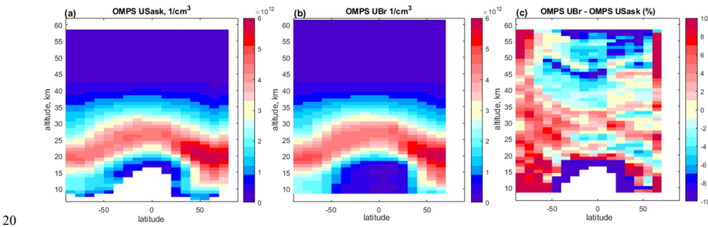
Figure 7. Monthly zonal mean ozone profiles in January 2018 evaluated using OMPS-LP USask data (panel a), OMPS-LP UBr data (panel b). Panel (c): relative difference of OMPS UBr and OMPS USask monthly zonal mean ozone profiles for January 2018.
