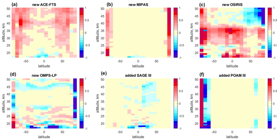
Figure 15 Difference in trend estimated (in % dec -1 ) cause by changes in the datasets (new minus baseline, see text for explanation)
