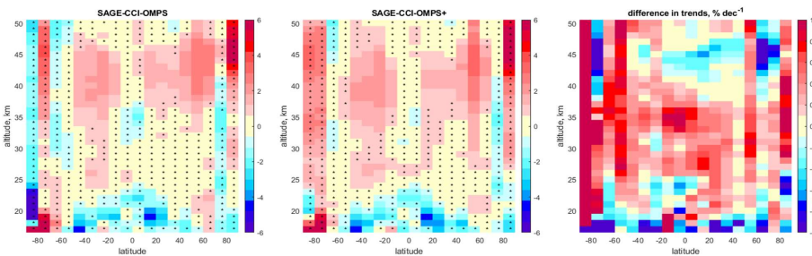
5 Figure 16. Ozone trends in 1997-2020 (% decade -1 ) evaluated using the baseline SAGE-CCI-OMPS dataset (left) and the SAGE-CCI-OMPS+ dataset. Stars indicate the latitude-altitude bins, in which trends are not statistically significant at the 95% confidence level. Right panel shows the difference in ozone trends in % decade -1 (new minus baseline)
