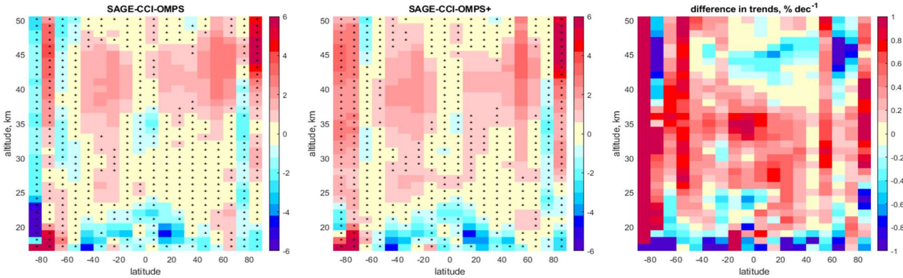
5 Figure 16. Ozone trends in 1997-2020 ( \% \text{ decade}^{-1} ) evaluated using the baseline SAGE-CCI-OMPS dataset (left) and the SAGE-CCI-OMPS+ dataset. Stars indicate the latitude-altitude bins, in which trends are not statistically significant at the 95% confidence level. Right panel shows the difference in ozone trends in \% \text{ decade}^{-1} (new minus baseline)
