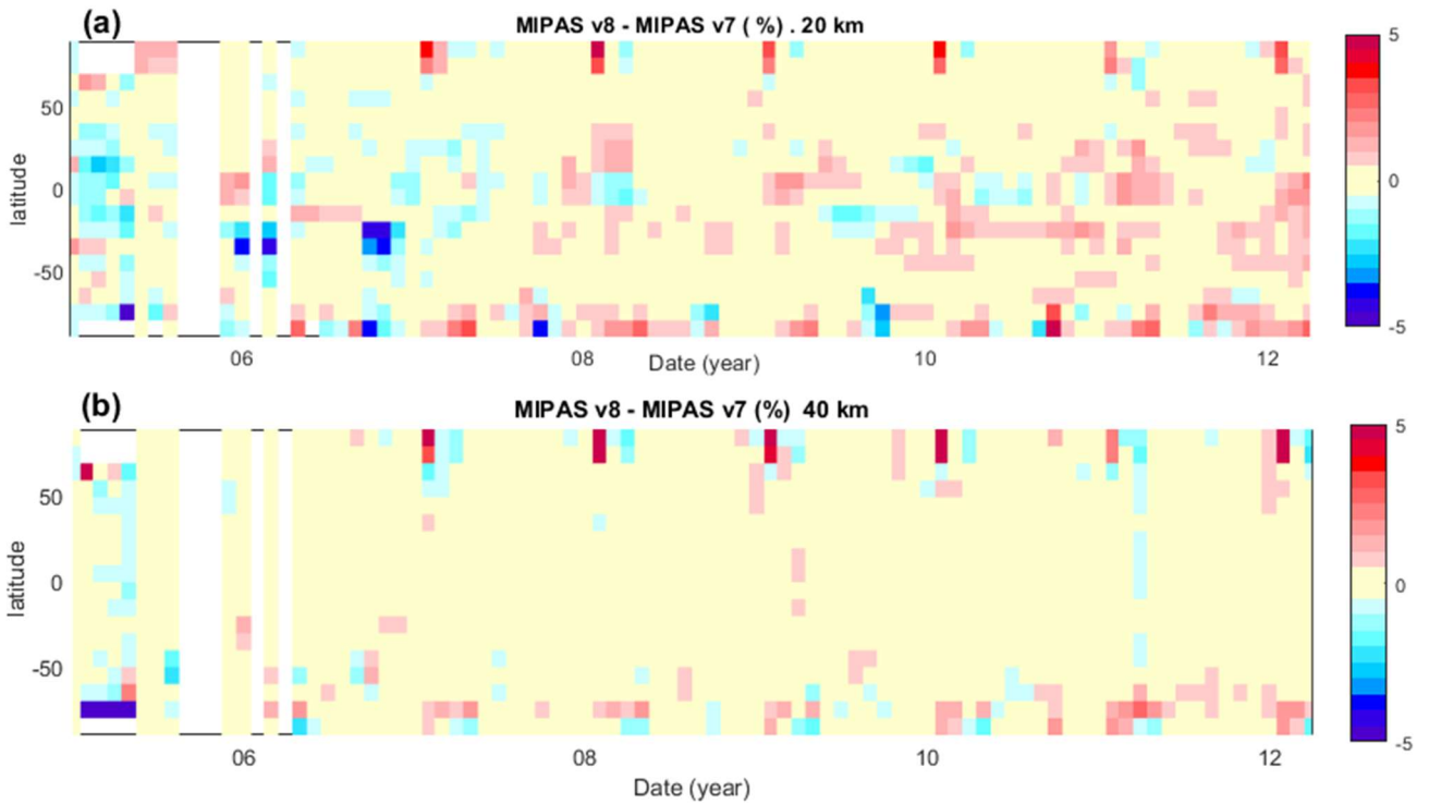
5 Figure 2. Difference in the deseasonalized anomalies between MIPAS v8 and v7 ozone data (v8 minus v7) in %, for altitudes 20 km (panel a) and 40 km (panel b).
