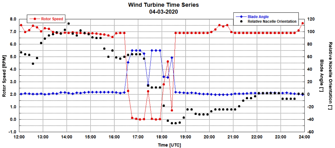
145 Figure 1. Wind turbine rotor speed ( red, left y-axis ), blade pitch angles ( blu, right y-axis ), and relative -nacelle orientation ( black dots, right y-axis ) on March 4, 2020.
