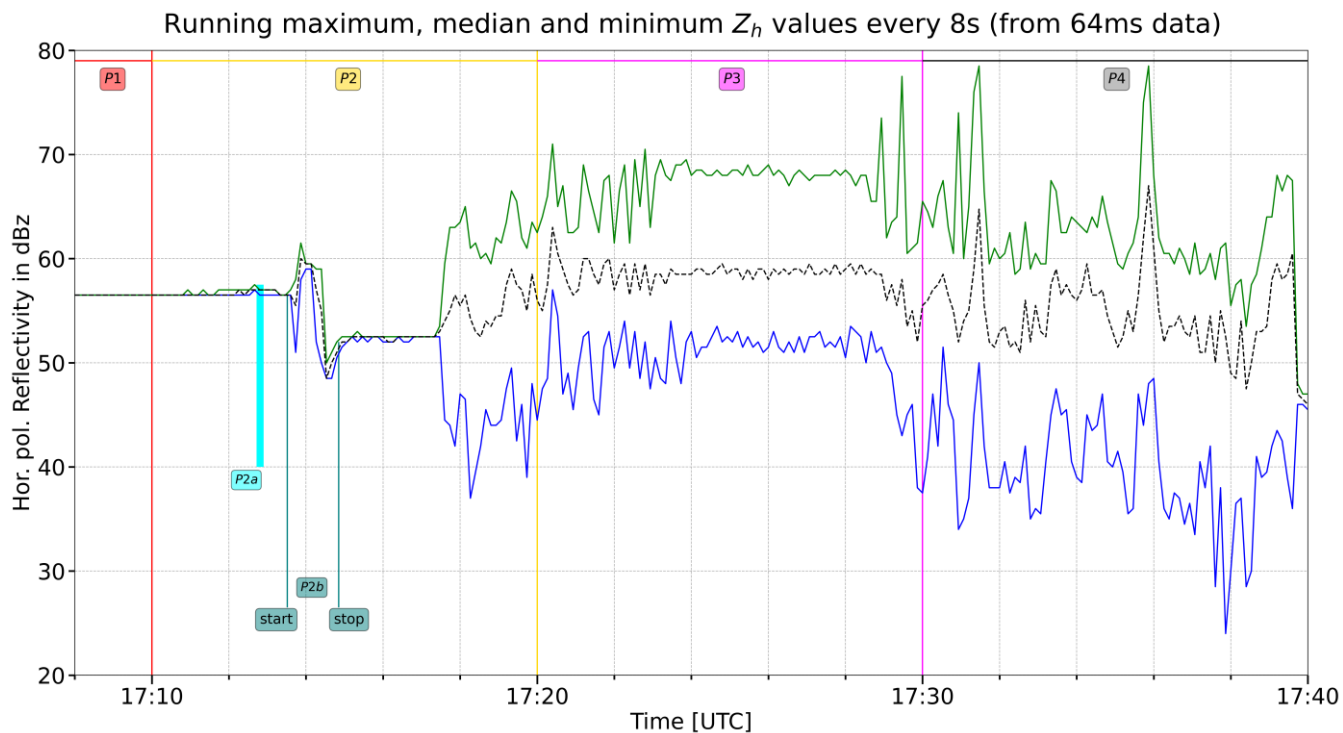
Figure 2. Time line plot of horizontal polarization reflectivity for the 75 m radar gate that contains the pole of the wind turbine. The solid lines join 8 s statistical values (median using black, maximum using green, minimum using blue) obtained by using 125 consecutive radar echoes at the original 64 ms resolution. Being the visualization based on 8 s points, the solid lines consist of 240 points that cover 32 minutes (15 points every 2 minutes, which is in correspondence of the vertical grid lines).
