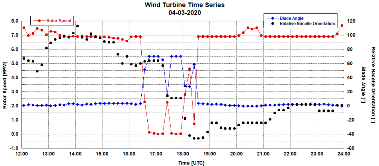
140 Figure 1. Wind turbine rotor speed (red, left y-axis), blade pitch angle (blue, right y-axis), and nacelle orientation (black dots, right y-axis) on March 4, 2020.
