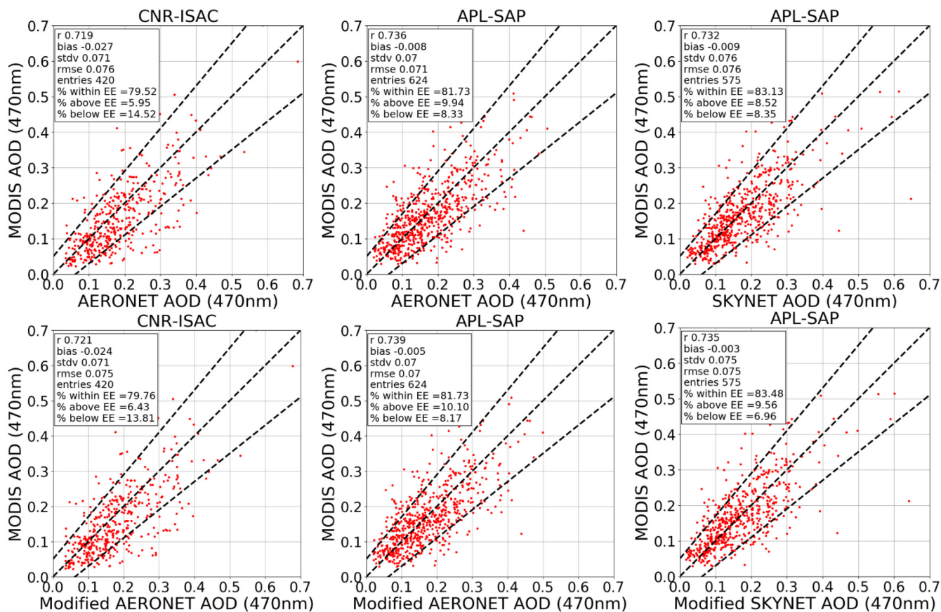
Figure 109: Inter-comparison of MODIS DB with standard (upper panels) and modified (lower panels) ground-based AOD at 470 nm for CNR- ISAC (left panels) and APL-SAP (middle and right panels) sites. In the left and middle panels, against AERONET AOD products, whereas in the right panels against SKYNET AOD. The y=x lines and MODIS DB EE envelopes \pm (0.05 + 20\%) are plotted as dashed lines. The inter-comparison was performed considering a maximum distance between the center of the MODIS DB pixel and the site location of 5 km and \Delta t_{\max} (time between MODIS and AERONET/SKYNET observations) of \pm 30 minutes.
