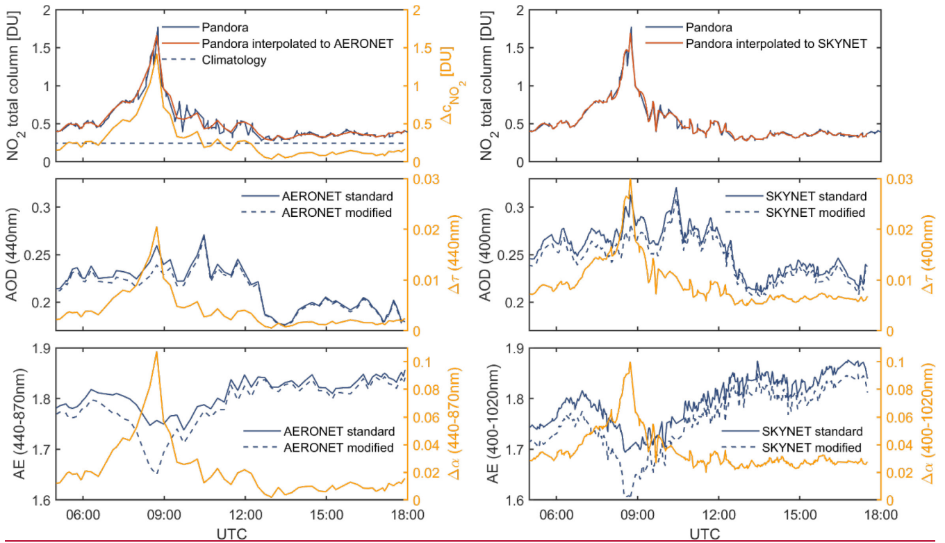
Figure 8: Case study over APL-SAP for 25th June 2020 for both AERONET (left panels) and SKYNET (right panels) . Upper panels: Pandora total NO 2 column and its deviation from climatology. Middle panels: AERONET AOD (solid blue line), its improvement using Pandora NO 2 (dashed blue line) and the magnitude of improvement (light orange line and right y-axis). Lower panels: Similar to middle panels, but for AE retrievals. Note that the spectral channels for the retrievals are different for the two networks.
