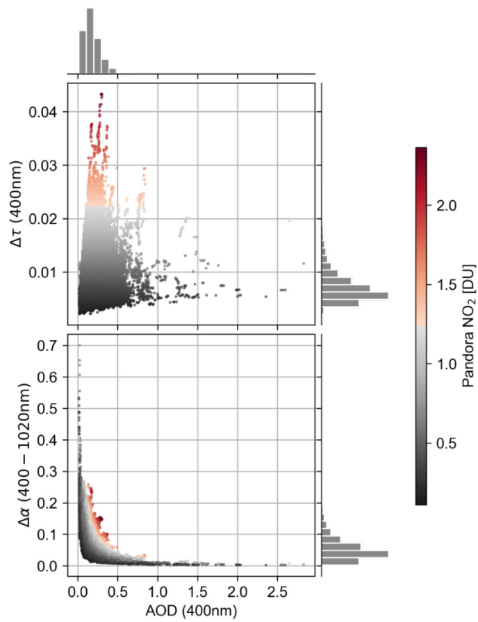
Figure 7: Similar to Fig. 6, but for SKYNET retrievals over APL-SAP. Note that the spectral channels for the retrievals are different compared to AERONET, i.e. 400nm for AOD and 400-1020nm for AE. Also the axis scales are different.
