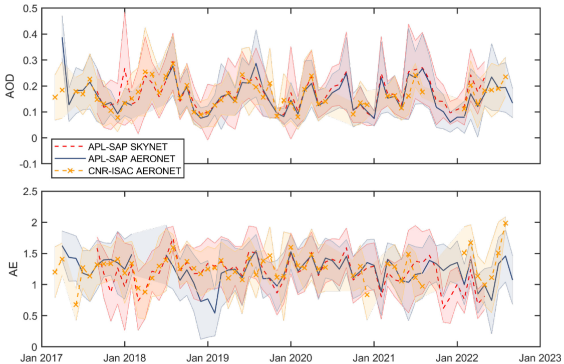
1075 Figure 1: Time series of monthly averaged AOD (upper panel) and AE (lower panel) measurements over APL-SAP (AERONET and SKYNET) and CNR-ISAC (AERONET). Note that AERONET AOD and AE correspond to the wavelength channels of 440nm and 440-870nm, respectively, whereas SKYNET AOD and AE refer to 400nm and 400-1020nm, respectively. The shaded areas correspond to the monthly 1-sigma standard deviation.
