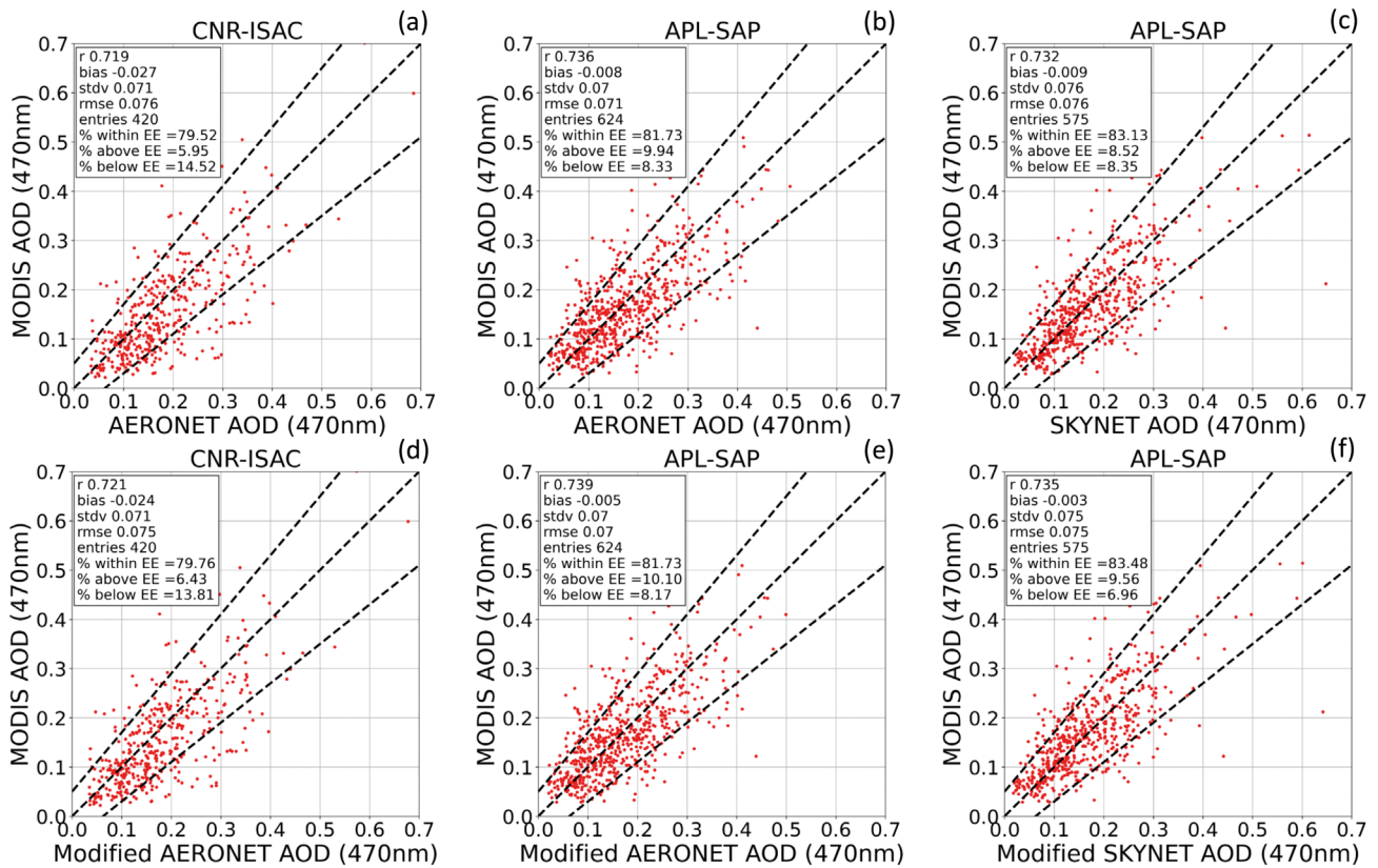
1060 Figure 9: Inter-comparison of MODIS DB with standard (a, b, c) and modified (d, e, f) ground-based AOD at 470 nm for both CNR-ISAC (a, d) and APL-SAP (b, c, e, f) sites against AERONET AOD (a, b, d, e) and SKYNET AOD (c, f). The y=x lines and MODIS DB EE envelopes \pm (0.05 + 20\%) are plotted as dashed lines. The inter-comparison was performed considering a maximum distance between the center of the MODIS DB pixel and the site location of 5 km and \Delta t_{\max} (time between MODIS and AERONET/SKYNET observations) of \pm 30 minutes.
