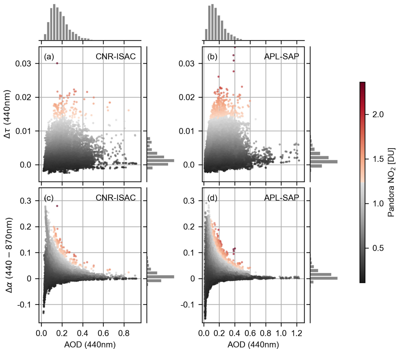
1040 Figure 6: The differences of modified AERONET AOD at 440 nm (a, b) and AE at 440-870 nm (c, d) over CNR-ISAC and APL-SAP from the standard products illustrated with respect to the standard AERONET AOD measurements at 440 nm and the actual \text{NO}_2 observed by Pandora (color scale). The corresponding distributions of all variables are also included.
