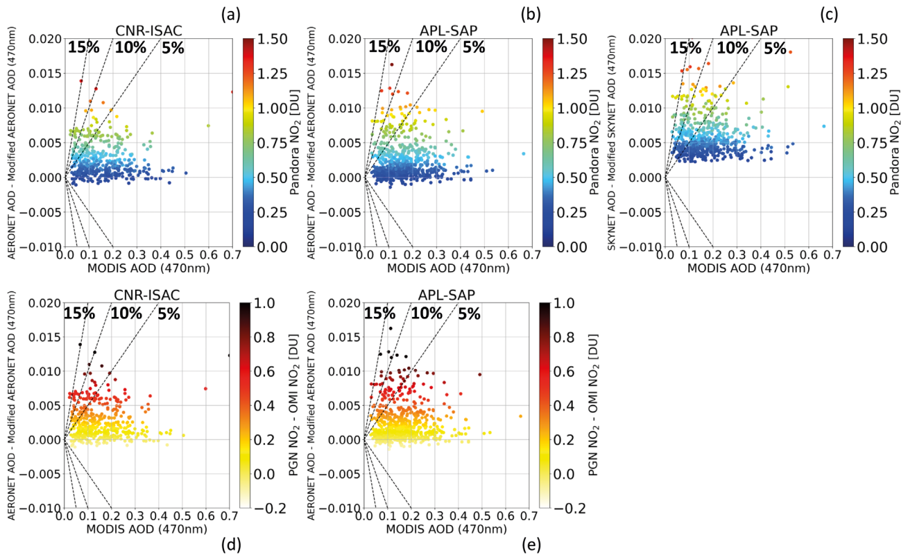
1065 Figure 10: (a, b, c) Absolute correction as a function of the corresponding MODIS DB AOD data and PGN NO 2 data (color scale) for both CNR-ISAC and APL-SAP sites using AERONET and SKYNET AOD. The analysis was performed considering a maximum distance between the center of the MODIS DB pixel and the site location of 5 km and \Delta t_{\max} of \pm 30 minutes. (d, e) Absolute correction of the MODIS DB AOD data for both CNR-ISAC and APL-SAP using AERONET AOD as a function of the corresponding MODIS DB AOD data and the absolute difference between PGN and OMI climatological NO 2 (color scale).
