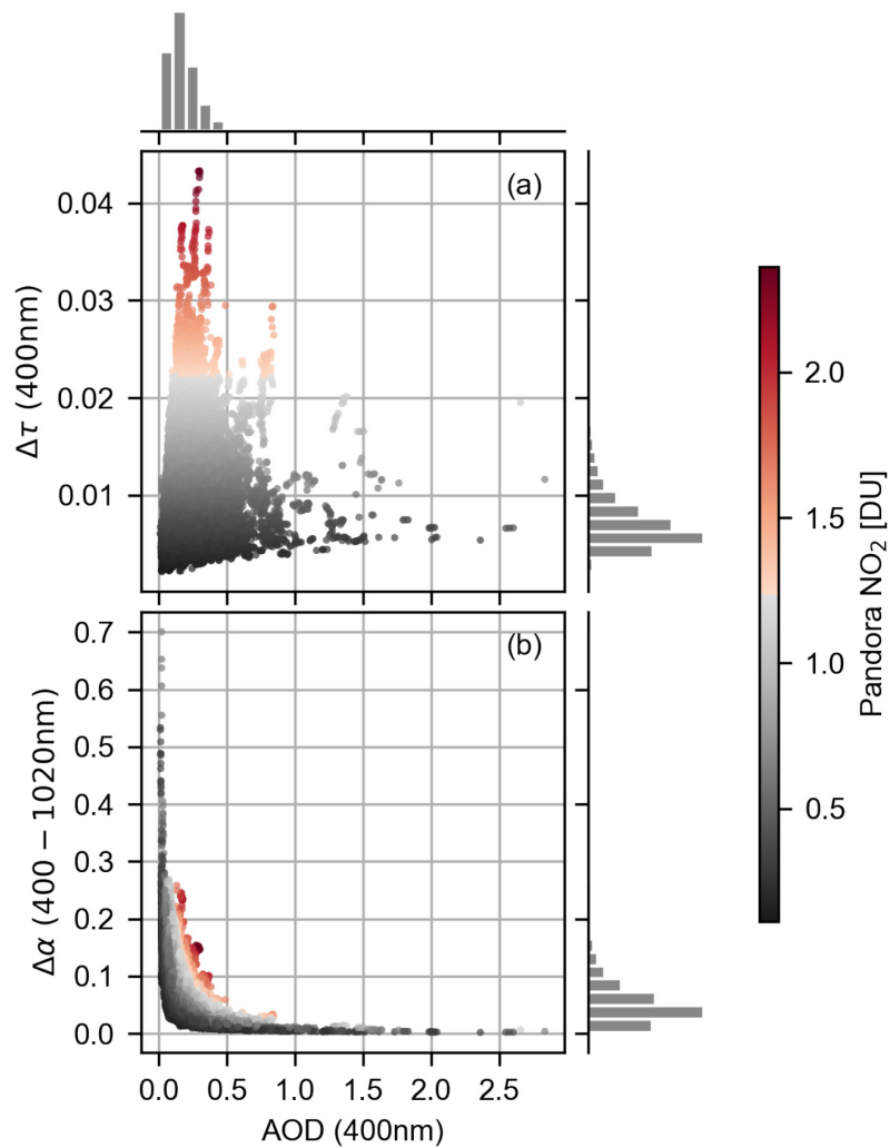
1045 Figure 7: The differences of modified SKYNET AOD at 400 nm (a) and AE at 400-1020 nm (b) over APL-SAP from the standard products illustrated with respect to the standard SKYNET AOD measurements at 400 nm and the actual NO 2 observed by Pandora (color scale). The corresponding distributions of all variables are also included. Note that the spectral channels for the retrievals and the axis scales are different compared to AERONET.
