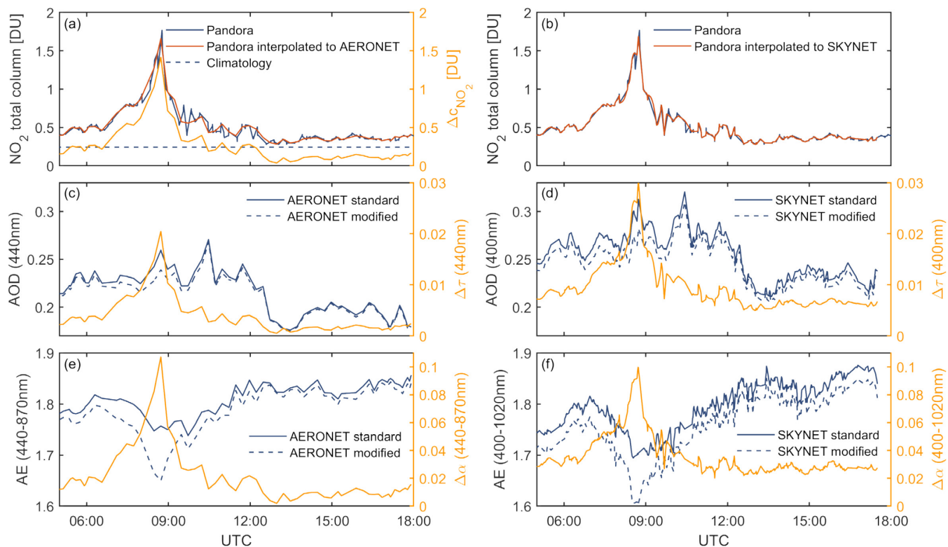
Figure 8: Case study over APL-SAP on 25th June 2020 for both AERONET and SKYNET. (a, b) Pandora total NO 2 column and its deviation from climatology. (c, d) AOD (solid blue line), its improvement using Pandora NO 2 (dashed blue line) and the magnitude of improvement (light orange line and right y-axis). (e, f) Similar to (c, d), but for AE retrievals. Note that the spectral channels for the retrievals are different for the two networks.
