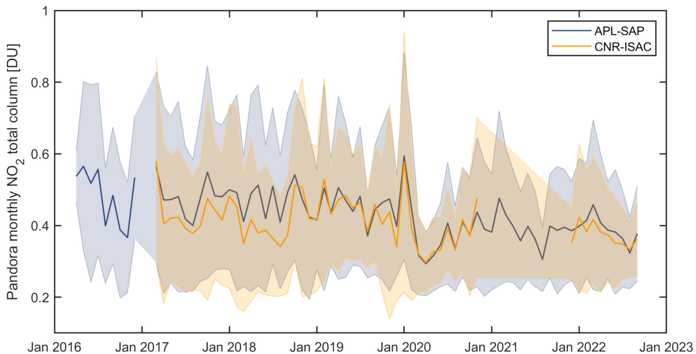
1020 Figure 2: Time series of monthly NO 2 total column from Pandora instruments over APL-SAP (blue line) and CNR-ISAC (yellow line). The shaded areas correspond to the 1-sigma standard deviation of the monthly averaged values. The NO 2 concentration is clearly affected by the COVID-19 lockdown during February – May 2020.
