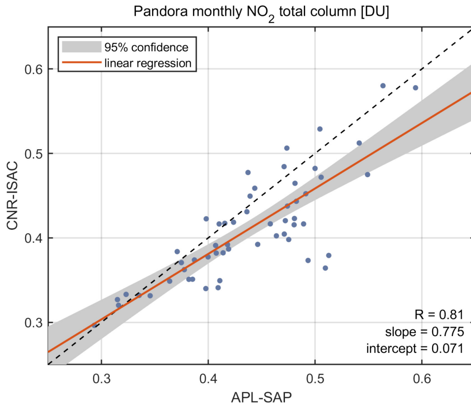
Figure 3: Monthly NO 2 total column from Pandora over CNR-ISAC against synchronous APL-SAP observations. The grey shaded area corresponds to the 95% confidence interval of the linear regression fit (red line).
