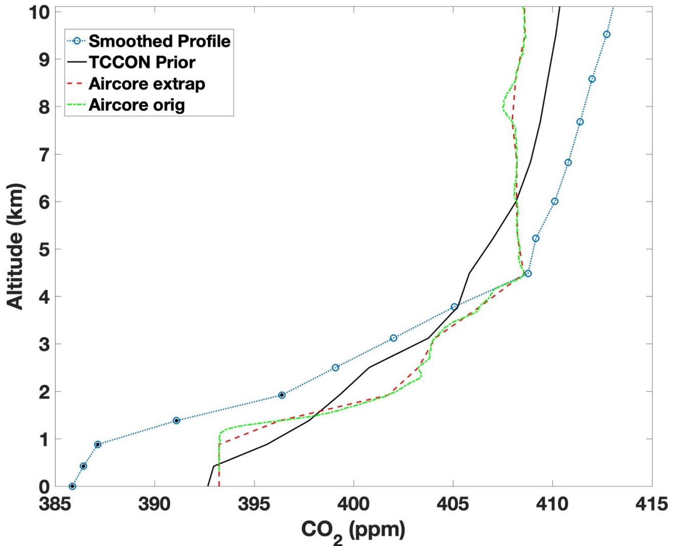
570 Figure 4. An example of the profiles used in the direct comparison calculations using data from the Park Falls site on July 27, 2018. The profile above 10 km is not shown. The solid black line is the TCCON a priori profile scaled by the median of the vertical scaling factors from the spectral windows used. The green dot-dashed line is the measured AirCore mole fraction. The red, dashed line is the AirCore measurements interpolated to the vertical spacing of the TCCON prior, and the blue, dotted line with circles is the smoothed, vertical sensitivity weighted profile that is integrated to calculate the 575 partial column that the TARDISS retrieval would calculate if it had a ‘true,’ AirCore profile. The black dots within the blue circles represent the points of the profile that make up the lower partial column.
