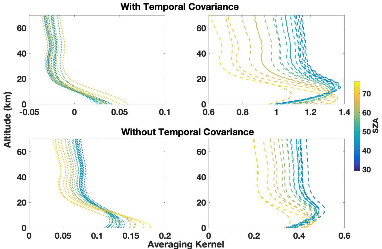
Figure 8. Vertical sensitivities of the lower partial column (left column) and upper partial column (right column) scalars color coded by solar zenith angle in degrees. The sensitivities calculated when using a temporally covariant a priori covariance matrix are shown in the top row and when using a non- 845 temporally covariant a priori covariance matrix are shown in the bottom row.
