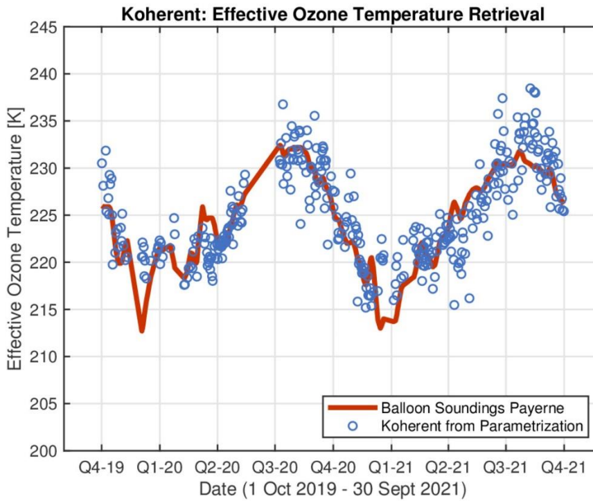
720 Figure 7: Effective ozone temperature derived from the parametrization of differences between CDR retrieval from Brewer and Dobson wavelength and slit function settings.
