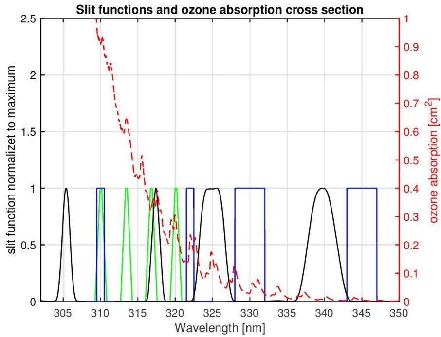
680 Figure 2: Slit functions of the Custom Double Ratio technique for Koherent (blue), the trapezoidal slit functions of the Brewer (green) and the measured slit function of Dobson 101 (black). The red dashes line indicates the ozone absorption cross section SG14 at effective temperature of 228 K.
