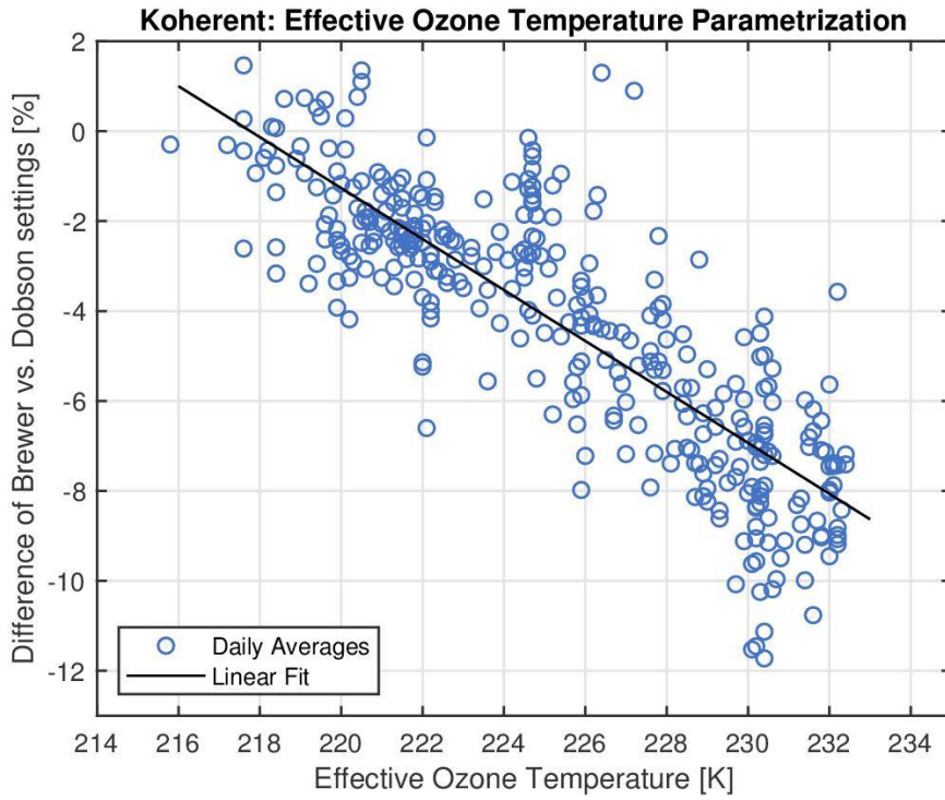
710 Figure 6: Parametrization of the relative differences between CDR retrieval using Dobson and Brewer wavelength and slit function settings at 228 K effective ozone temperature, with daily effective ozone temperature from balloon soundings. The linear fit exhibits a slope of 0.5%/K indicating the sensitivity of the differences to effective ozone temperature.
