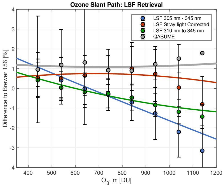
685 Figure 3: Ozone slant path comparison of Koherent LSF retrieval with the double monochromator Brewer 156 for the wavelength range of 305 – 345 nm retrieval (blue), the wavelength range of 310 – 345 nm retrieval (green), and stray light corrected retrieval (red). For comparison, the performance of QASUME is indicated in grey. The lines indicate quadratic fits to all measurements, which are not specifically shown. The circles are averages on 100 DU bins.
