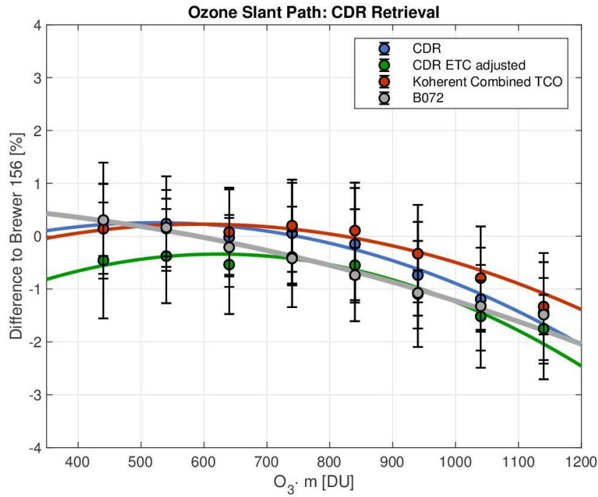
695 Figure 4: Ozone slant path comparison of Koherent CDR retrieval with the double monochromator Brewer 156 for standard CDR retrieval (blue), ETC adjusted CDR retrieval (green), and LSF/CDR combined retrieval (red). For comparison, the performance of the single monochromator Brewer 072 is indicated in grey. The lines indicate quadratic fits to all measurements, which are not specifically shown. The circles are averages on 100 DU bins.
