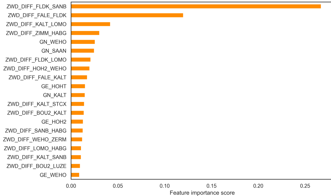
Figure 6. Feature importance score of the 20 strongest predictors for the GB algorithm, when using the FS3 setup.
