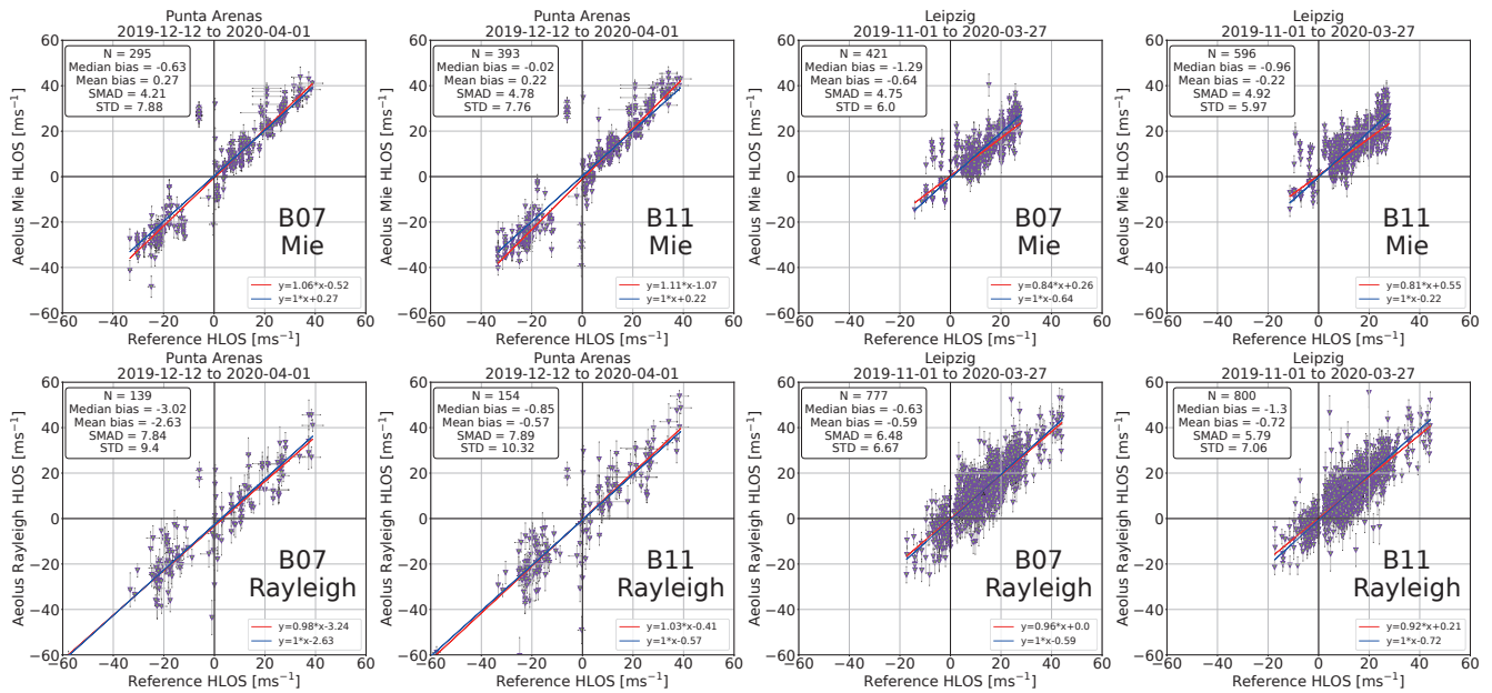
Figure 12. Aeolus performance at the reference stations of Punta Arenas (left, cloud radar, ascending and descending orbit) and Leipzig (right, radiosondes, ascending orbit) for Baselines 07 and 11 in the period from November 2019 to April 2020. Plots in analogy to Figures 6 and 7, left.
