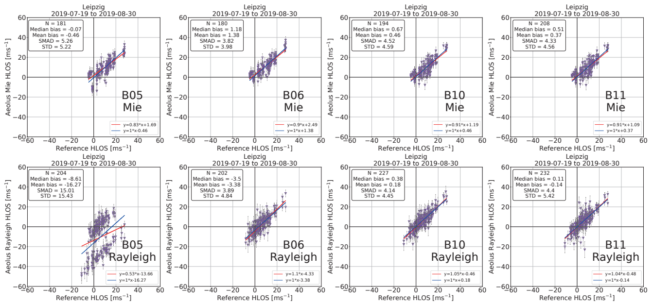
Figure 10. Aeolus performance as obtained by comparison to radiosonde launches at Leipzig (ascending orbit only) for Baselines 05, 06, 10, and 11 in the period from July to August 2019. Plots in analogy to Figures 6 and 7, left.
