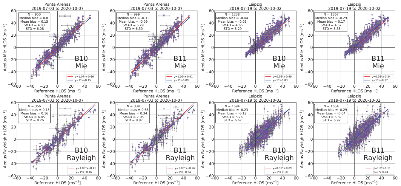
Figure 14. Aeolus performance at the reference stations of Punta Arenas (left, cloud radar, ascending and descending orbit) and Leipzig (right, radiosondes, ascending orbit only) for Baselines 10 and 11 in the period from July 2019 to October 2020. Plots in analogy to Figures 6 and 7, left.
