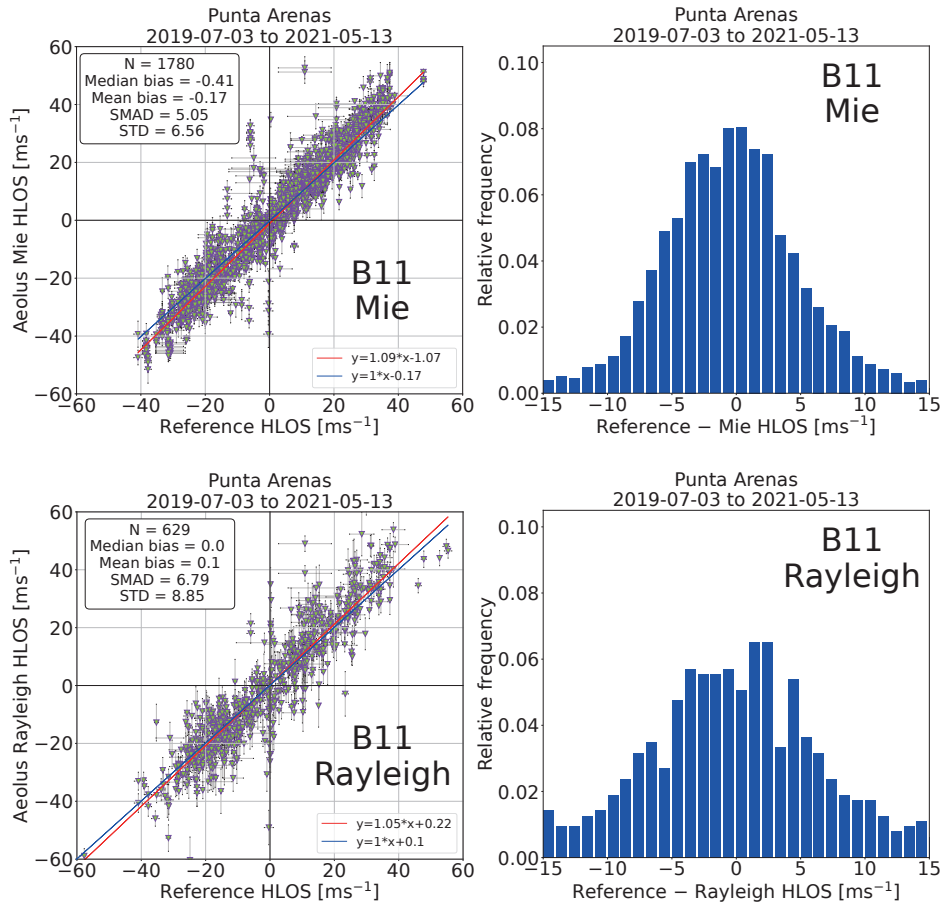
Figure 6. Long-term wind statistic for the Baseline-11-wind-validation based on ground-based Doppler cloud radar observations at Punta Arenas (ascending and descending orbit). Top: Aeolus Mie wind, bottom: Rayleigh wind, left: 1:1 statistic with respective measures (median and mean bias, scaled median absolute deviation (SMAD), and standard deviation (STD) provided in \text{ms}^{-1} , and N indicating the number of samples), right: frequency distribution of differences between the two data sources.
