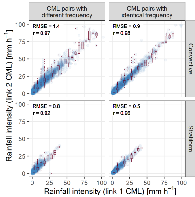
645 Figure 10: Scatter plots of CML-derived rainfall intensity for collocated CML pairs of (left column) different frequency band and (right column) identical frequency band in 1-min temporal resolution for (top row) convective and (bottom row) stratiform rainfall events. In the top left corner are the performance measures (correlation and RMSE in \text{mm h}^{-1} ). Values under 100 \text{ mm h}^{-1} are shown.
