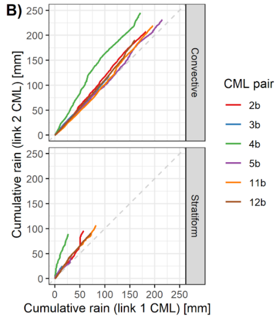
Figure 9: (left) Double-mass curve for collocated sensors operating at different frequency bands. The curve, which differs the most from the line y = x , belongs to site 4b. (right) The same, but the convective and stratiform rainfall types are separated.
