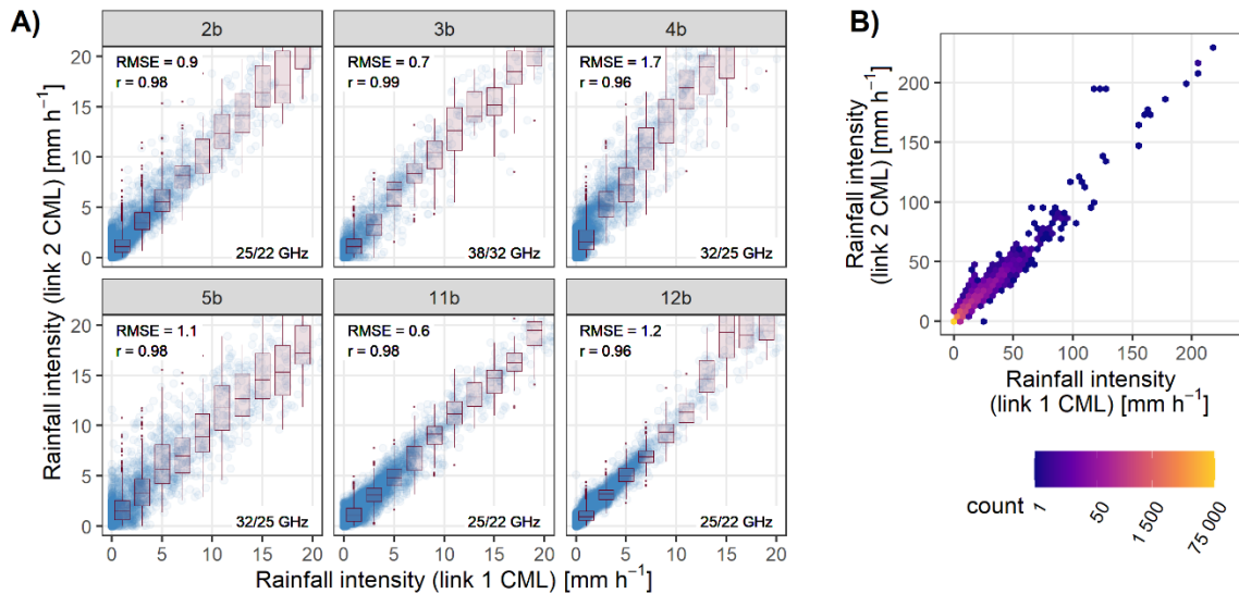
Figure 8: (left) Scatter plot of CML-derived rainfall intensity for six collocated CML pairs having different frequencies. Values under 20 mm h -1 are shown. The boxplots show a spread when binned to 2 mm h -1 bins by link 1. The performance metrics (correlation and RMSE in mm h -1 ) are in the top left corner and the frequency band is indicated in the bottom right corner for each site. (right) Scatter density plot of rainfall intensity for all pairs at the full range of values.
