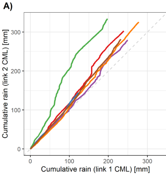
Figure 9: (left) Double-mass curve for collocated sensors operating at different frequency bands. The curve, which differs the most from the line y = x , belongs to site 4b. (right) The same, but the convective and stratiform rainfall types are separated.
