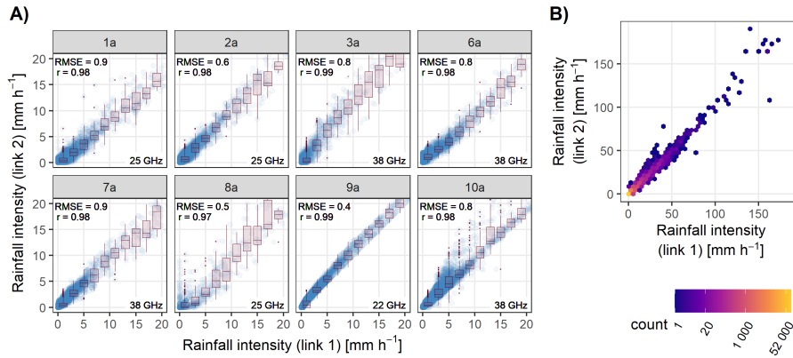
Figure 6. (left) Scatter plot of CML-derived rainfall intensity for eight collocated CML pairs having identical frequencies. Values under 20 \text{ mm h}^{-1} are shown. The boxplots show a spread when binned to 2 \text{ mm h}^{-1} bins by link 1. The performance metrics (correlation and RMSE in \text{mm h}^{-1} ) are in the top left corner and the frequency band is indicated in the bottom right corner for each site. (right) Scatter density plot of rainfall intensity for all pairs at the full range of values.
