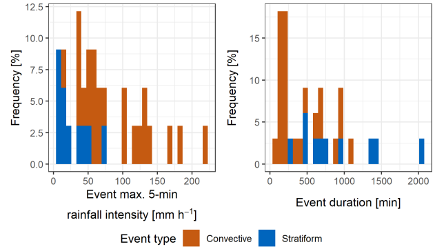
Figure 3. Characteristics of 33 selected rainfall events. (left) Histogram of maximum event rainfall intensity based on 5-min moving average of 23 municipal rain gauge measurements. (right) Histogram of event durations. The colour indicates the type of rainfall event (convective or stratiform).
