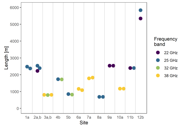
Figure 2. Distribution of lengths and frequencies of CMLs used in this study. The colours indicate the frequency band at which CMLs operate. The "a" in the name of the site indicates pairs of CMLs having identical frequency bands and "b" indicates pairs of CMLs having different frequency bands.
