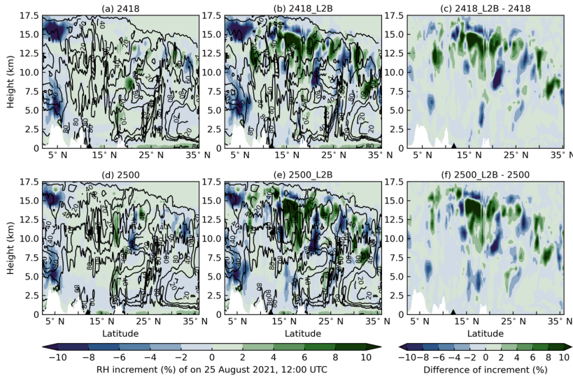
Figure 10: As in Fig. 9, but for RH.
