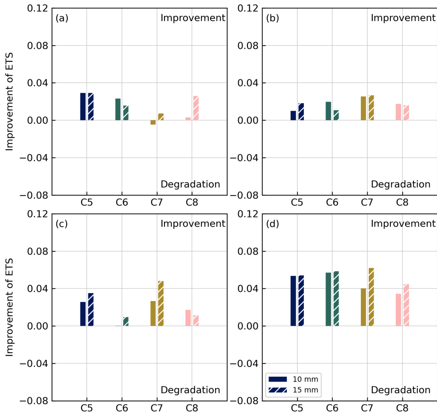
545 Figure 6: Improvements of the 48 h averaged ETSs of forecasts initialized from the analysis DA cycles 5 (blue), 6 (green), 7 (brown), and 8 (pink) for different precipitation thresholds: 10 mm (without white lines) and 15 mm (with white lines) in experiments 2406_L2B (a), 2412_L2B (b), 2418_L2B (c), and 2500_L2B (d), compared with the corresponding experiments without assimilation of Aeolus HLOS winds. The ETS scores are calculated using the forecasts of 6 h accumulated precipitation against the IMERG precipitation data within a 10^\circ \times 10^\circ box centered on Hurricane Ida (2021).
