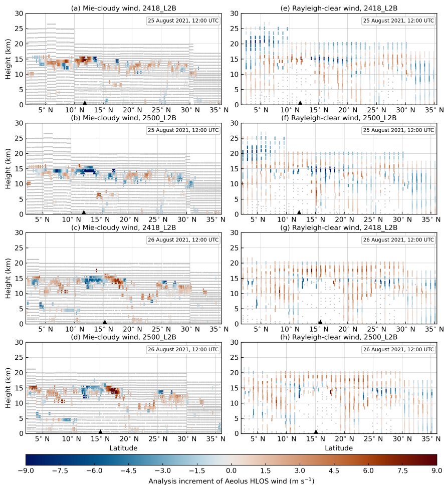
635 Figure 8: Vertical cross sections of analysis increments of Mie-cloudy winds for the Aeolus descending measurement swath close to the center of Ida (2021) in experiments 2418_L2B (a) and 2500_L2B (b) on 25 August 2021, 12:00 UTC. The triangles indicate the locations of Ida (2021) in the simulations on 25 August 2021, 12:00 UTC. (c)-(d) As in (a)-(b) but for 26 August 2021, 12:00 UTC. (e)-(h) As in (a)-(d), but for Rayleigh-clear winds.
