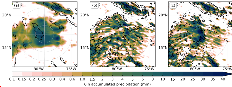
765 Figure 12: (a) 6 h accumulated IMERG precipitation (color shading) from 21 August 2021, 18:00 UTC to 22 August 2021, 00:00 UTC and divergence over 5 \times 10^{-5} \text{ s}^{-1} at 850 hPa (black contour) from the GFS analysis on 22 August 2021, 00:00 UTC. (b)-(c) As in (a), but the precipitation and divergence are calculated by the WRF model simulations of experiment 1918 (b) and experiment 1918_L2B (c). The gray circles indicate radii of 150, 300, and 450 km, respectively.
