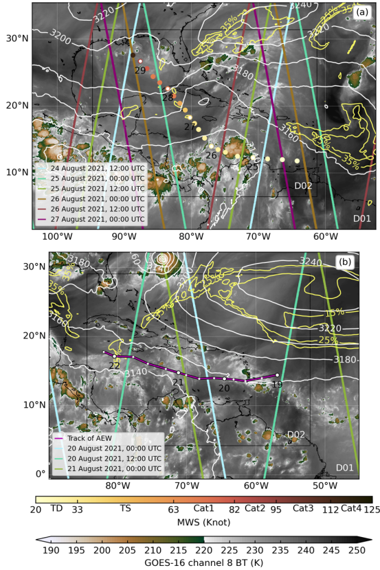
110 Figure 1: Two nested domains (d01: 12 km, and d02: 4 km) in experiments 2418_L2B (a) and 1918_L2B (b). The Aeolus measurement swaths (colored line) are from 24 August 2021, 12:00 UTC to 27 August 2021, 00:00 UTC (a) and from 20 August 2021, 00:00 UTC to 21 August 2021, 00:00 UTC (b). The track and maximum surface wind speeds (MWSs, colored dot) of Hurricane Ida (2021) in (a) are adopted from the NHC best-track data, and the days are illustrated below the open markers indicating 00:00 UTC. Two classifications (TD: tropical depression; TS: tropical storm) and different categories (Cat1: Category 1; Cat2: Category 2; Cat3: Category 3; Cat4: Category 4) based on the Saffir-Simpson Hurricane wind scale are given below the color bar of MWS. The AEW in (b) is tracked manually using the GFS-analyzed relative vorticity maxima at 700 hPa (purple line with black edges). The white dots with the numbers below along the AEW track indicate 00:00 UTC of a day. The geopotential height at 700 hPa (white line) and relative humidity at 850 hPa (RH; yellow line), obtained from GFS analysis, are overlaid atop GOES-16 channel 8 brightness temperatures (BTs; shaded), on 25 August 2021, 12:00 UTC (a), and 21 August 2021, 00:00 UTC (b). Only RH less than 35% is shown in (a) and (b). 115 120
