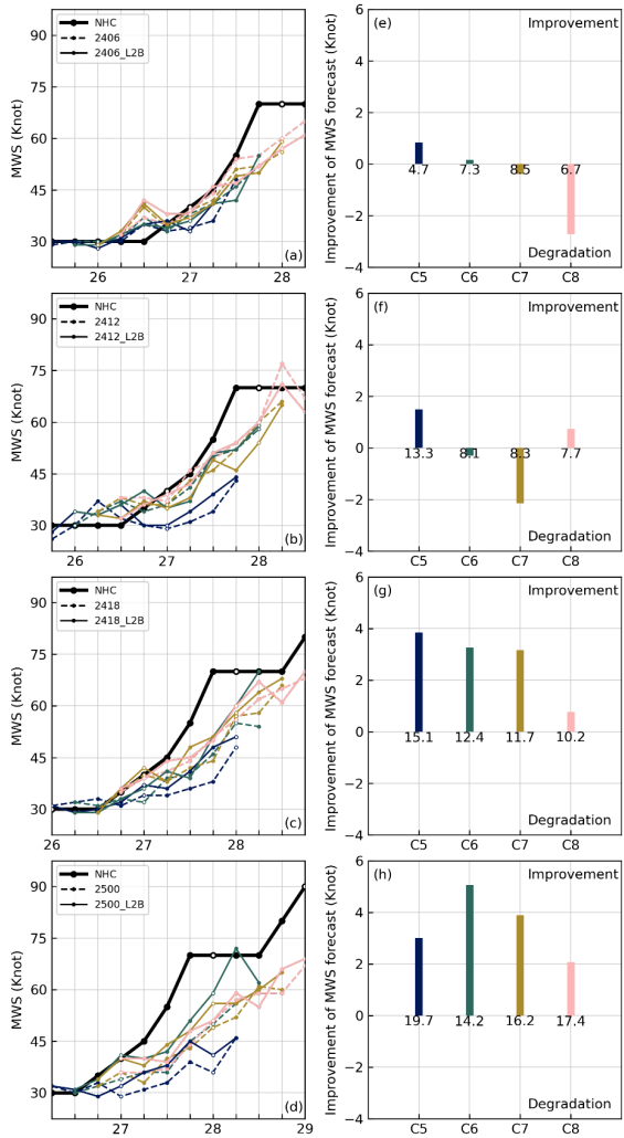
Figure 5: As in Fig. 3, but for MWS forecasts.
