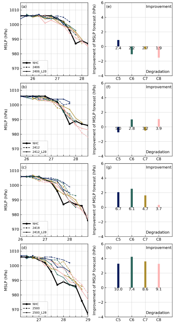
515 Figure 4: As in Fig. 3, but for MSLP forecasts.
