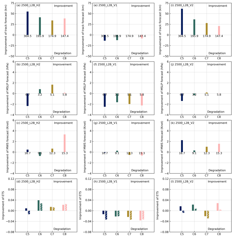
Figure 7: The reductions of the 48 h averaged track forecast errors (a), MSLP forecast errors (b), MWS forecast errors (c), and the improvements of ETSs (d) for DA cycles 5 (blue), 6 (green), 7 (brown), and 8 (pink) in experiments 2500_L2B_H2, compared with experiment 2500_L2B. Positive values of reductions of track, MSLP, and MWS forecast errors mean improvement, while negative values indicate degradation. (e)-(h), and (i)-(l) as in (a)-(d), but for experiments 2500_L2B_V1, and 2500_L2B_V2.
