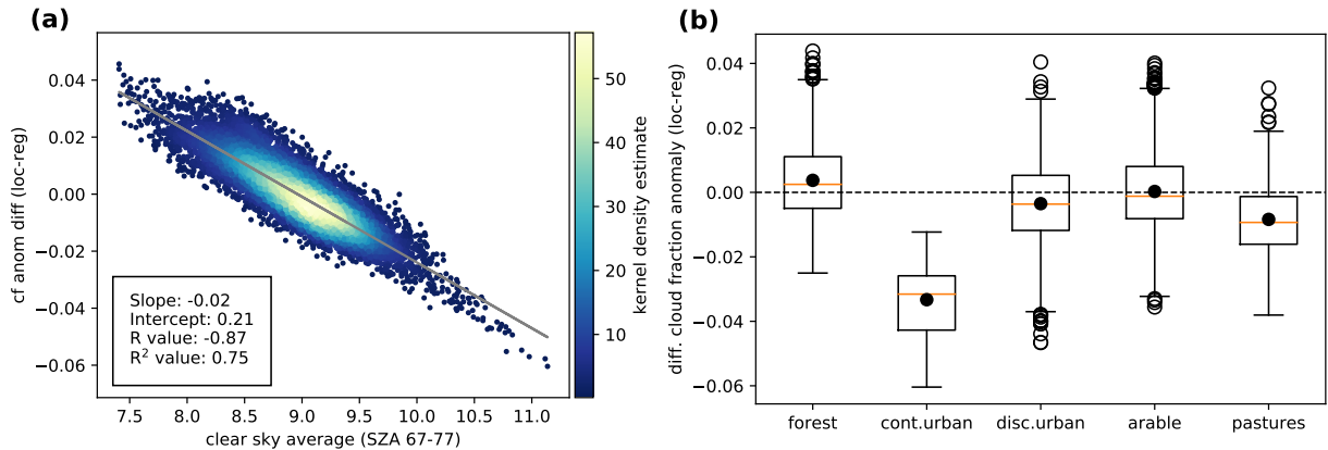
Figure 5. a) Linear regression: Difference of cloud fraction anomalies (LECD-RECDA) vs. clear sky reflectance (average of SZA bins 67-77). Bright colors represent a higher probability density of the data points using Gaussian kernels. b) Difference of cloud fraction anomalies ( CF_{loc} anomaly - CF_{reg} anomaly ) from Local and Regional Empirical Cloud Detection Approaches grouped by 5 main Corine Land Cover types: forest, continuous urban fabric, discontinuous urban fabric, arable land and pastures. Median and mean of each class are presented as orange horizontal lines and black dots, respectively. Whiskers are equal to 1.5 times IQR beyond the first and third quartiles. Outliers are shown as black circles.
