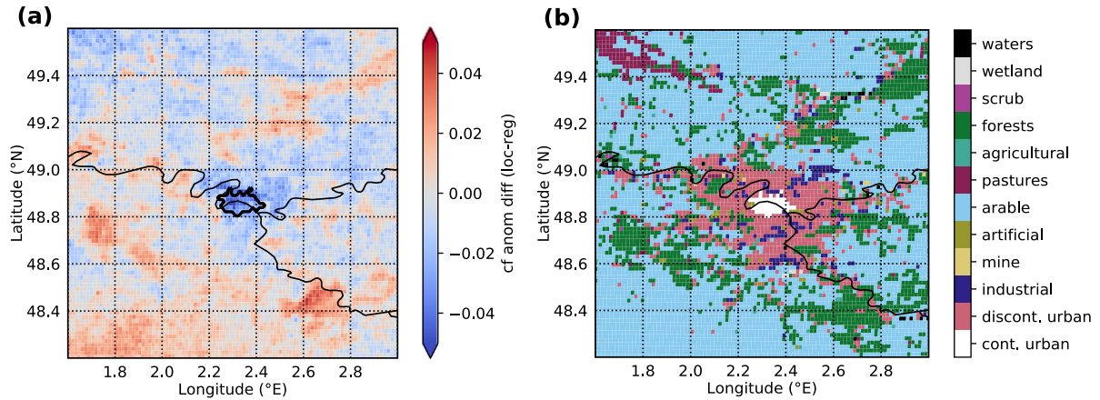
Figure 4. a) Difference of cloud fraction anomalies ( CF_{loc} anomaly - CF_{reg} anomaly ) from Local and Regional Empirical Cloud Detection Approaches. b) Main Corine Land Cover classes L2 and L3 for the year 2012. Larger rivers are visualized as black lines.
