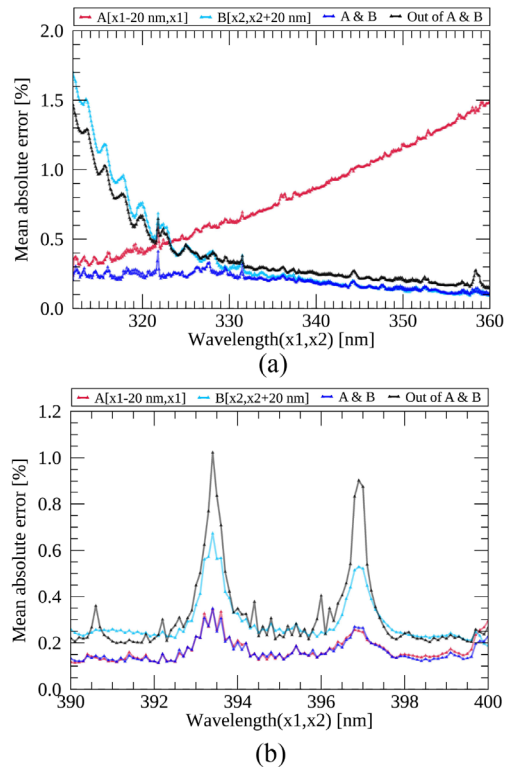
Figure 14 Mean absolute errors between the reproduced and measured radiances at (a) ozone absorption and (b) Fraunhofer lines with different input cases. The x_1 and x_2 in the legend indicate the wavelengths at the boundary of output spectral bands, respectively. The absolute error is calculated between the ML and GEMS radiances divided by the latter in percent.
