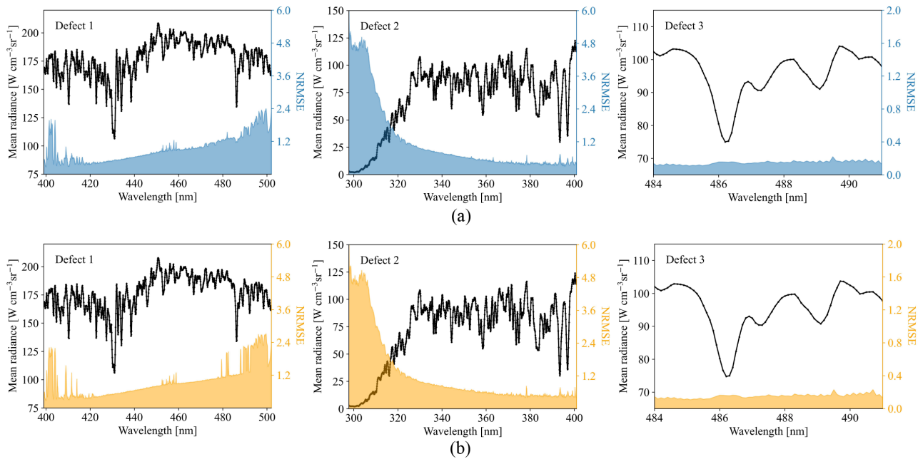
205 Figure 6 Output radiances for Defect 1-3 with the average and NRMSE for (a) training and (b) test datasets measured in March 2021. The unit of NRMSE is in percent.
