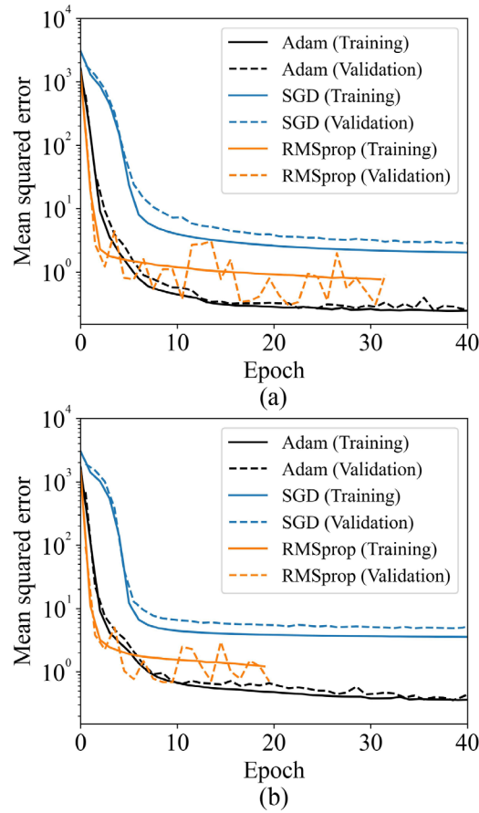
Figure 4 Training and validation losses for Defect 2 (a) with and (b) without the angle conditions as input parameters with different optimizers such as Adam (black), SGD with the gradient clipping value of 0.5 (blue) and RMSprop (orange).
