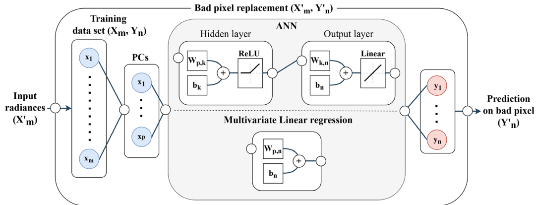
145 Figure 3 Schematic chart of the training and bad pixel replacement process. \mathbf{W} and \mathbf{b} represent weight and bias parameters in each layer. The subscripts m , n , p and k are equal to the spectral dimension of input and output parameters, the number of PCs and hidden nodes of the ANN model, respectively.
