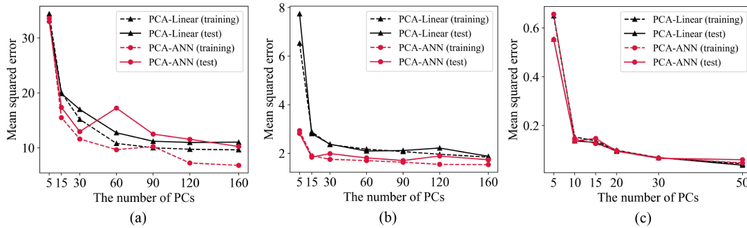
Figure 5 Loss function with the different number of PCs of the PCA-ANN (red) and PCA-Linear (black) models for spectral replacement with training and test datasets for Defects 1-3 ((a): Defect 1, (b): Defect 2 and (c): Defect 3). The number of hidden nodes for ANN is double the number of PCs.
