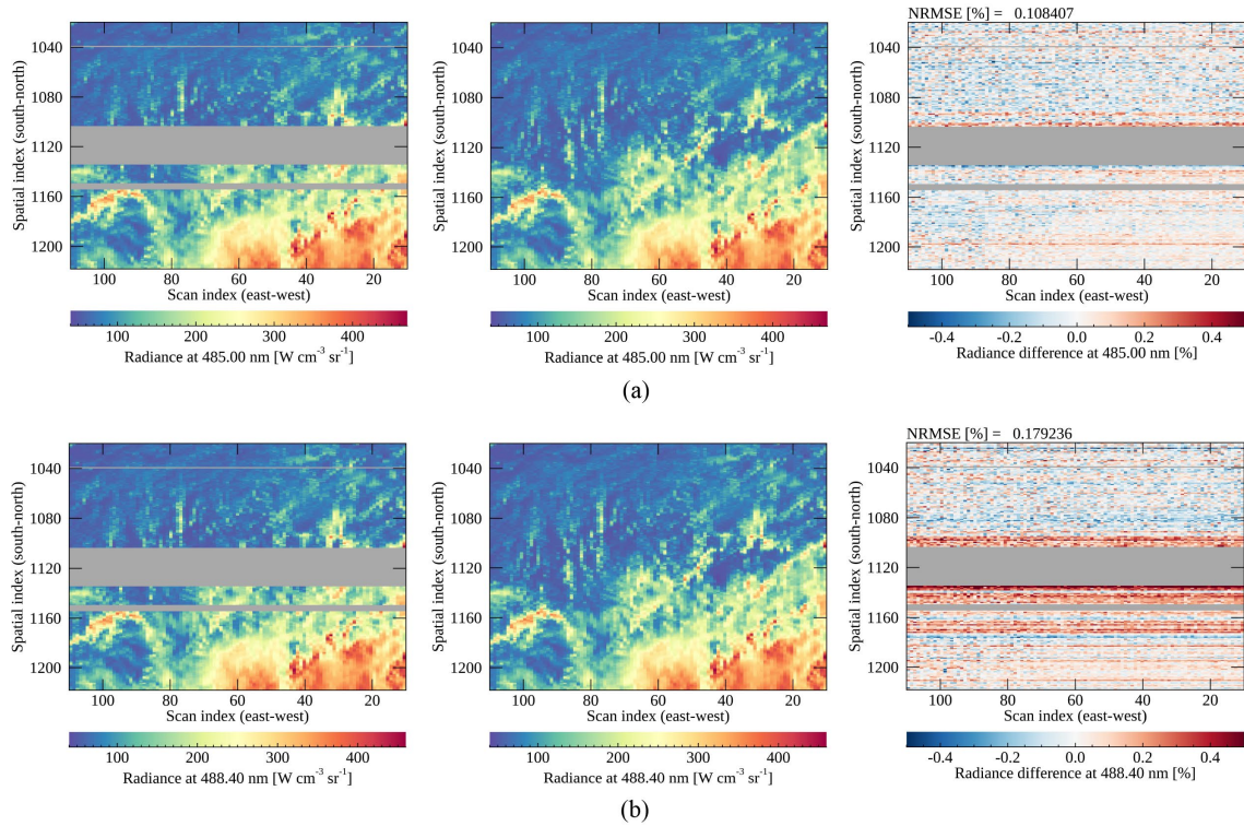
Figure 7 Spatial distribution of GEMS, ML radiances and the differences (from the first to the third column) at the wavelengths presenting (a) the smallest and (b) the largest differences for the Defect 3 area. The difference is calculated between the ML and GEMS radiances divided by the latter in percent. Bad pixels are marked in dark gray and the color bar range for differences is \pm 0.5\% . The unit of NRMSE is in percent divided by mean radiance.
