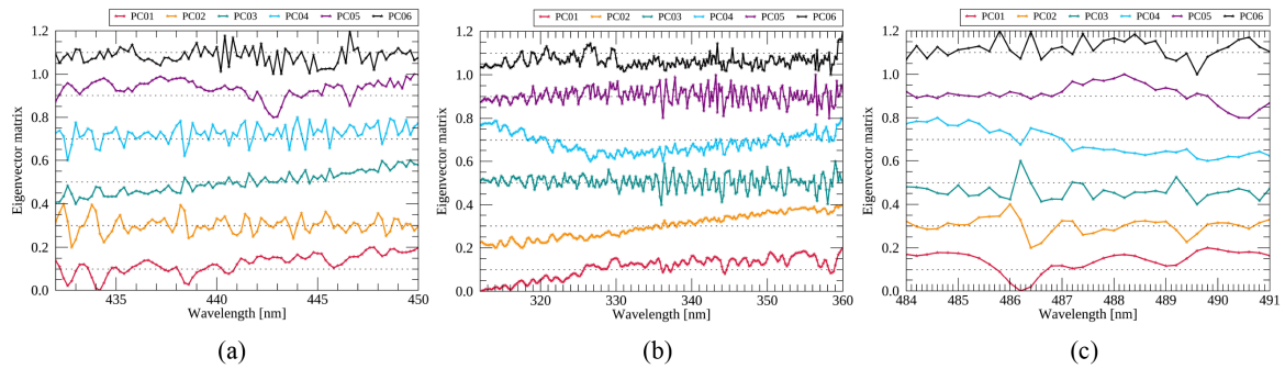
270 Figure 11 Eigenvector of the first-six PCs applied to GEMS radiances for the target wavelengths of (a) Defects 1, (b) Defect 2 and (c) Defect 3. All eigenvectors are scaled (min-max scaling) and shifted for clarity of presentation.
