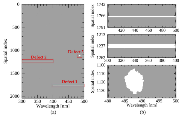
Figure 1 The two-dimensional bad pixel map (a) on the GEMS CCD detector along the spectral (x-axis) and spatial direction (y-axis) and (b) zooming in the bad pixel positions from top to bottom rows for Defects 1-3. Bad pixels are marked in white.
