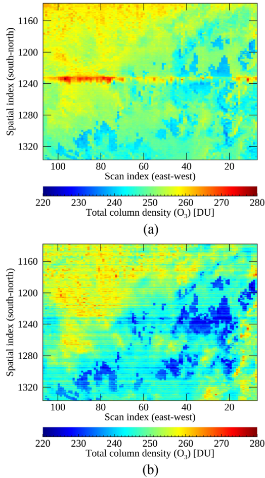
Figure 13 Spatial distribution of total ozone column density retrieved with (a) GEMS and (b) ML radiances presented in Fig.9. The GEMS spectra were measured on 10 March 2021 (06 UTC).
