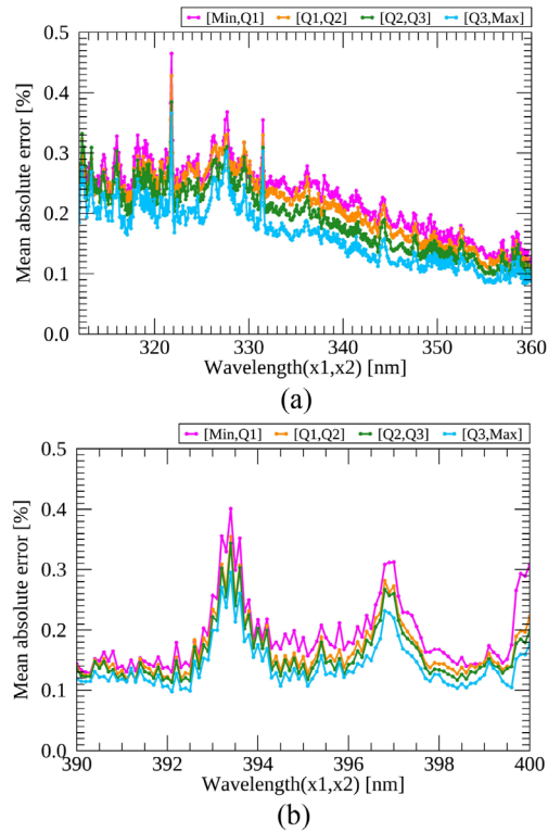
340 Figure 15 Mean absolute errors between the reproduced and measured radiances at (a) ozone absorption and (b) Fraunhofer lines with the input case showing the smallest errors in Fig. 14. The Q1, Q2 and Q3 represent the first, second and third quartile and each color indicates the average in the range of each quartile. The x1 and x2 indicates wavelengths at the boundary of output spectral bands and the absolute error is calculated between the ML and GEMS radiances divided by the latter in percent.
