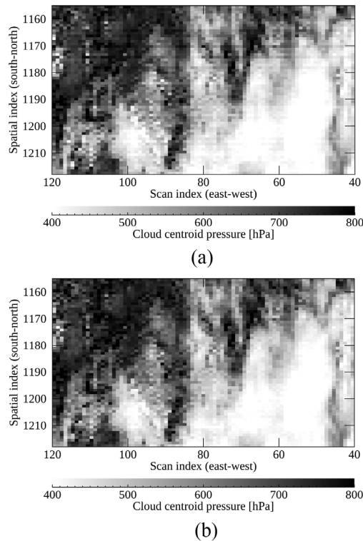
295 Figure 12 Spatial distribution of cloud centroid pressure retrieved with (a) GEMS and (b) ML radiances zooming in a certain area presented in Fig. 7. The GEMS spectra were measured on 10 March 2021 (06 UTC).
