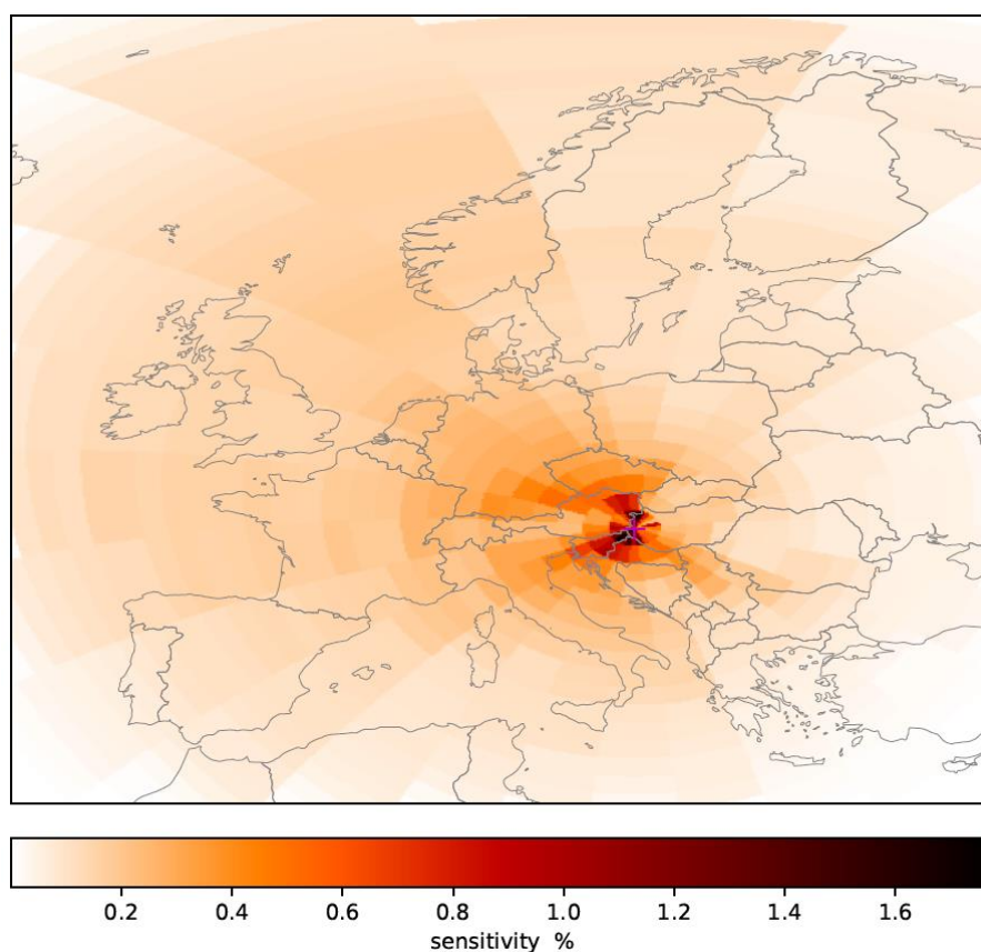
410 Figure 7: Footprint climatology of the concentration measurements performed at 115 m elevation above the ground in 2019 calculated by the STILT model (Carbon Portal, 2022).
