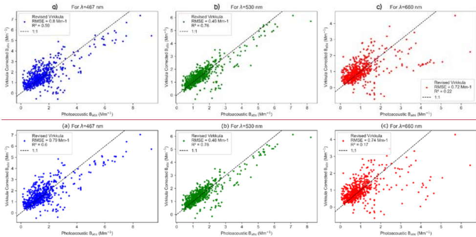
Figure 3: Comparison between PSAP absorption coefficients, corrected for using the Virkkula algorithm with revised coefficients, and the reference corresponding to (a) 467nm, (b) 530nm and (c) 660nm wavelengths.
