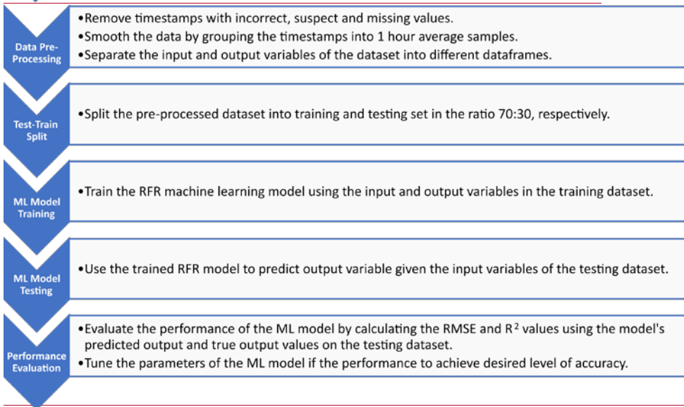
Figure A54: Workflow of Machine Learning based correction model developed and used in this study.
