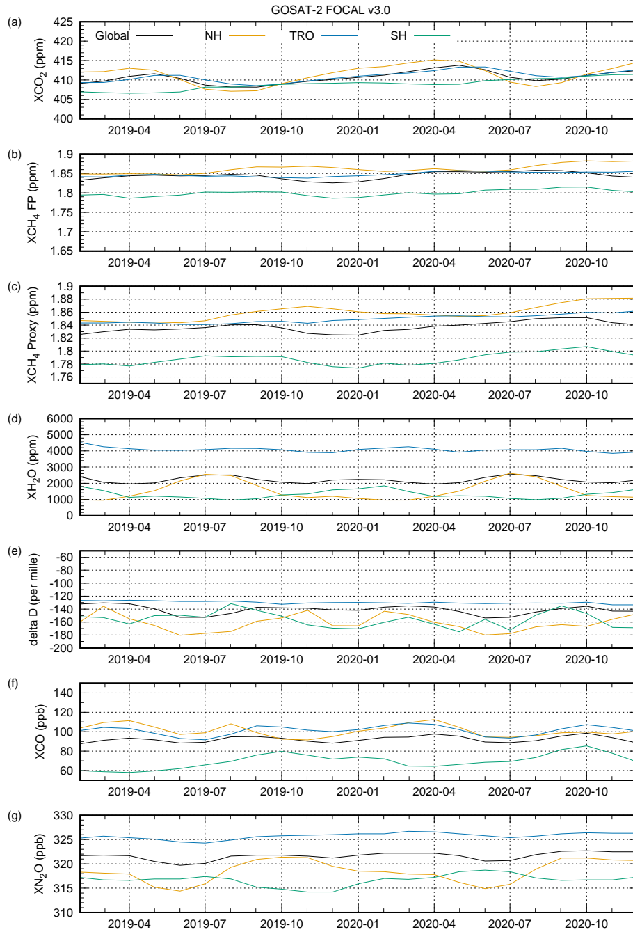
Figure 1 GOSAT-2 time series. NH = Northern hemisphere ( > 25^{\circ}\text{N} ). TRO = Tropics ( 25^{\circ}\text{S} - 25^{\circ}\text{N} ). SH = Southern hemisphere ( < 25^{\circ}\text{S} ). (a) \text{XCO}_2 . (b) \text{XCH}_4 full physics product. (c) \text{XCH}_4 proxy product. (d) \text{XH}_2\text{O} . (e) \delta\text{D} . (f) \text{XCO} . (g) \text{XN}_2\text{O} .
