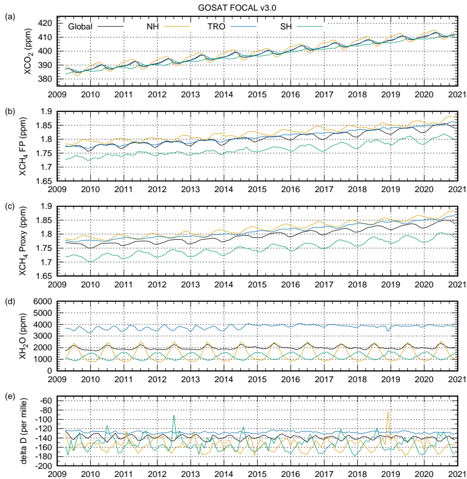
Figure 4. GOSAT time series. NH = Northern hemisphere ( > 25^\circ N ). TRO = Tropics ( 25^\circ S - 25^\circ N ). SH = Southern hemisphere ( < 25^\circ S ). (a) X_{CO_2} . (b) X_{CH_4} full physics product. (c) X_{CH_4} proxy product. (d) X_{H_2O} . (e) \delta D .
