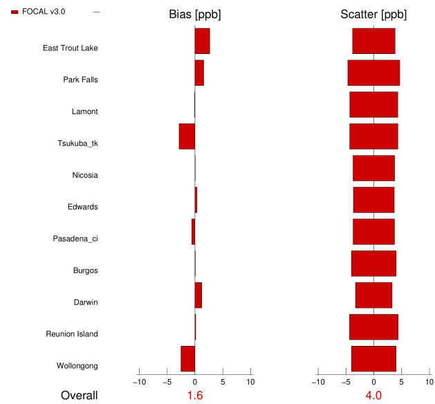
Figure 10. As Fig. 8, but for: (a) XCO. (b) XN 2 O.
