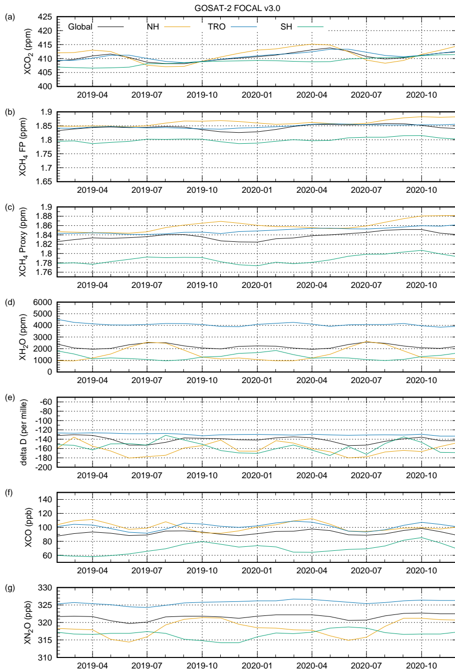
Figure 1 GOSAT-2 time series. NH = Northern hemisphere ( > 25^\circ N ). TRO = Tropics ( 25^\circ S - 25^\circ N ). SH = Southern hemisphere ( < 25^\circ S ). (a) XCO_2 . (b) XCH_4 full physics product. (c) XCH_4 proxy product. (d) XH_2O . (e) \delta D . (f) XCO . (g) XN_2O .
