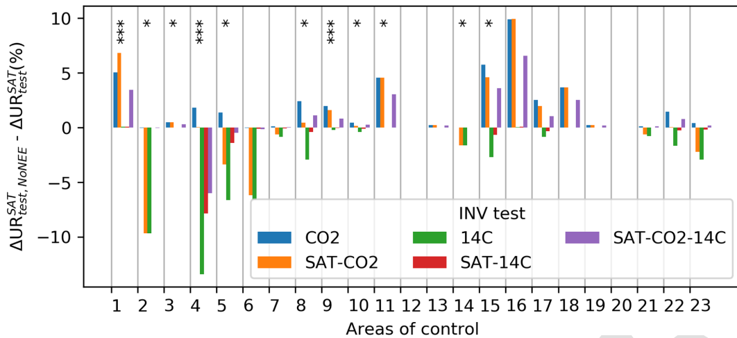
Figure 13. Impact of the NEE on the ground network capability at the top of the satellite observations for each area of control in the main area of interest: differences between \Delta UR_{test}^{SAT} on 24 h FF regional budgets, with and without NEE. Negative values highlight an increase in the additional observation network potential when NEE is taken into account. Positive values highlight a decrease in the additional observation network potential when NEE is taken into account. High absolute values highlight strong NEE impact. The number of stars indicates the number of stations in each controlled area. The areas are listed in Table 1.
