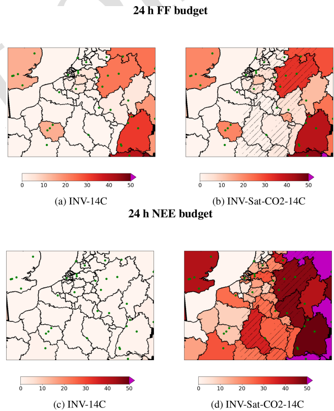
Figure 14. Uncertainty reduction in INV-14C (a, c) and INV-Sat-CO2-14C (b, d) inversions: for 24 h budgets of FF emissions (a, b) and biogenic fluxes (NEE, c, d). Stripes are indicative of the satellite field of view (see Fig. 6 for the full track). Green dots indicate the ground stations.
