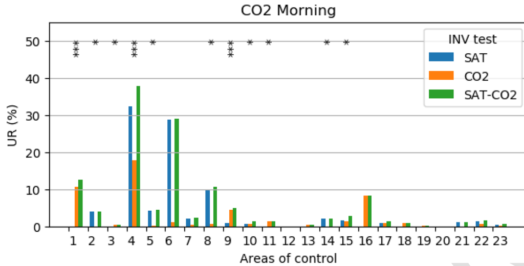
Figure A3. Uncertainty reduction in INV-SAT, INV-CO 2 , and INV-SAT-CO 2 inversions for morning budgets of FF emissions of each controlled area in the main area of interest. The number of stars indicates the number of stations in each controlled area. The controlled areas are listed in Table 1.
