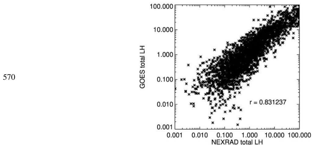
Figure 7: Scatter plot of NEXRAD total LH and GOES total LH in K/s. It is plotted in log-log axes.
