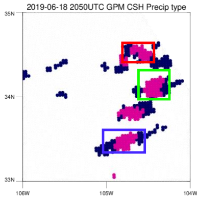
Figure 3: A scene on 18 June 2019. (a) NEXRAD composite reflectivity. Only the regions with reflectivity greater than 28dBZ are shown in colors. Color bar is in dBZ. (b) Convective regions detected by GOES-16 are colored in pink on top of GOES-16 visible image at channel 2 (0.65 \mu m). (c) Precipitation type defined by CSH. Convective regions are colored in pink while stratiform regions are colored in navy.
