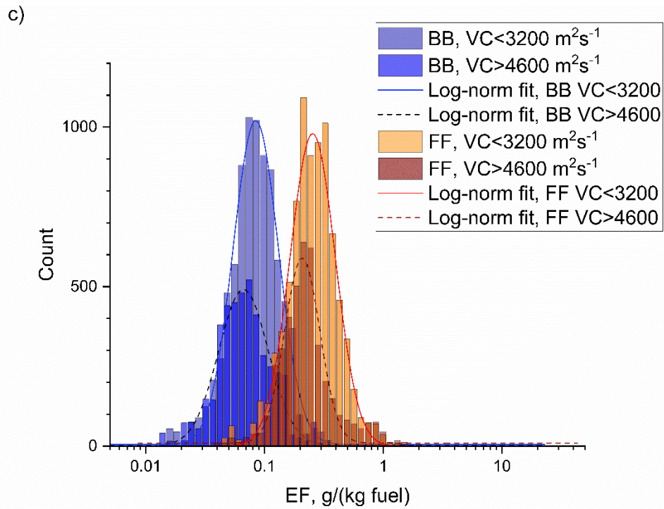
Figure 6. FF (brown bars) and BB (blue bars) related emission factors at a) BTC, b) SKY and c) TRO locations respectively. Low ( VC < 3200 \text{ m}^2\text{s}^{-1} ) and high ventilation cases ( VC > 4600 \text{ m}^2\text{s}^{-1} ) were plotted separately. Lognormal distributions (solid and dashed lines) were fitted to the results: the parameters are summarised in Table 3.
