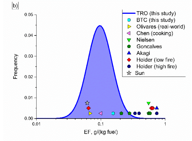
Figure 8. Distribution of the transformed FF EFs referring the diesel emission at the BTC location (a). Scatter points show average EF data from the literature and the highway measurement (only X-axis concerned). b) Distribution of the BB EFs at the TRO location.
