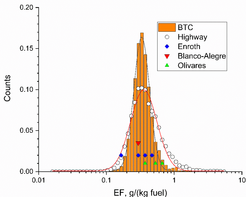
Figure 7. Distributions of the emission factors originated from traffic at BTC (all data) and the highway. Log-normal functions were fitted on the points with parameters summarised in Table 5. Coloured scatter symbols refer the literature data (only X-axes concerned). See more details in Table 6.
