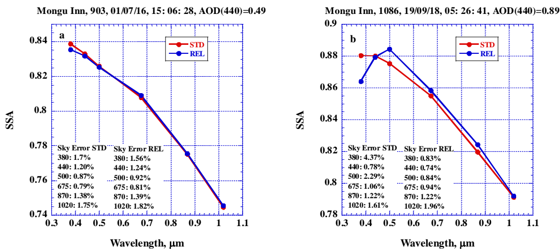
655 Figure 2. SSA retrieved using V3 assumptions on the IPRI smoothness constants (STD) and that of relaxed (REL) at Mongu Inn AERONET site: a) AOD(440)=0.49, AE=1.85 and b) AOD(440)=0.89, AE=1.97.
