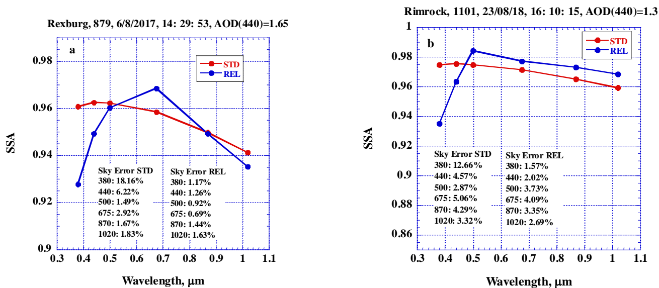
Figure 1. SSA retrieved using V3 assumptions on the IPRI smoothness constants (STD) and that of relaxed (REL): a) Rexburg (AOD(440)=1.65, AE=1.74) and b) Rimrock (AOD(440)=1.33, AE=1.79) AERONET sites.
