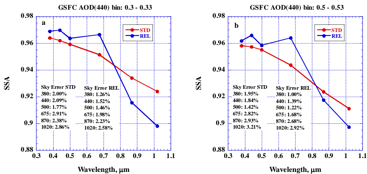
Figure 8. SSA averaged over AOD(440) bins for GSFC AERONET site: a) 0.3-0.33 and b) 0.5-0.53.
