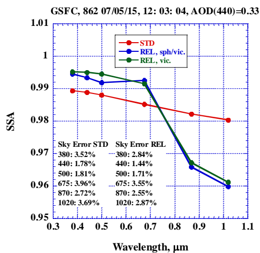
Figure 9. Same as Figure 7a with addition of SSA retrieved from vicariously calibrated sky radiances, depicted by REL, vic. Abbreviation REL, sph./vic. refers to SSA retrieved by inverting sky radiances calibrated using integrated sphere at all the channels except 380 nm which was calibrated using vicarious method.
