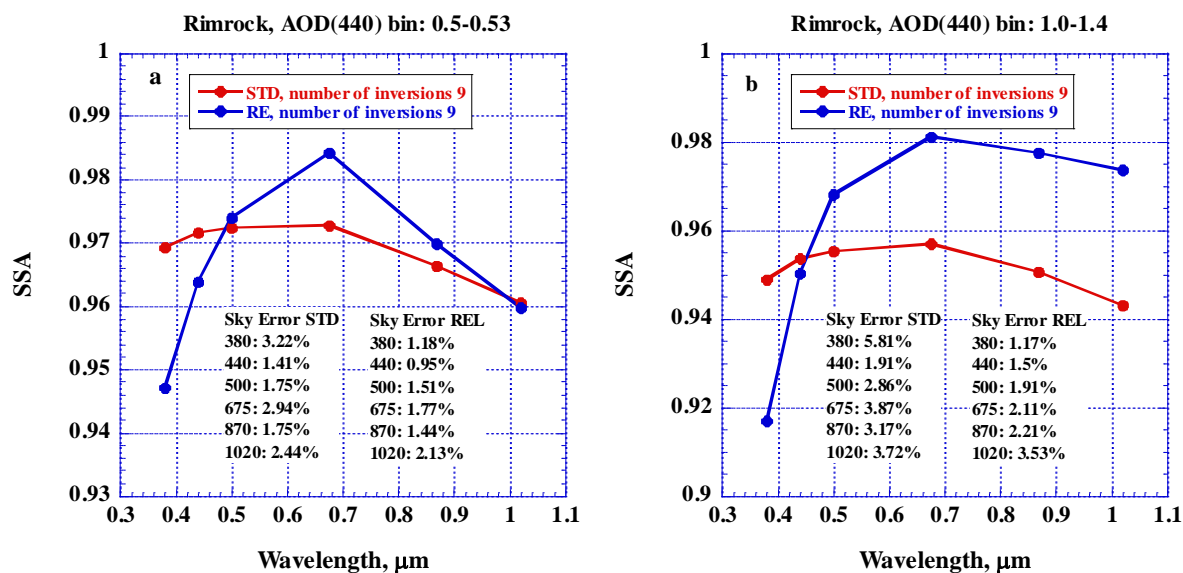
700 Figure 4. SSA averaged over AOD(440) bins for Rimrock AERONET site: a) 0.5-0.53 and b) 1.0-1.4
