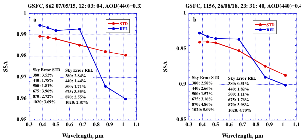
765 Figure 7. SSA retrieved using V3 assumptions, depicted as STD, and that of REL on the IPRI smoothness constants at GSFC AERONET site: a) AOD(440)=0.33, AE=1.74 and b) AOD(440)=0.49, AE=1.63.
