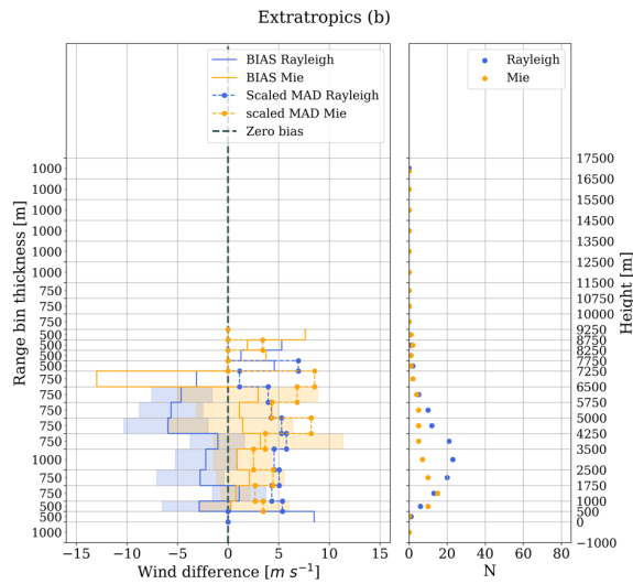
Figure 6. Wind differences (Aeolus-WPR) with range bins for (a) tropics and (b) extratropics. Left: distributions of BIAS and scaled MAD of wind differences over different range bins with shading areas representing the uncertainty. Right: the number of available match-ups at each range bin. Blue and orange colours indicate the results for the Rayleigh and Mie channels, respectively. Note: the heights on y-axis are just for reference, which are not exactly same with the actual heights of each vertical range bin.
