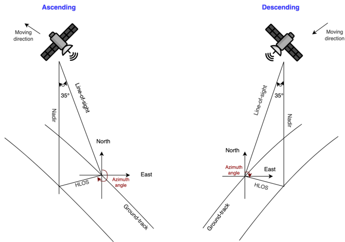
Figure 2. Geometry of Aeolus wind measurements.
