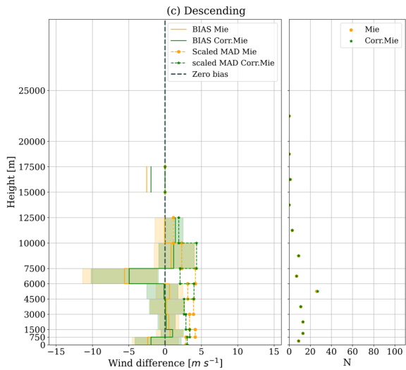
Figure A2. Wind differences (Aeolus-WPR) with height for (a) all data, (b) ascending orbits and (c) descending orbits. Left: BIAS and scaled MAD of wind differences as a function of height with shading areas representing the uncertainty. Right: the number of available match-ups at each height. Orange and green colours indicate the results for Mie-cloudy and corrected Mie-cloudy winds, respectively.
