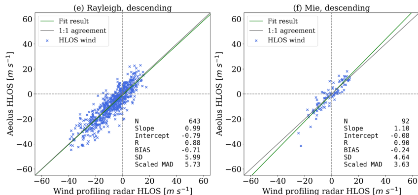
Figure 4. Scatter plots of Aeolus HLOS winds against WPR HLOS winds for all data, ascending orbits and descending orbits. Plot (a), (c) and (e) are for the Rayleigh-clear winds, and (b), (d) and (f) are for the Mie-cloudy winds. Green and grey lines indicate the fitted regression result and 1:1 agreement, respectively.
