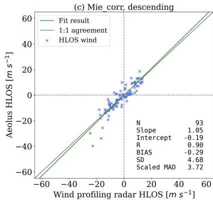
630 Figure A1. Scatter plots of corrected Mie-cloudy winds against WPR HLOS winds for all data (a), ascending orbits (b) and descending orbits (c). Green and grey lines indicate the fitted regression result and 1:1 agreement, respectively. Regarding the wind difference as a function of height (Fig. A2), some improvements in accuracy and precision can be found mainly below 10,000 m. In particular, for data from all orbits, the random error below 3,000 m reduced by at least 0.6 m s -1 ; the biases between 1,500 m and 6,000 m during descending orbits are close to 0. The reduction in random error can also be seen below 4,000 m and between 6,000 m and 8,000 m in tropics; the reduction in both biases and random errors can be found 635 from 1,750 m to 3,500 m and from 4,250 m to 5,000 m in extratropics (Fig. A3). These are in line with the fact that most of the corrected Mie winds are from moderate wind speed range.
