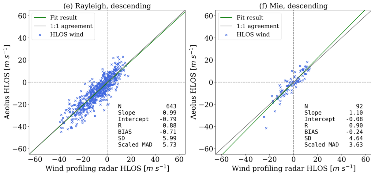
270 Figure 4. Scatter plots of Aeolus HLOS winds against WPR HLOS winds for all data, ascending orbits and descending orbits. Plot (a), (c) and (e) are for the Rayleigh-clear winds, and (b), (d) and (f) are for the Mie-cloudy winds. Green and grey lines indicate the fitted regression result and 1:1 agreement, respectively.
