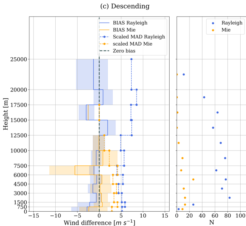
Figure 5. Wind differences (Aeolus-WPR) with height for (a) all data, (b) ascending orbits and (c) descending orbits. Left: BIAS and scaled MAD of wind differences as a function of height with shading areas representing the uncertainty. Right: the number of available match-ups at each height. Blue and orange colours indicate the results for the Rayleigh and Mie channels, respectively.
