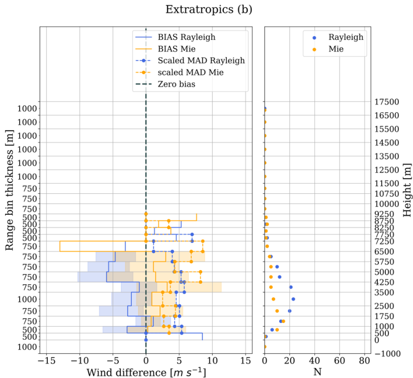
305 Figure 6. Wind differences (Aeolus-WPR) with range bins for (a) tropics and (b) extratropics. Left: distributions of BIAS and scaled MAD of wind differences over different range bins with shading areas representing the uncertainty. Right: the number of available match-ups at each range bin. Blue and orange colours indicate the results for the Rayleigh and Mie channels, respectively. Note: the heights on y-axis are just for reference, which are not exactly the same with the actual heights of each vertical range bin.
