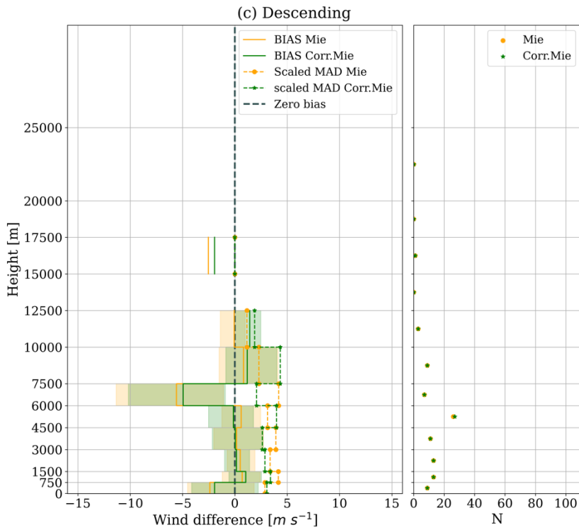
465 Figure A2. Wind differences (Aeolus-WPR) with height for (a) all data, (b) ascending orbits and (c) descending orbits. Left: BIAS and scaled MAD of wind differences as a function of height with shading areas representing the uncertainty. Right: the number of available match-ups at each height. Orange and green colours indicate the results for Mie-cloudy and corrected Mie-cloudy winds, respectively.
