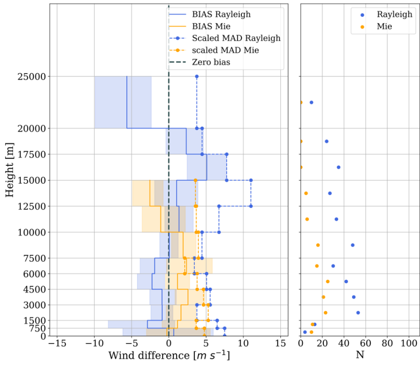
(b) Ascending
