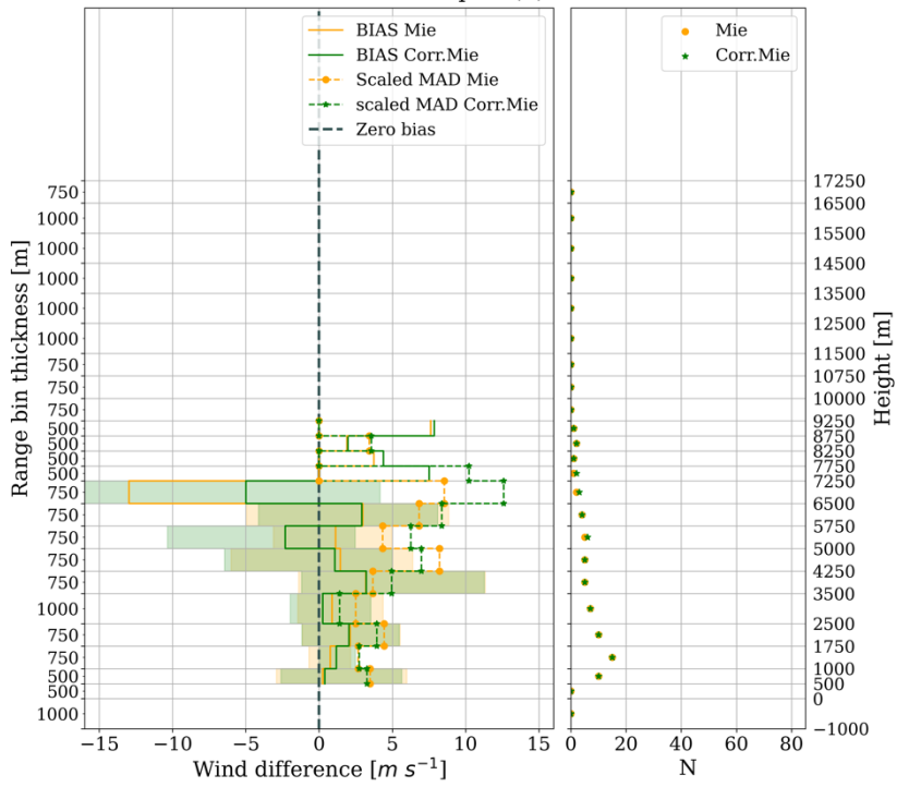
Extratropics (b)
