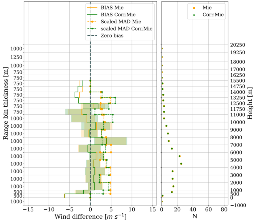
Extratropics (b)
