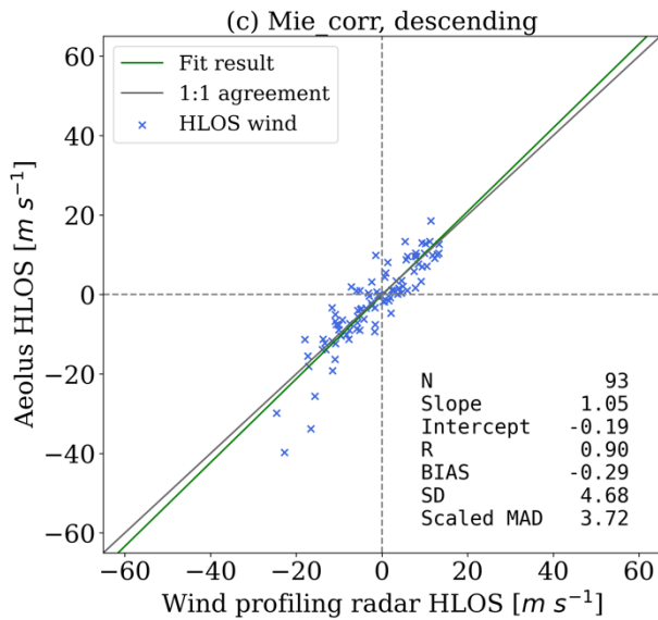
Figure A1. Scatter plots of corrected Mie-cloudy winds against WPR HLOS winds for all data (a), ascending orbits (b) and descending orbits (c). Green and grey lines indicate the fitted regression result and 1:1 agreement, respectively.
