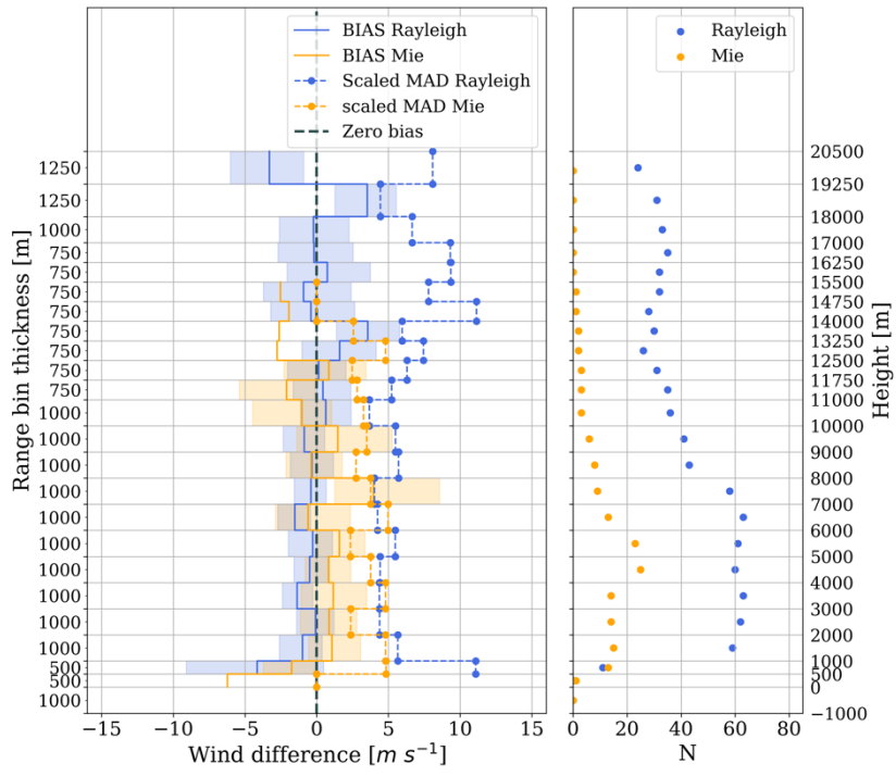
Tropics (a)
