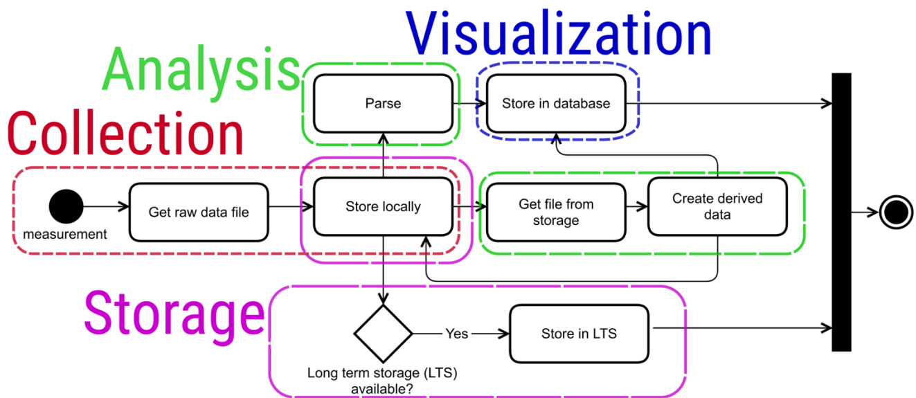
Figure 1. Workflow of processing of a raw file of time series data and creating derived data products from it. The datafile is collected, parsed and stored, then various further processing can be done to it to create derived data. The different colored hashed boxes show which implementation part of SMEARcore is involved in each processing step. The implementation parts are explained in Section 3. The black bordered boxes are steps in the workflow. The black dot on the right of the figure marks the end of the workflow.
