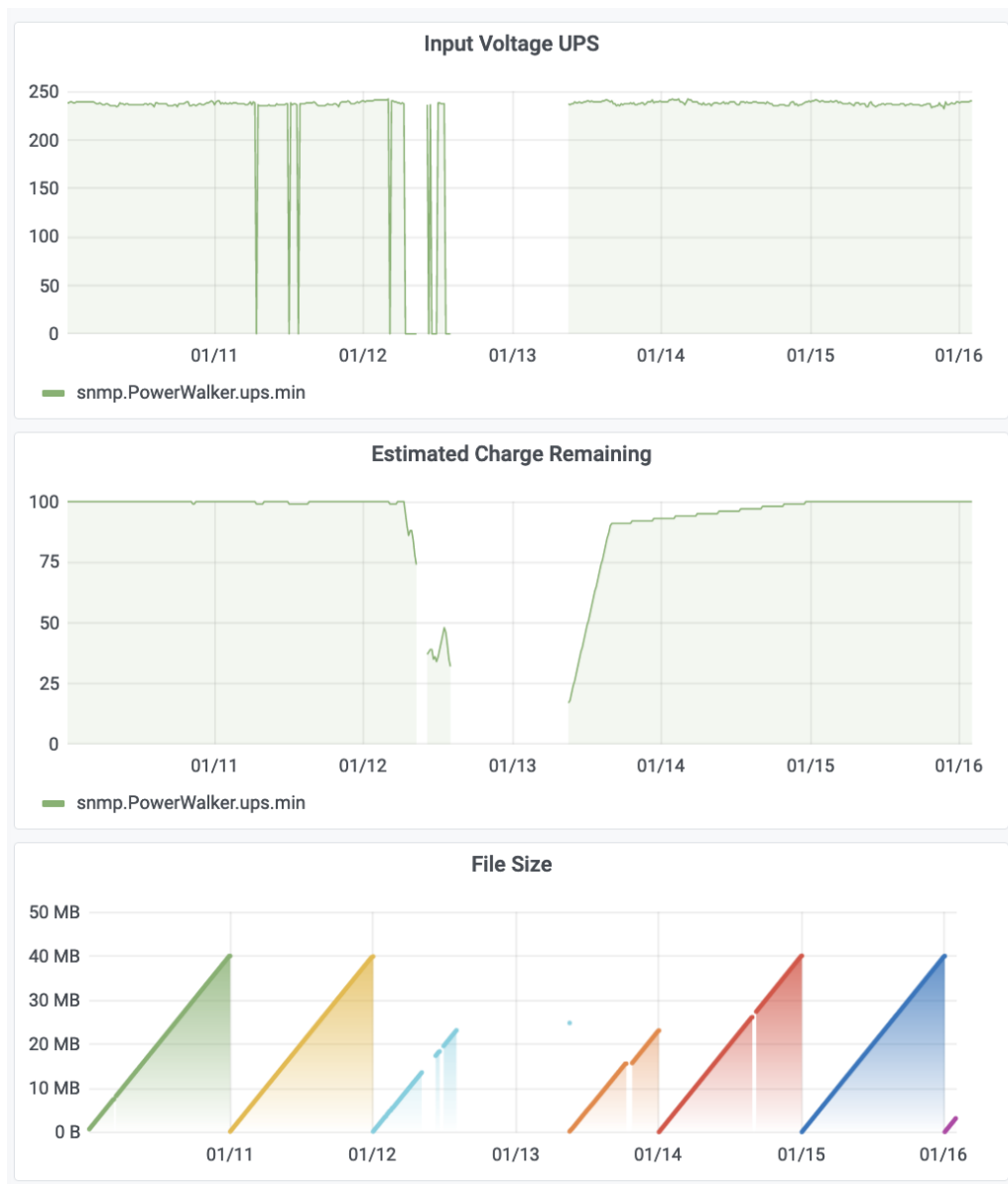
335 Figure 9. Effects of a long power cut on data collection at the SMEAR Estonia station on 10.-15.1.2021. UPS is fully discharged, and the station experienced network related issues due to no power. The observed data file size is considerably smaller due to missing data, and this is easily diagnosed from the collected metadata.
