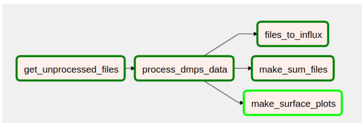
Figure 10. The DMPS processing graph as seen from Airflow. It follows the same structure as the workflow in Figure 2. Influx refers to the database used for storing the processed data. Sum files are the processed file type and surface plots are used for visualization. The arrows represent dependencies, and the last three tasks can be done in parallel. All files are stored in a s3 instance. Colors represent the status of the task. In this case everything but make_surface_plots has completed successfully, while that task is still running.
