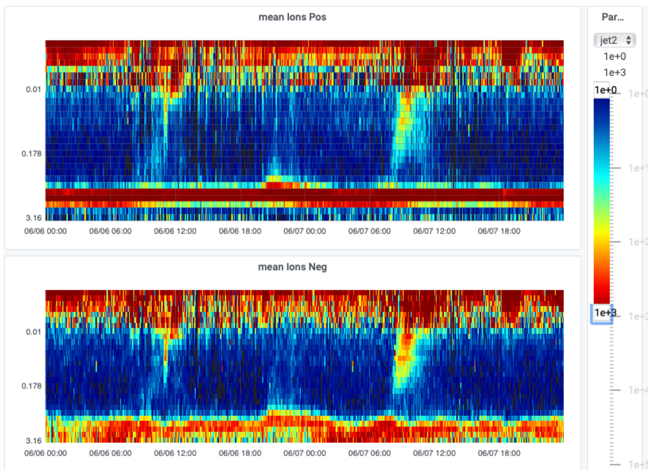
Figure 3. On-line visualization of number size-distribution of positive (top) and negative (bottom) air ions measured with Neutral cluster and Air Ion Spectrometer (NAIS) at Järvelja SMEAR station on 6-7 th of June 2021. Visualization is done with a custom plugin developed at the SMEAR station. The colormap and the number concentration scale can be changed by the user for their preferred viewing experience. The y-axis displays in logarithmic scale the ion mobility in units (sV/cm 2 ). Colorscale indicates the number concentration (dN/dlog 10 (dp), cm -3 ).
