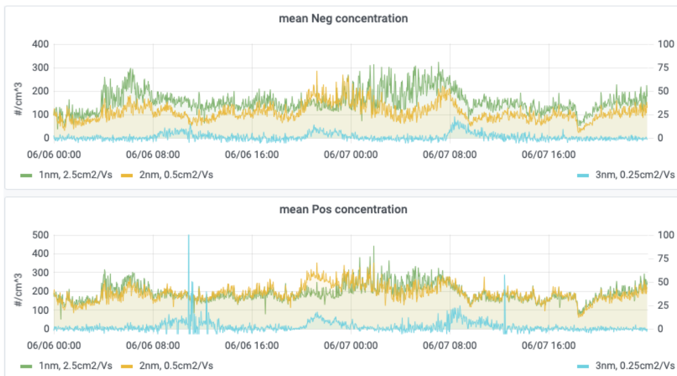
285 Figure 4. Concentrations of atmospheric ions with geometric mean diameter of collection electrodes of 1 nm (green line) and 2 nm (yellow line) cluster ions, and 3 nm (cyan line) intermediate ions measured at the Järvelja SMEAR station during 6.6.2021 - 7.6.2021 measured by the Cluster Ion Counter (CIC). Due to the instrument design, the measured concentrations include ions from a wide mobility range. Negative ions are shown in the top panel and positive ions in the bottom panel.
