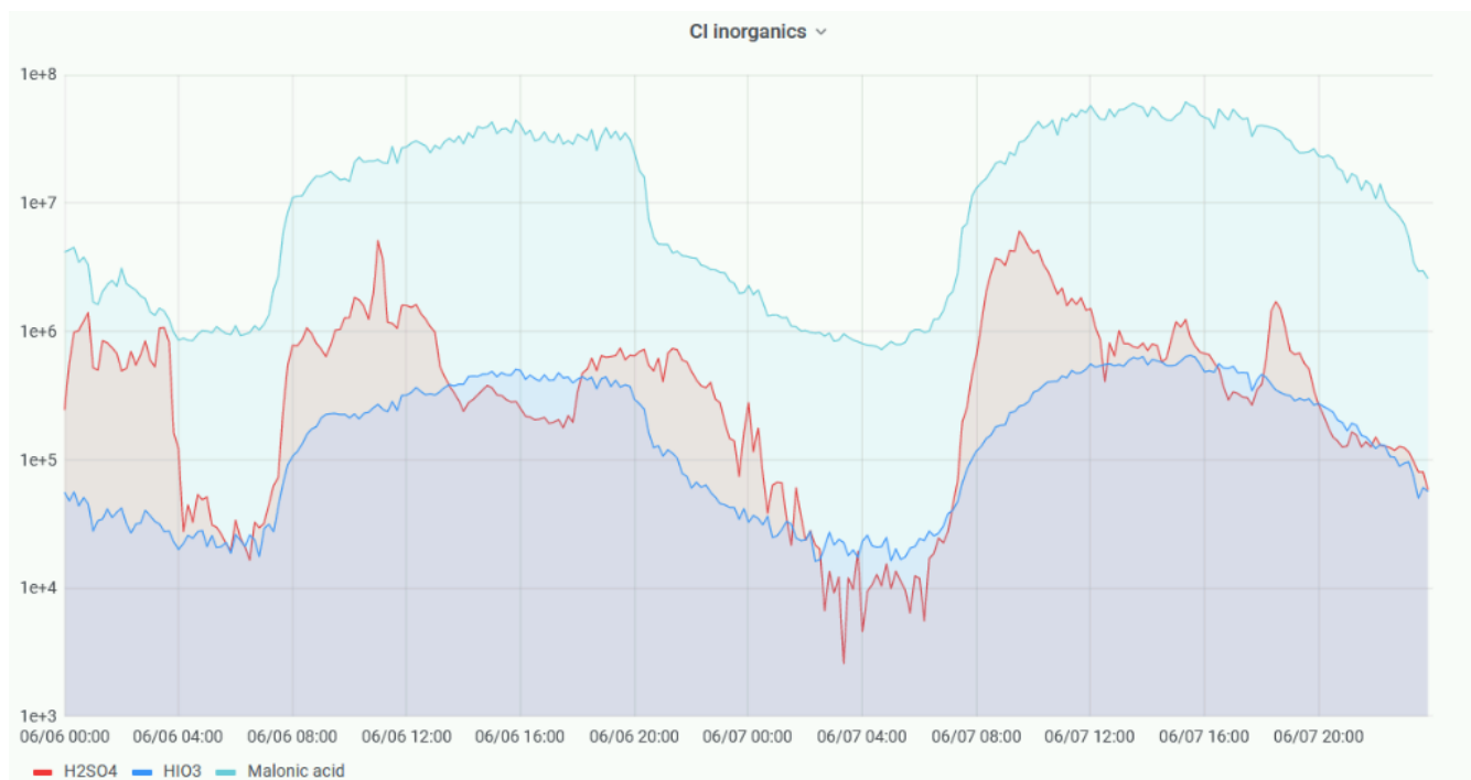
295 Figure 6. CI-API-TOF on-line inorganic acid concentrations (sulphuric acid shown in red, iodic acid in blue and malonic acid in cyan) measured at the SMEAR Estonia station during 6.6.2021- 7.6.2021. The formation of all three acids is initiated by solar radiation and formation of OH-radicals, however the precursor gases are different, SO 2 , I 2 , and a wide variety of volatile organic compounds, respectively.
