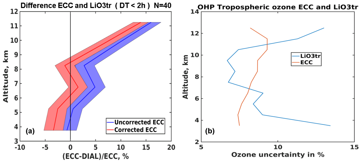
Figure 5. (a) Mean relative ECC - LiO3Tr ozone concentration differences in % between 3 and 12 km for uncorrected (blue) and homogenized (red) ozonesonde. Shaded areas represent the error for statistical standard uncertainty on the mean difference. (b) Vertical profiles of the median of the relative ozone concentration error for the homogenized ECC (red) and LiO3Tr (blue).
