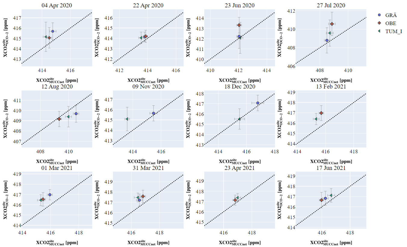
Figure A1. Daily X_{CO_2} by-site comparison results.
