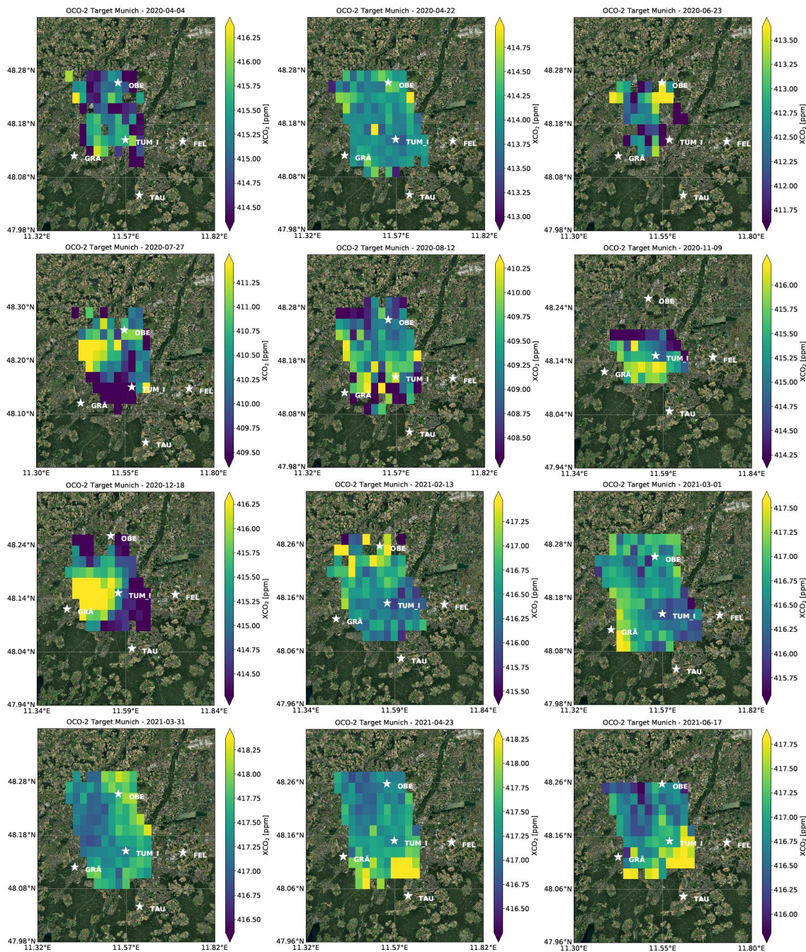
Figure 3. Number Daily XCO 2 maps of soundings for each of the OCO-2 target overpasses observations in Munich. On most days days OCO-2 captured more than 1000 non-flagged ( qf = 0 ) soundings per overpass. MUCCNnet spectrometer locations are highlighted on the map. Usually a higher number of good quality soundings corresponds with more robust and less sparse data. Thus Map Source: Esri , we remove overpasses with less than 500 good quality soundings. Maxar, Earthstar Geographics, and the GIS User Community
