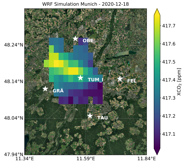
(b) Gridded X_{CO_2} at 12:00 UTC - 2 minutes before the OCO-2 overpass.
