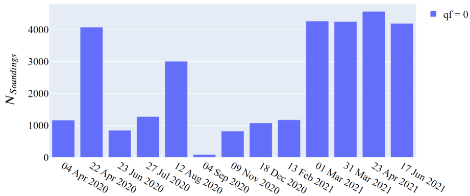
Figure 2. Daily heatmaps Number of soundings for each of the OCO-2 target X_{CO_2} in Munich overpasses. MUCCnet spectrometer locations are highlighted on the map On most days OCO-2 captured more than 1000 good quality ( qf = 0 ) soundings per overpass. Usually a higher number of good quality soundings corresponds with more robust and less sparse data. Thus, we remove overpasses with less than 500 good quality soundings.
