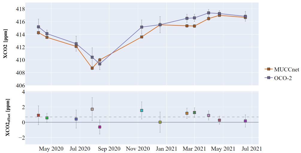
Figure 8. Both observing systems detect the seasonal X_{CO_2} variations and a X_{CO_2} growth in the study period. The lower panel shows the daily X_{CO_2} differences of satellite data and MUCCnet observations. The space-borne observations are biased high by 0.7 ppm.
