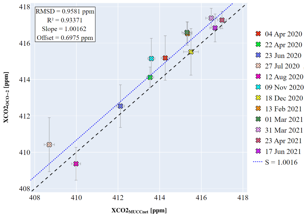
Figure 7. Scatter plot of MUCCNnet and OCO-2 X_{\text{CO}_2} in the comparison time frame. Each overpass is color-coded. The error bars represent the standard deviations of the samples in the corresponding domain.
