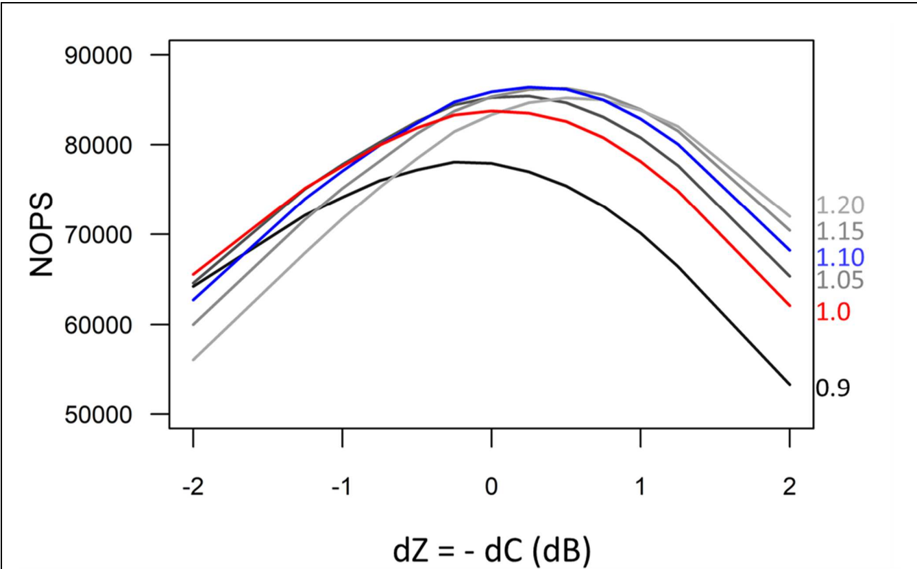
Figure 9: Evolution of the total number of optimal parameter sets (NOPS) computed for the three convective events all together as a function of dZ for various values of the exponent of the A - K_{dp} relationship listed on the right-hand side of the figure. Like in Figs. 4b and 7, the red curve corresponds to b_{AK} = 1.0 and the blue curve to b_{AK} = 1.1 .
