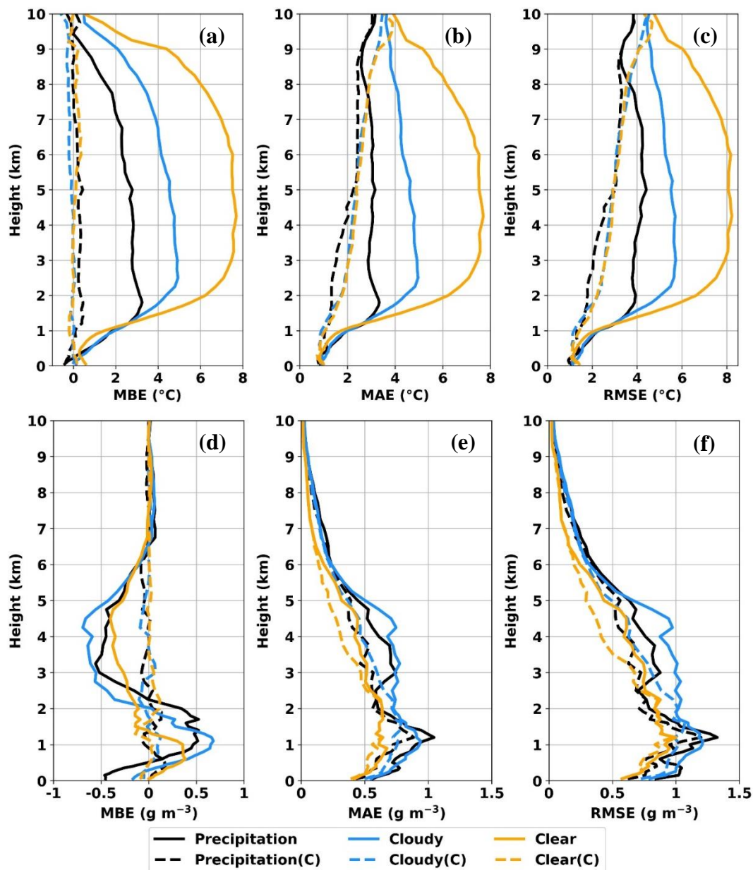
520 Figure 11. Vertical profiles of MBE, MAE and RMSE for original and corrected (C) MWR measured (a – c) temperature and (d – f) water vapor density during three weather conditions from the NYSM Profiler site at Albany.
