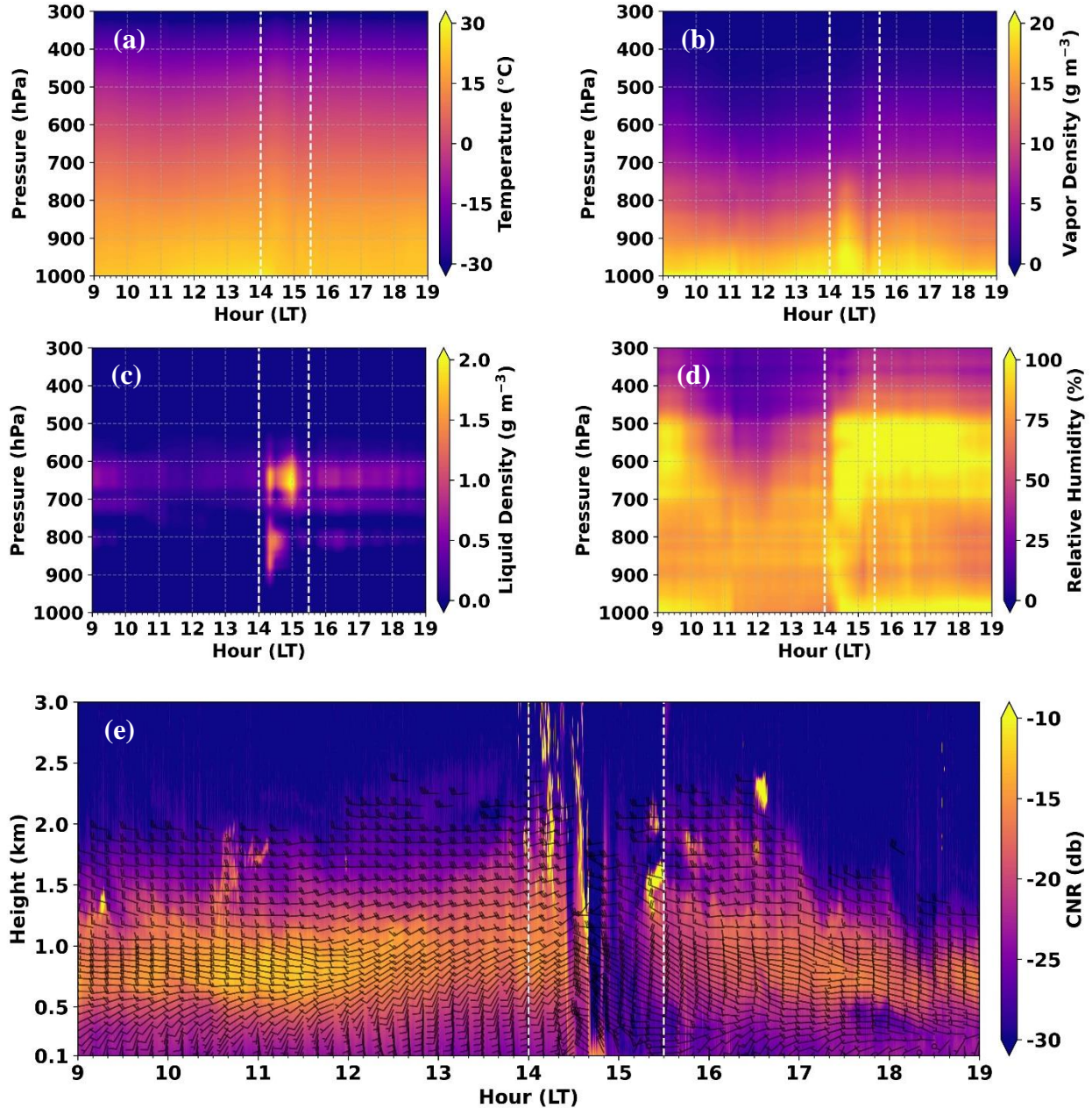
Figure 12. The MWR measured time-height cross section plots for (a) temperature (°C), (b) vapor density ( \text{g m}^{-3} ), (c) liquid density ( \text{g m}^{-3} ), (d) relative humidity (%) and (e) DL measured CNR (dB) with 10 minutes averaged wind barbs at Albany on 12 August 2021. Dotted box represents thunderstorm episode.
