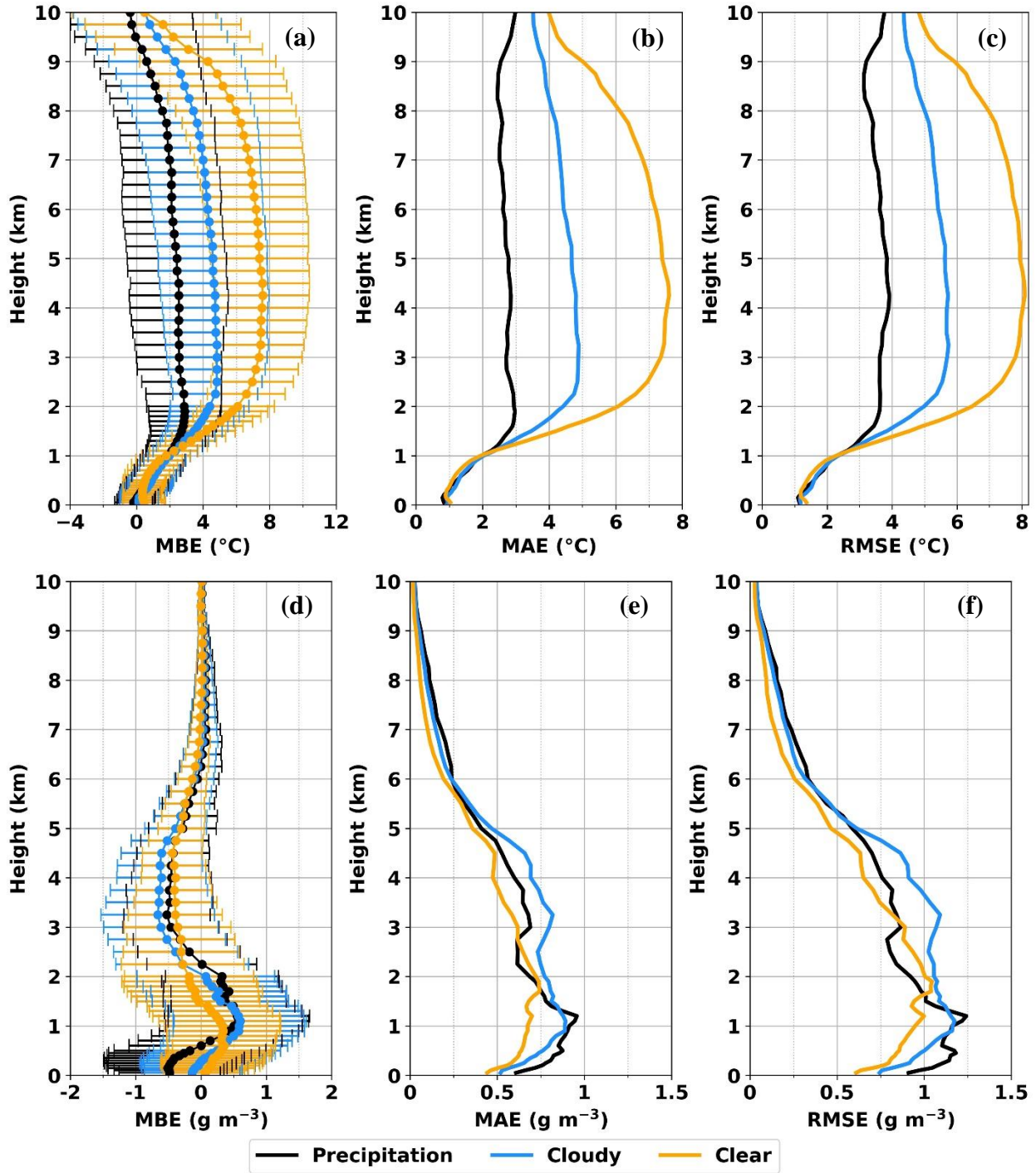
Figure 10. Vertical profiles of MBE with one standard deviation error bars, MAE and RMSE for (a – c) temperature and (d – f) water vapor density during three weather conditions from the NYSM
