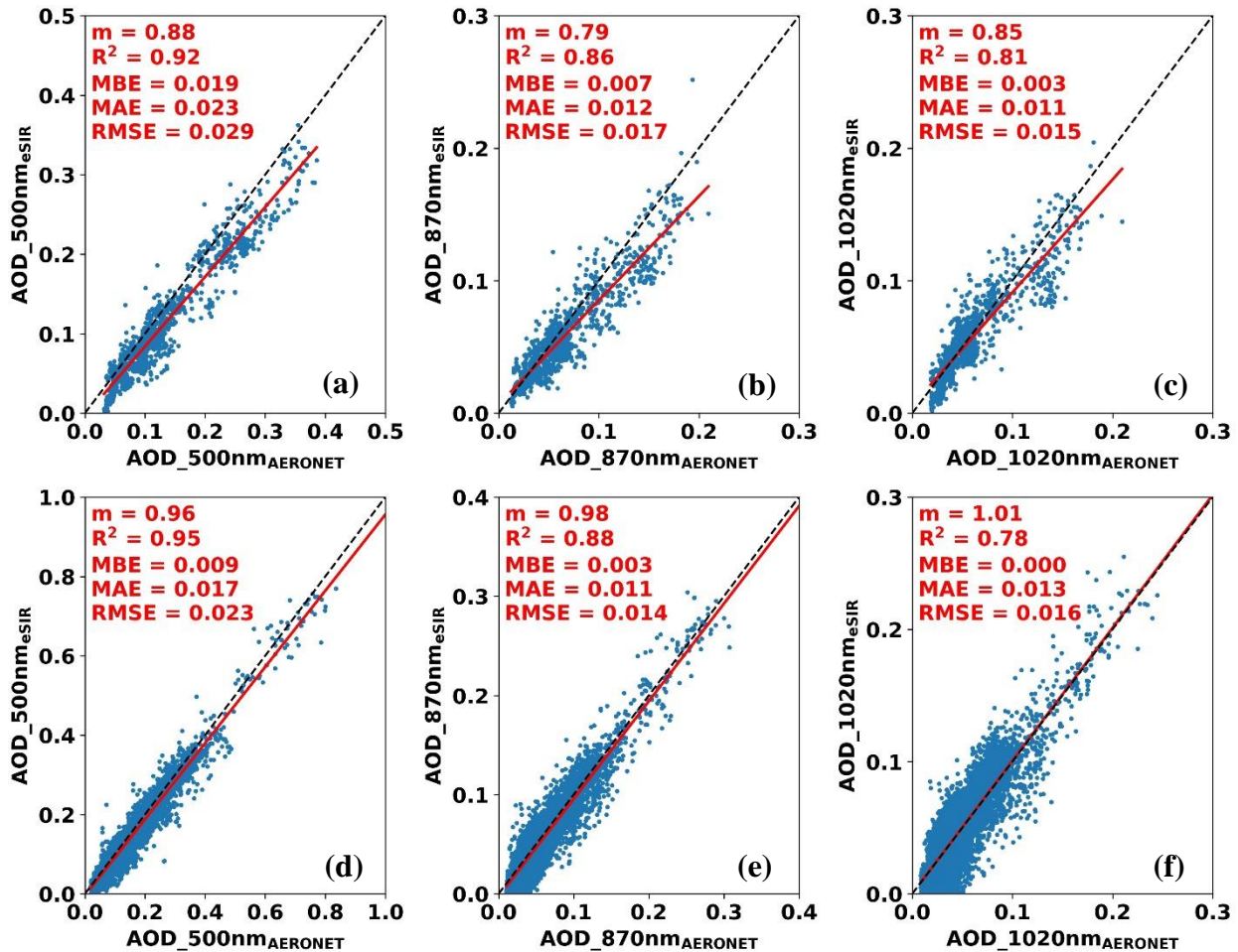
620 Figure 14. Scatterplots for the eSIR and Aeronet derived AOD for three channels: 500 nm, 870 nm, and 1020 nm at (a – c) Stony Brook and (d – f) Bronx.
