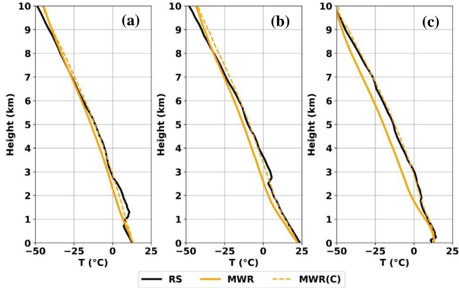
Figure 7. Vertical profiles of temperature (T) measured by RS and MWR – Original and Corrected (C) at (a) 23 UTC on 2 May (precipitation day), (b) 23 UTC on 28 July (cloudy day), (c) 11 UTC 370 on 2 May 2021 (clear sky day) at Albany.
