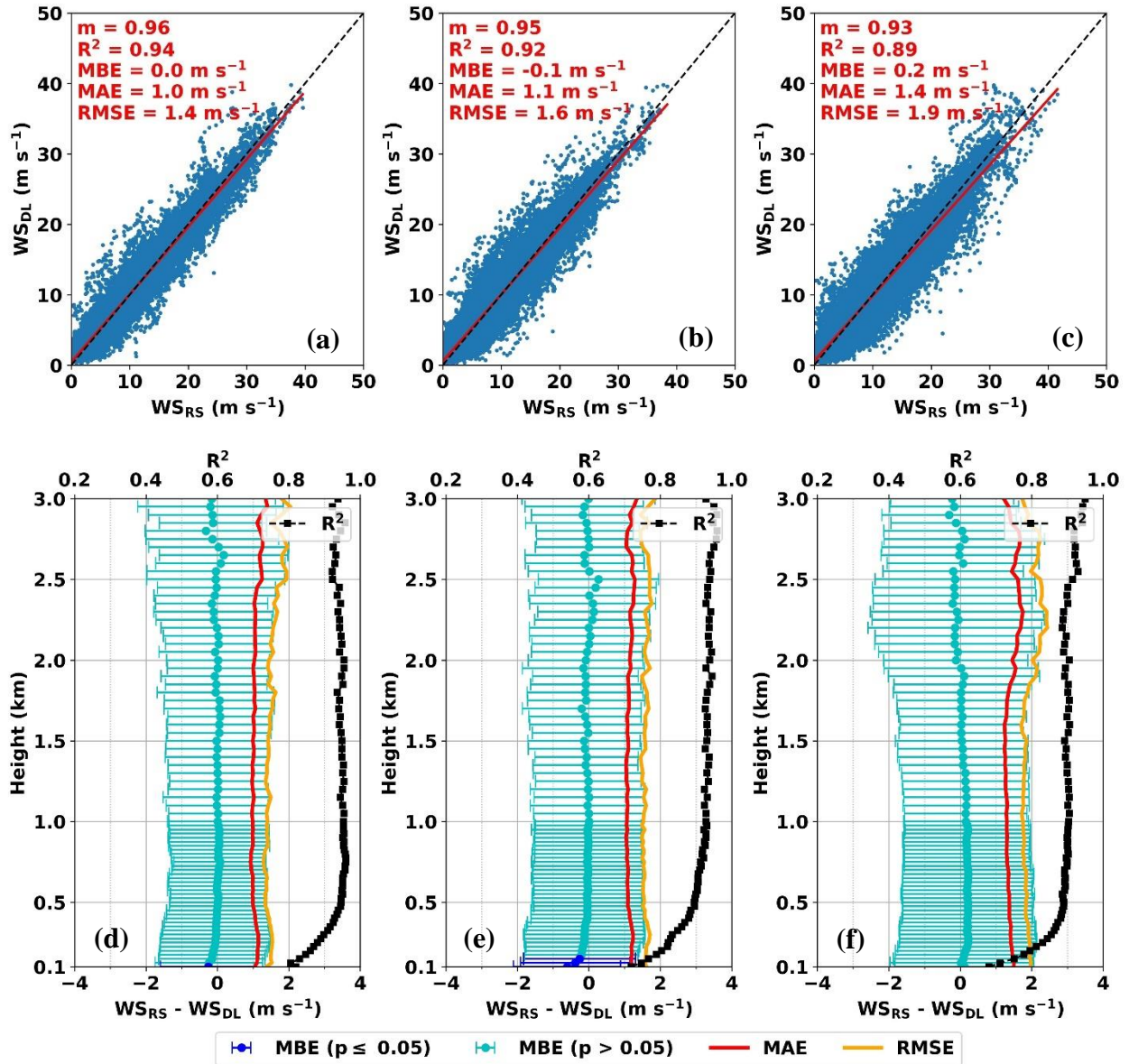
Figure 3. Scatterplots for RS and DL measured horizontal wind speed (WS) at three NYSM Profiler Network sites at: (a) Buffalo, (b) Albany, and (c) Stony Brook. Vertical profiles of R^2 , MBE with one standard deviation error bars, MAE and RMSE for the same variable at the respective sites: (d) Buffalo, (e) Albany, and (f) Stony Brook.
