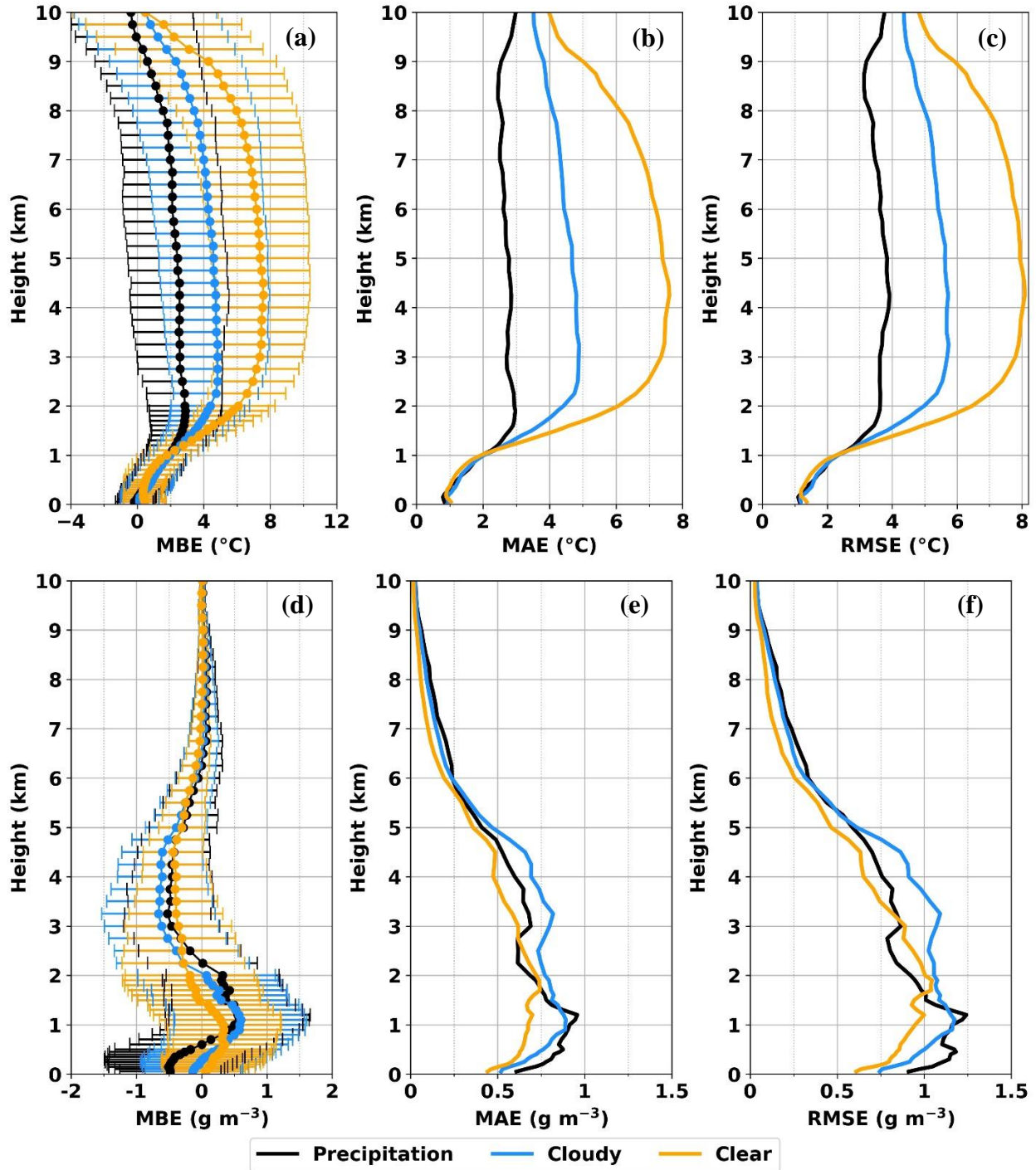
480 Figure 10. Vertical profiles of MBE with one standard deviation error bars, MAE and RMSE for (a – c) temperature and (d – f) water vapor density during three weather conditions from the NYSM Profiler site at Albany.
