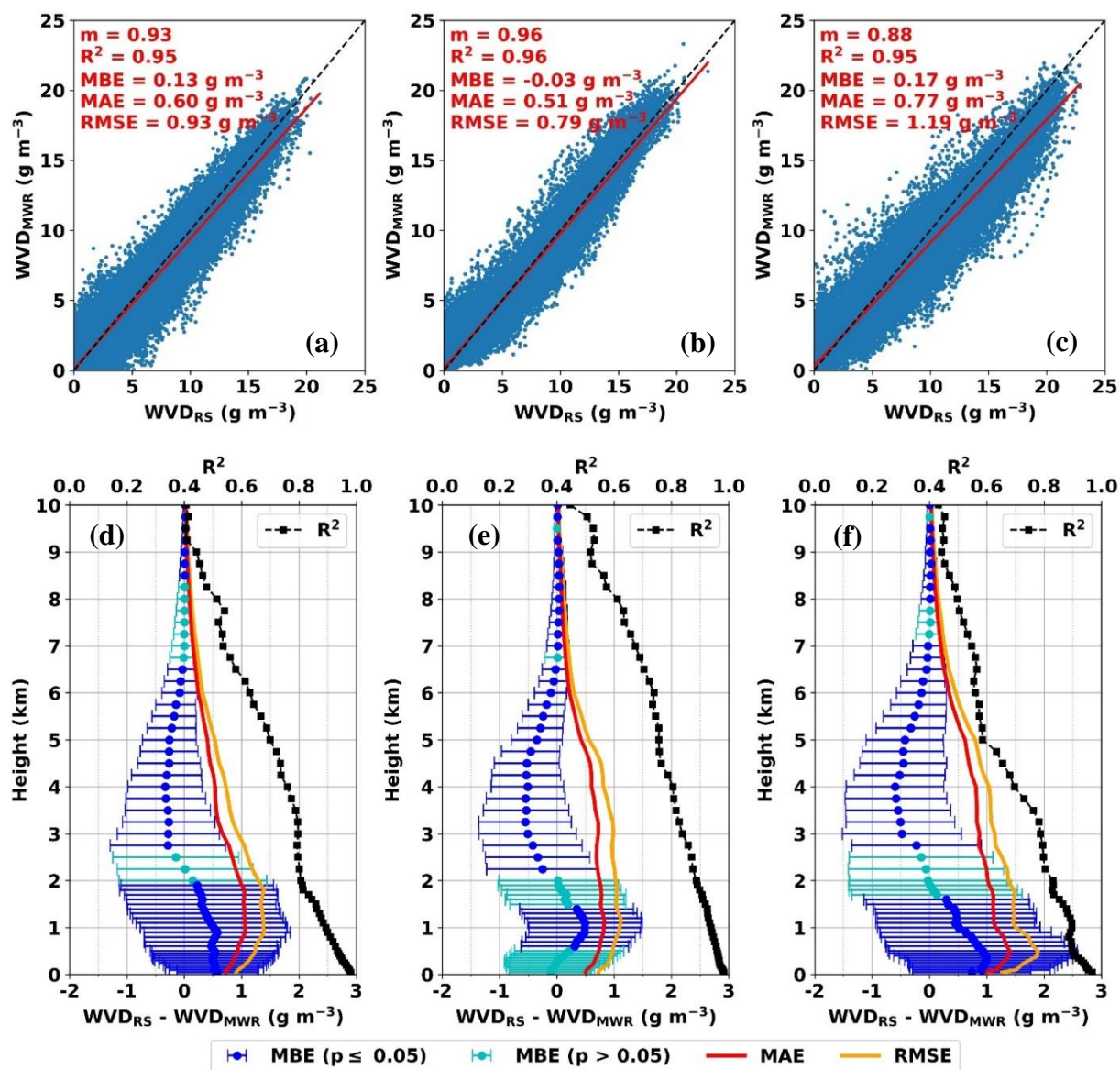
395 Figure 8. Scatterplots for RS and MWR measured water vapor density (WVD) at three NYSM Profiler Network sites at: (a) Buffalo, (b) Albany, and (c) Stony Brook. Vertical profiles of R^2 , MBE with one standard deviation error bars, MAE and RMSE for the same variable at the respective sites: (d) Buffalo, (e) Albany, and (f) Stony Brook.
