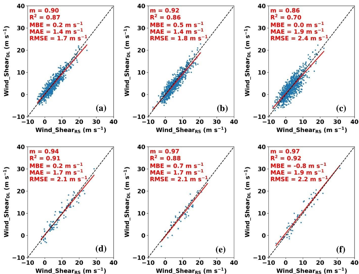
330 Figure 5. Scatterplots for RS and DL derived 100 m – 1 km wind shear at three NYSM Profiler Network sites at: (a) Buffalo, (b) Albany, and (c) Stony Brook and 100 m – 3 km wind shear at the respective sites: (d) Buffalo, (e) Albany and (f) Stony Brook.
