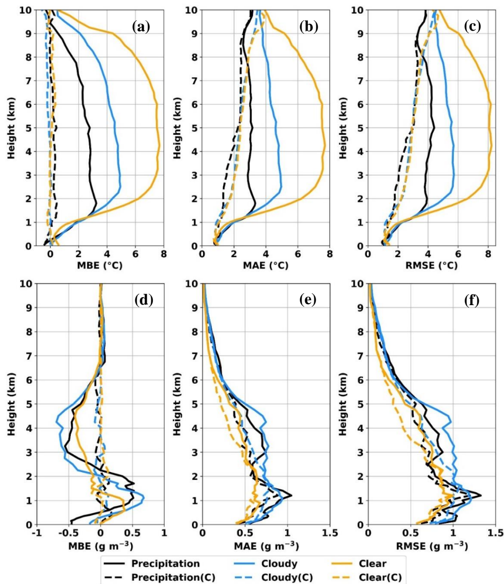
525 Figure 11. Vertical profiles of MBE, MAE and RMSE for original and corrected (C) MWR measured (a – c) temperature and (d – f) water vapor density during three weather conditions from the NYSM Profiler site at Albany.
