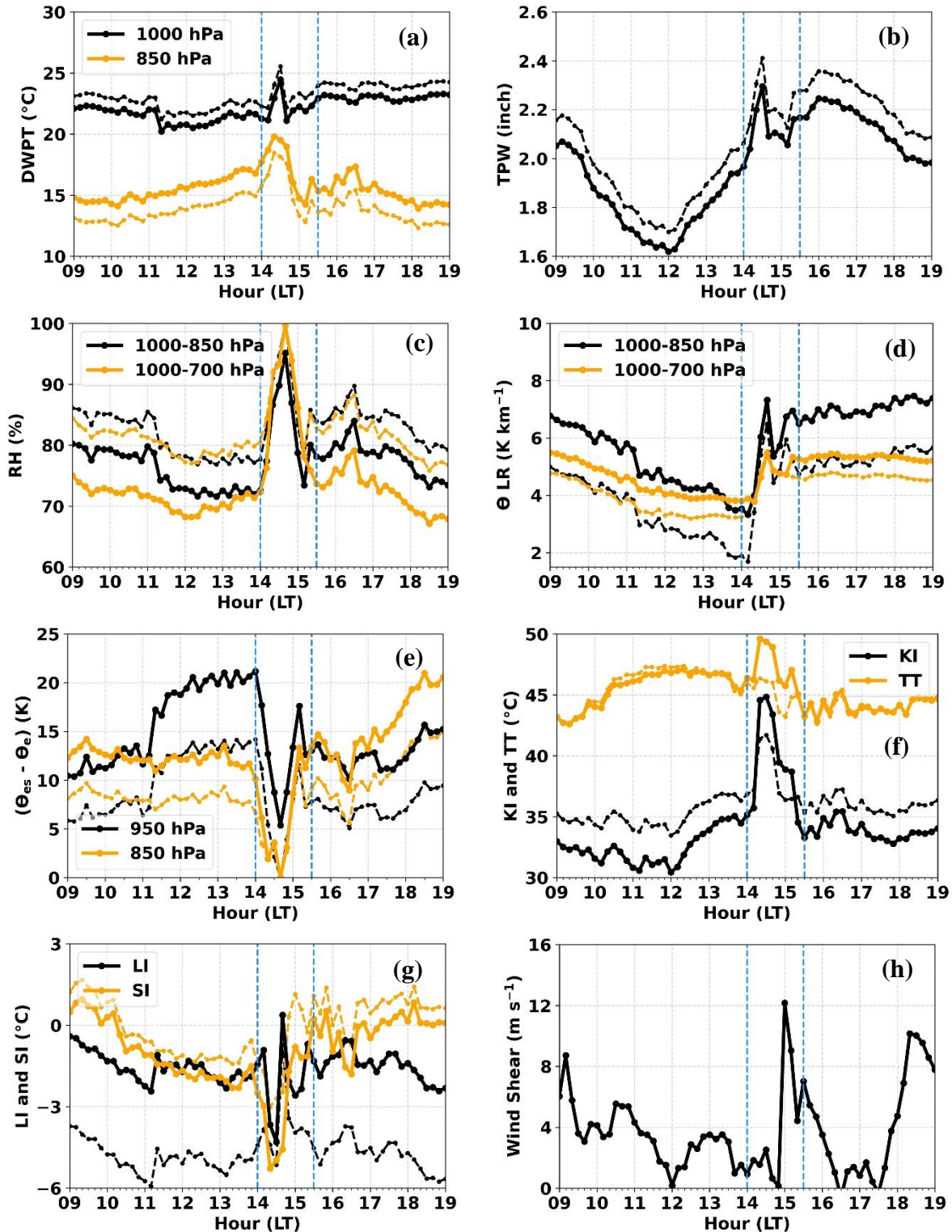
Figure 13. Original (light color) and corrected (bold color) MWR derived (a) DWPT, (b) TPW, (c) Mean RH (d) \theta LR (e) ( \theta_{es} - \theta_e ), (f) KI and TT, (g) LI and SI, and DL derived (h) Wind Shear (100 m – 1 km) at Albany on 12 August 2021. Dotted box represents thunderstorm episode.
