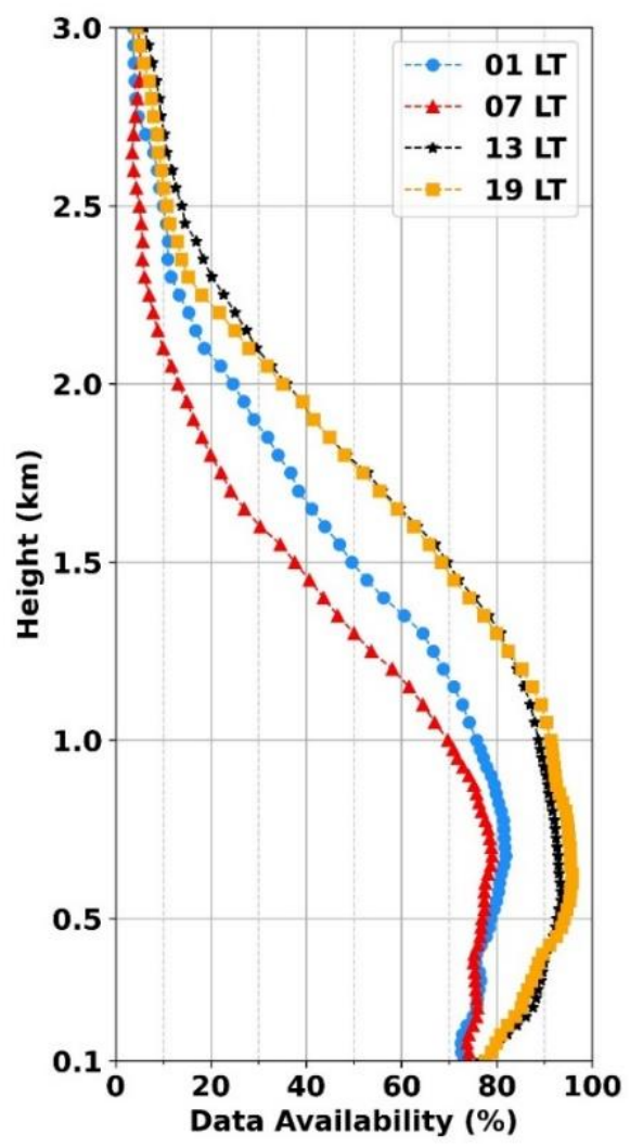
190 Figure 2. The DL data availability during four different hours at NYSM Profiler site at Albany during May – August 2021. The NWS RS launches are at 12 UTC (7 LT) and at 00 UTC (19 LT).
