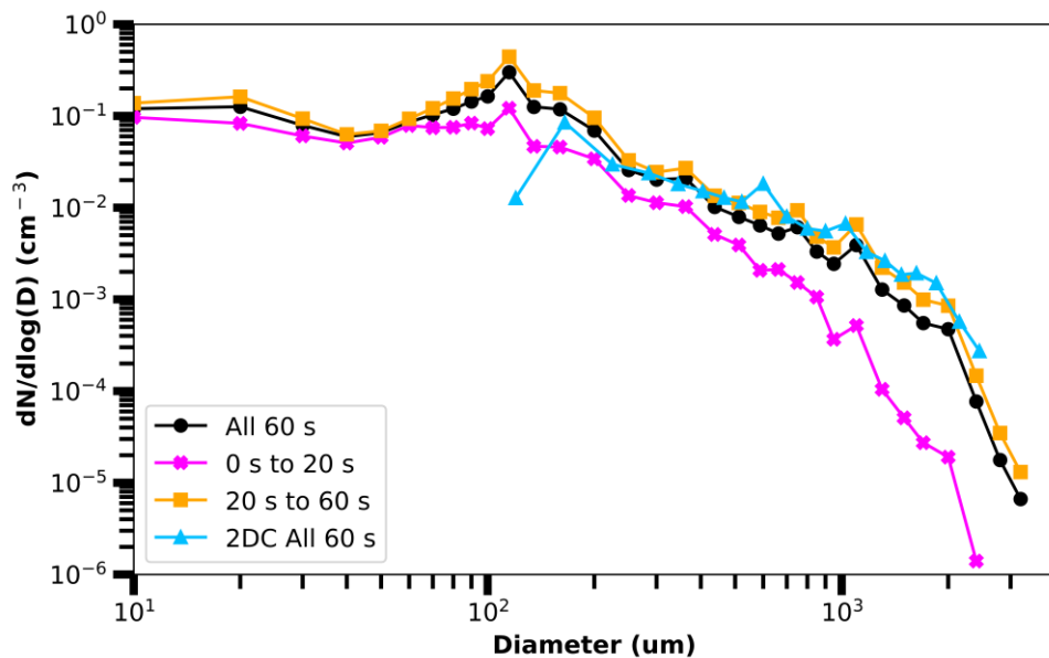
Figure 11: The size spectrum normalized by bin width measured by the external cloud probes (ECP) for the -33 °C case (Table 2). The spectrum of the entire 60 s case (round, black) has been separated according to times of more (cross, magenta) and less (square, orange) agreement between ECP and Optical Ice Detector (OID) backscatter coefficients. Also given is the 2D-C spectrum (triangle, blue) obtained using the fast-circle and full particle reconstruction processing methods. The 2D-S and HVPS3 diameters for the ECP combine spectrum are obtained using image data processed with the area-equivalent diameter-mm method.
