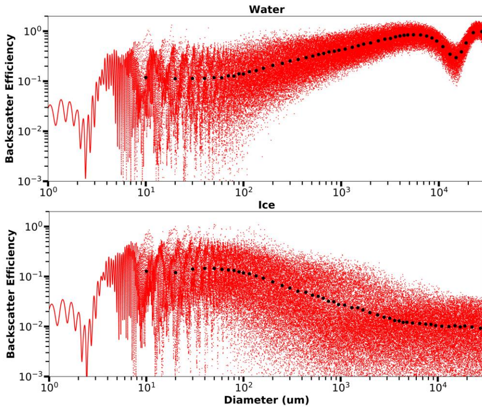
Figure 3: Plots showing backscatter efficiencies using Mie theory for spherical water (top) and ice (bottom) particles. The MiePlot software package (Laven 20182020) is used to calculate efficiencies for 100 000 particle diameters distributed log-normally between 1 \mu\text{m} and 30 mm (red dots). Intervals between diameters used for the individual backscatter efficiency calculations range from 0.0001 \mu\text{m} at the lowest diameters, to 3 \mu\text{m} at the highest diameters. Intervals range from 0.0001 \mu\text{m} for the smallest diameters and 3 \mu\text{m} for the largest diameters. Black circles are average efficiencies over the combined spectrum channel widths (see Table 1 for numerical values). A refractive index of 1.3263 + 5.6 \times 10^{-7}i is used for water (Kedenburg et al. 2012) and 1.3031 + 5.6 \times 10^{-7}i for ice (Warren and Brandt 2008). Scattering is for an air medium at 20 ^{\circ}\text{C} and incident light of 905 nm.
