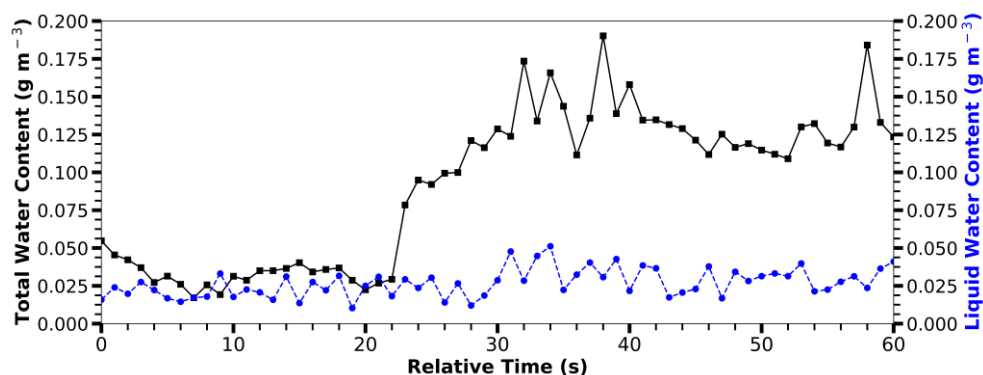
Figure 12: Nevzorov probe measured total water content (TWC) (solid, square black) and liquid water content (LWC) (dashed, round blue) for the -33\text{ }^{\circ}\text{C} case (Table 2). Each point represents 1 s of Nevzorov data. The average LWC is 0.022\text{ g m}^{-3} \pm 0.009\text{ g m}^{-3} and the average TWC is 0.032\text{ g m}^{-3} \pm 0.008\text{ g m}^{-3} during times of Optical Ice Detector (OID) and external cloud probe (ECP) backscatter coefficient agreement (0 s to 20 s). The average LWC is 0.027\text{ g m}^{-3} \pm 0.009\text{ g m}^{-3} and the average TWC is 0.092\text{ g m}^{-3} \pm 0.05\text{ g m}^{-3} during times of OID and ECP backscatter coefficient disagreement (30 s to 60 s).
