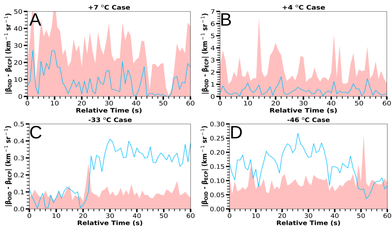
340 Figure 6: Plots showing 1 Hz time series of the absolute difference (blue line) between the Optical Ice Detector (OID) and external cloud probes (ECP) backscatter coefficients for the four case study segments (Table 2). The shadowed region top represents 3 standard deviations of OID and ECP backscatter coefficients, determined using Eq. (7).
