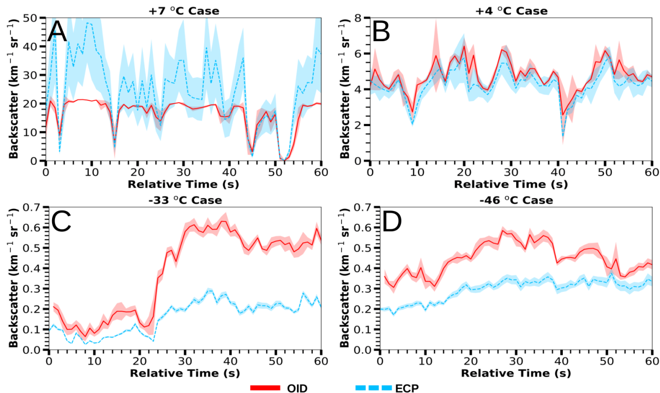
Figure 5: Plots showing 1 Hz time series in seconds of backscatter coefficients with a shadowed range for the four case study segments (Table 2). Note the differing backscatter coefficient scales for the warm cloud cases. The external cloud probes (ECP) shadowed range is the measurement uncertainty determined from Eq. (5) and represents 1 standard deviation. The Optical Ice Detector (OID) shadowed range is 1 Hz data representing 1 standard deviation computed of the 5 Hz measurements. The ECP backscatter coefficient is obtained from particle data processed with the area method.
