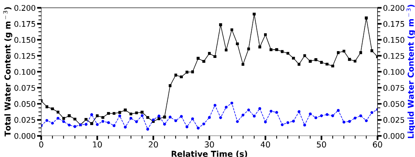
485 Figure 12: Nevzorov probe measured total water content (TWC) (solid, square black) and liquid water content (LWC) (dashed, round blue) for the -33\text{ }^{\circ}\text{C} case (Table 2). Each point represents 1 s of Nevzorov data. The average LWC is 0.022\text{ g m}^{-3} \pm 0.009\text{ g m}^{-3} and the average TWC is 0.032\text{ g m}^{-3} \pm 0.008\text{ g m}^{-3} during times of Optical Ice Detector (OID) and external cloud probe (ECP) backscatter coefficient agreement (0 s to 20 s). The average LWC is 0.027\text{ g m}^{-3} \pm 0.009\text{ g m}^{-3} and the average TWC is 0.092\text{ g m}^{-3} \pm 0.05\text{ g m}^{-3} during times of OID and ECP backscatter coefficient disagreement (30 s to 60 s).
