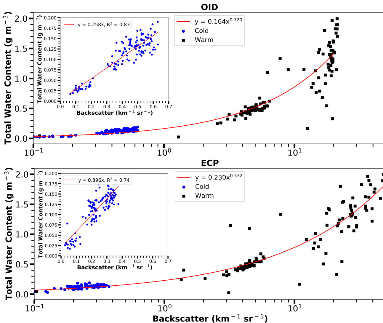
400 Figure 9: Plots showing Nevzorov probe total water content (TWC) versus Optical Ice Detector (OID) backscatter coefficients (top) and external cloud probes (ECP) backscatter coefficients (bottom) with a logarithmic x-axis. Backscatter coefficients are separated by warm (+7 °C and +4 °C) cases (square, black) and cold (-33 °C and -46 °C) cases (round, blue) (Table 2). Insets in the top-left corners show further detail of Nevzorov probe TWC versus respective backscatter coefficients for the -33 °C and -46 °C cases. Each point represents 1 s of Nevzorov, OID, and ECP data. The ECP backscatter coefficient is obtained using image data processed with the area-equivalent diameter method for all cases.
