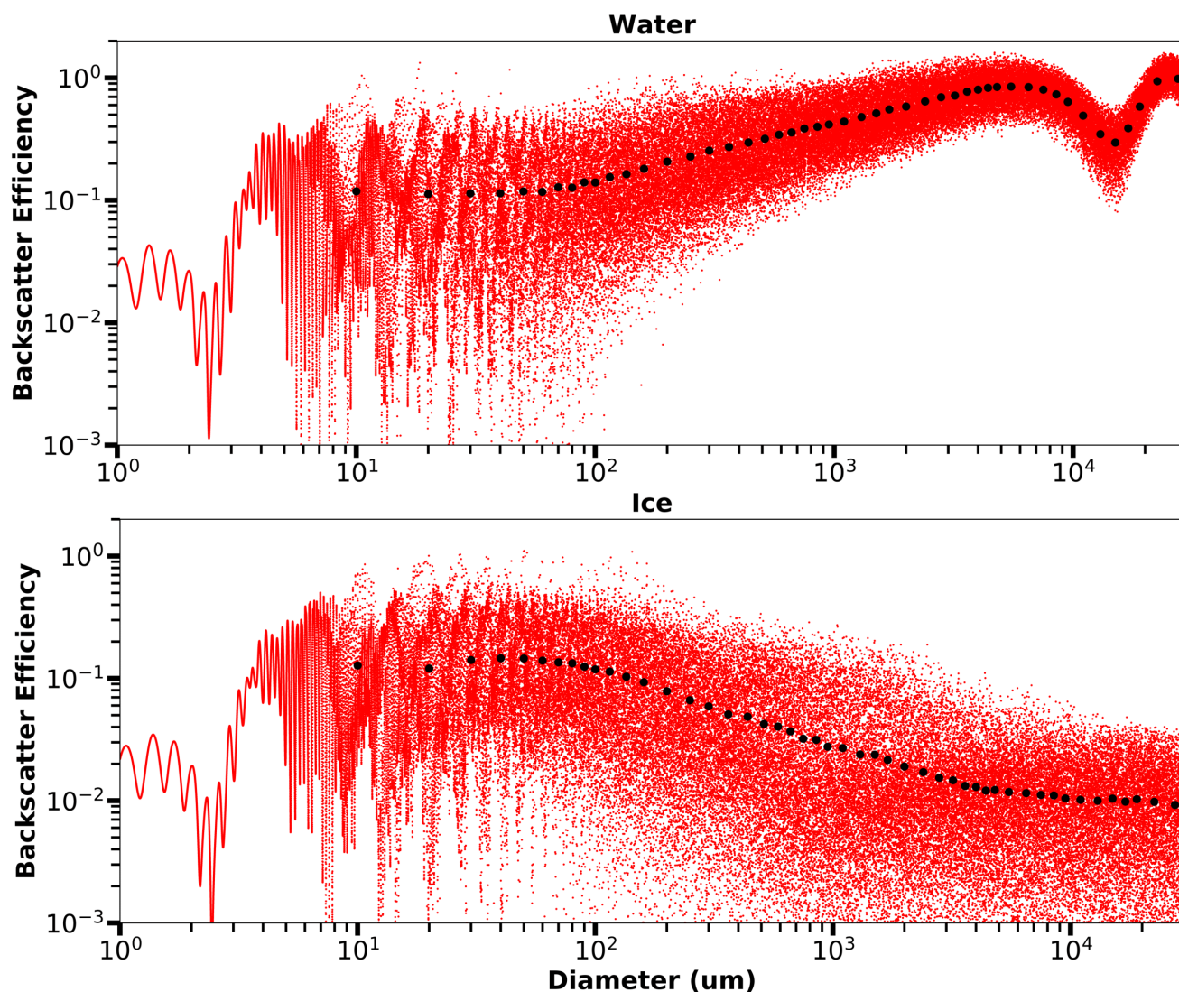
270 Figure 3: Plots showing backscatter efficiencies using Mie theory for spherical water (top) and ice (bottom) particles. The MiePlot software package (Laven 2018) is used to calculate efficiencies for 100 000 particle diameters distributed log-normally between 1 µm and 30 mm (red dots). Intervals range from 0.0001 µm for the smallest diameters and 3 µm for the largest diameters. Black circles are average efficiencies over the combined spectrum channel widths (see Table 1Error! Reference source not found. for numerical values). A refractive index of 1.3263 + 5.6 \times 10^{-7}j is used for water (Kedenburg et al. 2012) and 1.3031 + 5.6 \times 10^{-7}j for ice 275 (Warren and Brandt 2008). Scattering is for an air medium at 20 °C and incident light of 905 nm.
