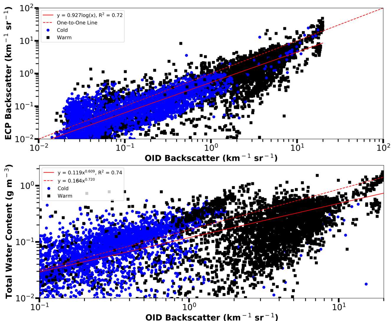
405 Figure 10: The external cloud probes (ECP) backscatter coefficients versus Optical Ice Detector (OID) backscatter coefficients (top) and Nevzorov probe total water contents (TWC) versus OID backscatter coefficients (bottom) for all times within the four flights (Table 2) that contain the four temperature cases. The 1 Hz data is grouped by cold (round, blue) and warm (square, black) environments. Data are excluded when temperatures are between 0^\circ\text{C} and -20^\circ\text{C} . Liquid scattering efficiencies are used for 410 temperatures greater than 0^\circ\text{C} and ice scattering efficiencies used for temperatures below -20^\circ\text{C} . OID data has a 20 \text{ km}^{-1} \text{sr}^{-1} limit to avoid times where observations are above the OID's detection limit. The lower plot's red dashed line indicates the fit equation in Fig. 9. The ECP backscatter coefficient is obtained using image data processed with the area-equivalent diameter method for all cases.
